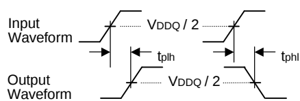
Fig.2 Tdly measurement
