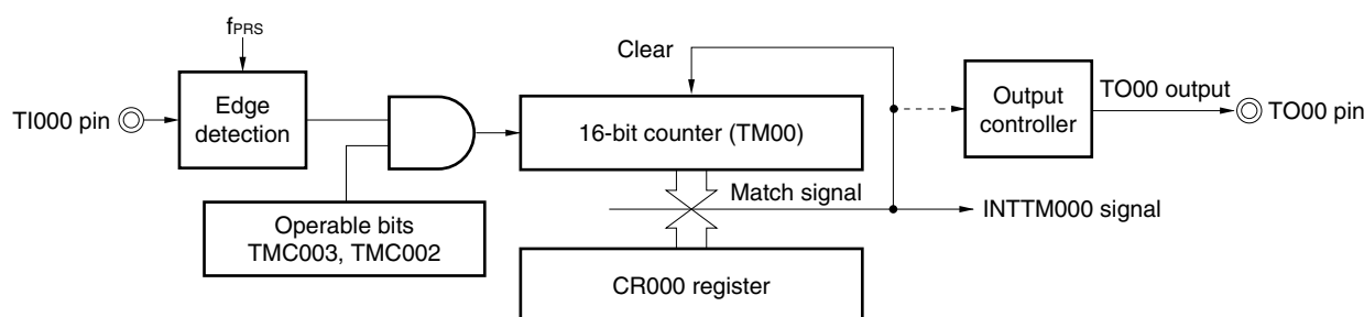
Figure 6-19. Block Diagram of External Event Counter Operation
