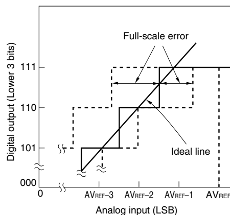
Figure 11-17. Full-Scale Error
