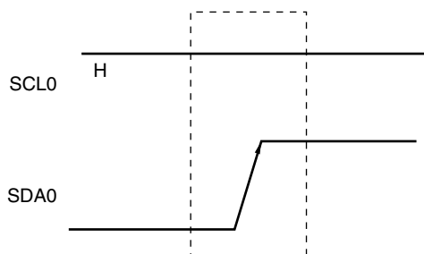
Figure 15-17. Stop Condition
