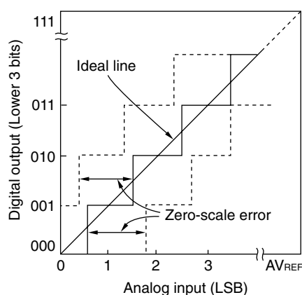
Figure 11-16. Zero-Scale Error
