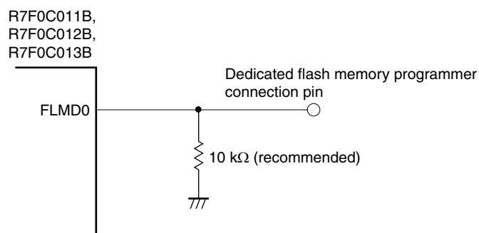
Figure 22-5. FLMD0 Pin Connection Example
