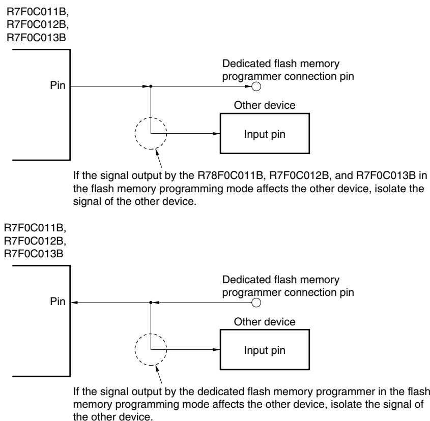
Figure 22-7. Malfunction of Other Device
