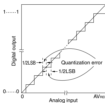
Figure 11-15. Quantization Error
