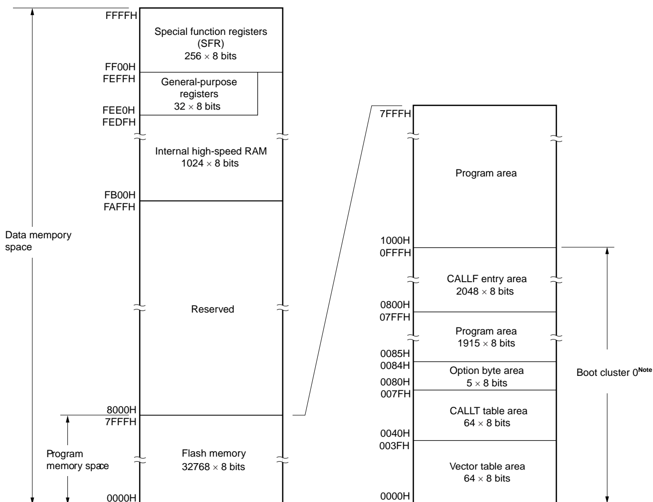
Figure 3-3. Memory Map (R7F0C013B)
