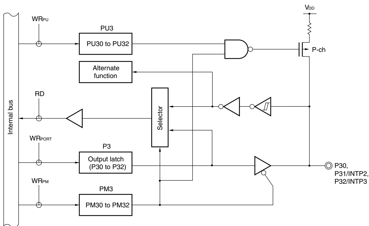
Figure 4-9. Block Diagram of P30 to P32
