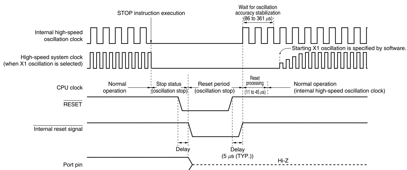
Figure 18-4. Timing of Reset in STOP Mode by RESET Input
