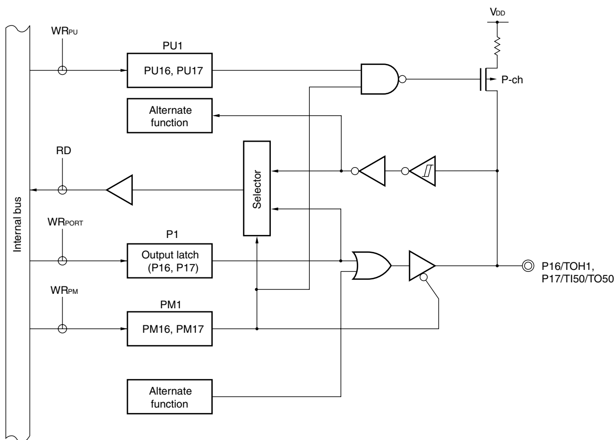
Figure 4-7. Block Diagram of P16 and P17
