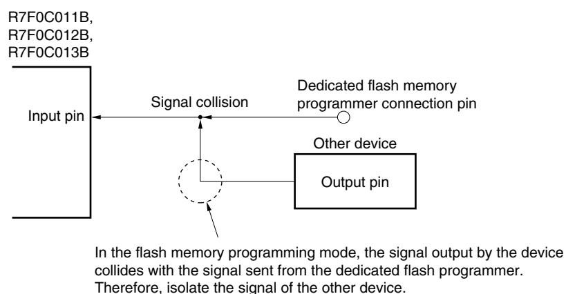
Figure 22-6. Signal Collision (Input Pin of Serial Interface)
