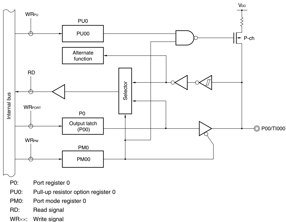
Figure 4-1. Block Diagram of P00
