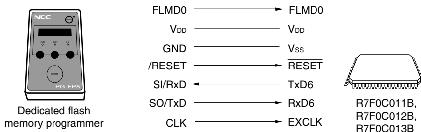
Figure 22-4. Communication with Dedicated Flash memory programmer (UART6)
