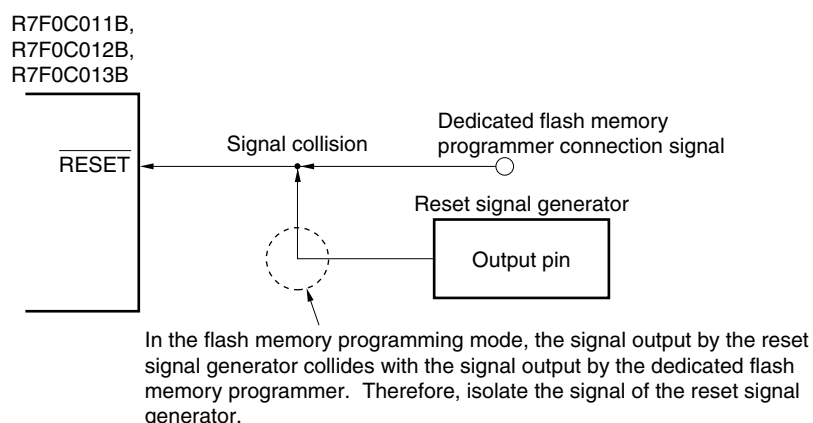
Figure 22-8. Signal Collision ( \overline{\text{RESET}} Pin)
