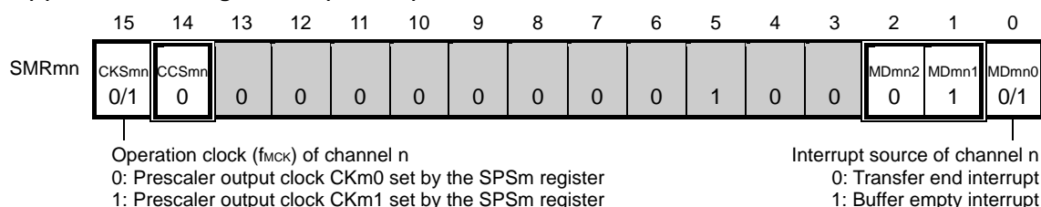
Figure 12-76. Example of Contents of Registers for UART Transmission of UART (UART0 to UART3) (1/2)
