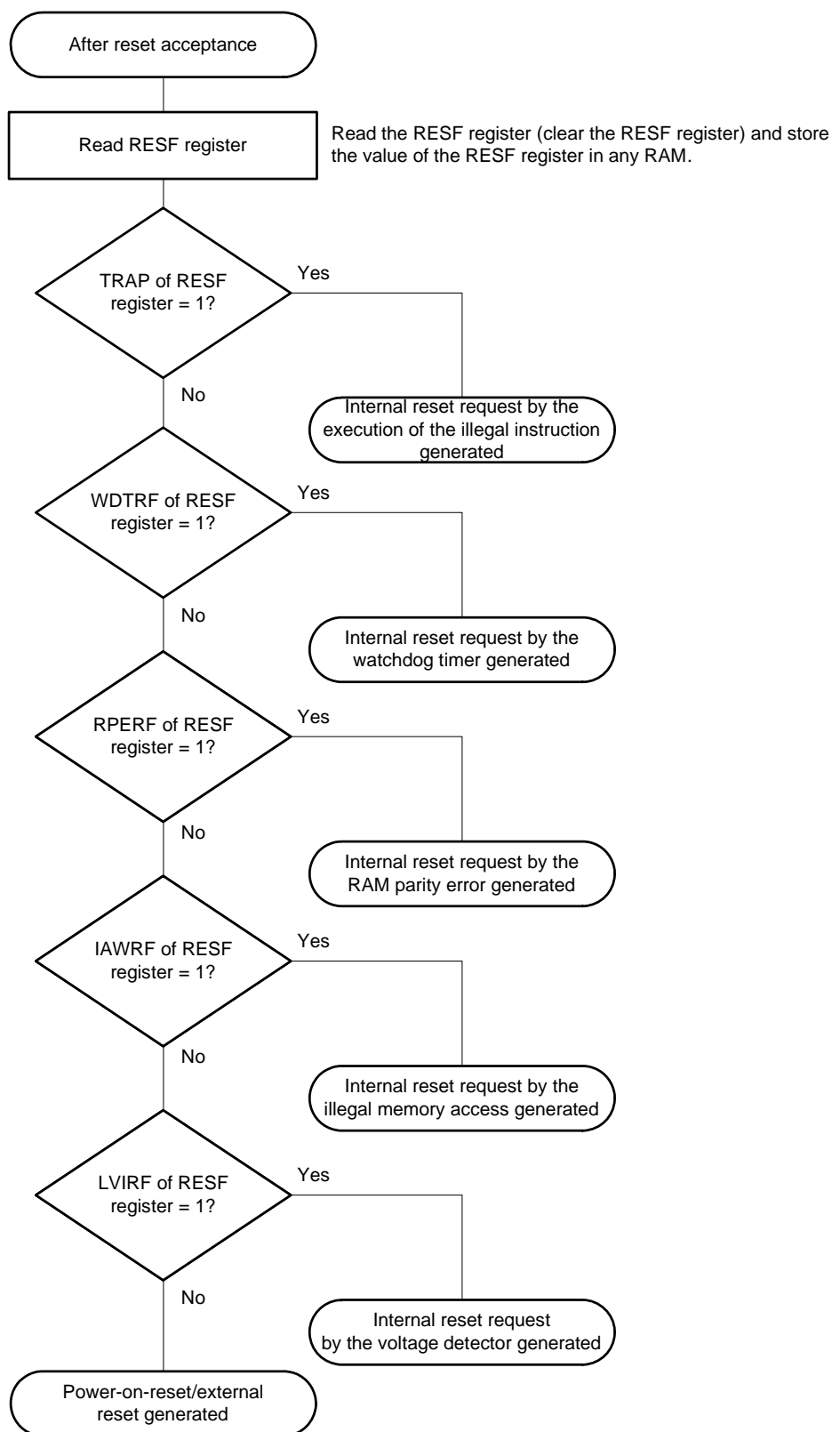
Figure 19-5. Example of Procedure for Checking Reset Source
