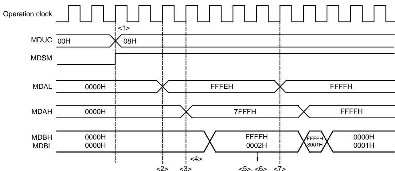
Figure 14-7. Timing Diagram of Multiplication (Signed) Operation ( -2 \times 32767 = -65534 )
