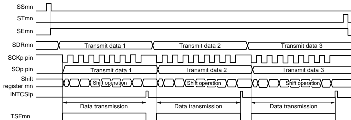
Figure 12-29. Timing Chart of Master Transmission (in Single-Transmission Mode) (Type 1: DAPmn = 0, CKPmn = 0)
