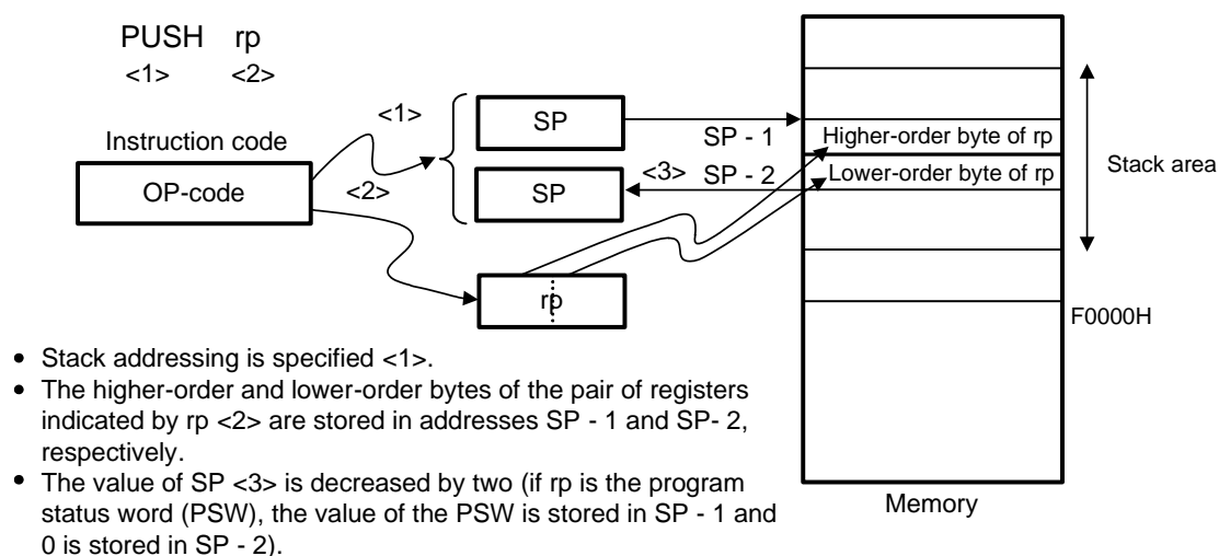
Figure 3-41. Example of PUSH rp
