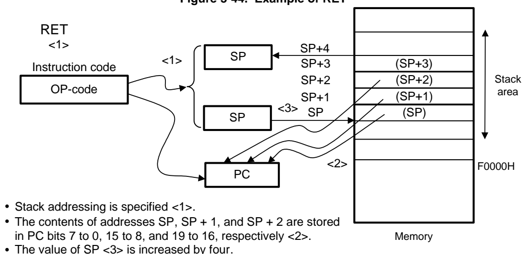
Figure 3-44. Example of RET
