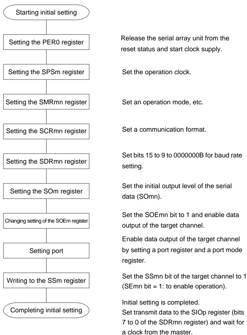
Figure 12-64. Initial Setting Procedure for Slave Transmission/Reception
