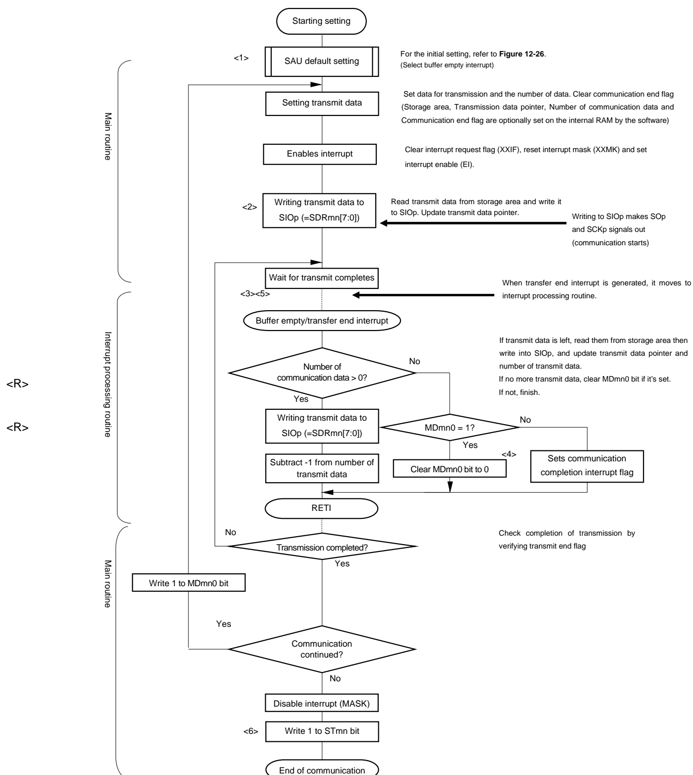
Figure 12-32. Flowchart of Master Transmission (in Continuous Transmission Mode)
