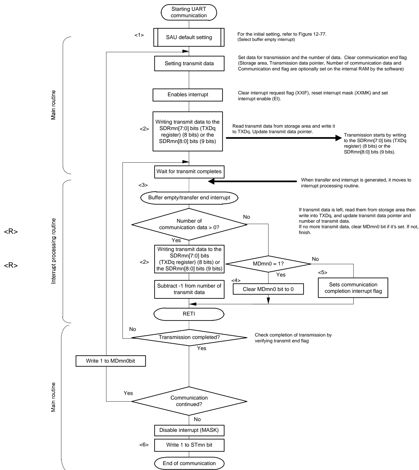
Figure 12-83. Flowchart of UART Transmission (in Continuous Transmission Mode)
