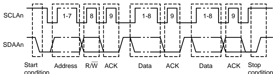
Figure 13-14. I 2 C Bus Serial Data Transfer Timing
