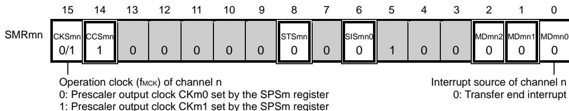
Figure 12-57. Example of Contents of Registers for Slave Reception of 3-Wire Serial I/O (CSI00, CSI01, CSI10, CSI11, CSI20, CSI21, CSI30, CSI31) (1/2)
