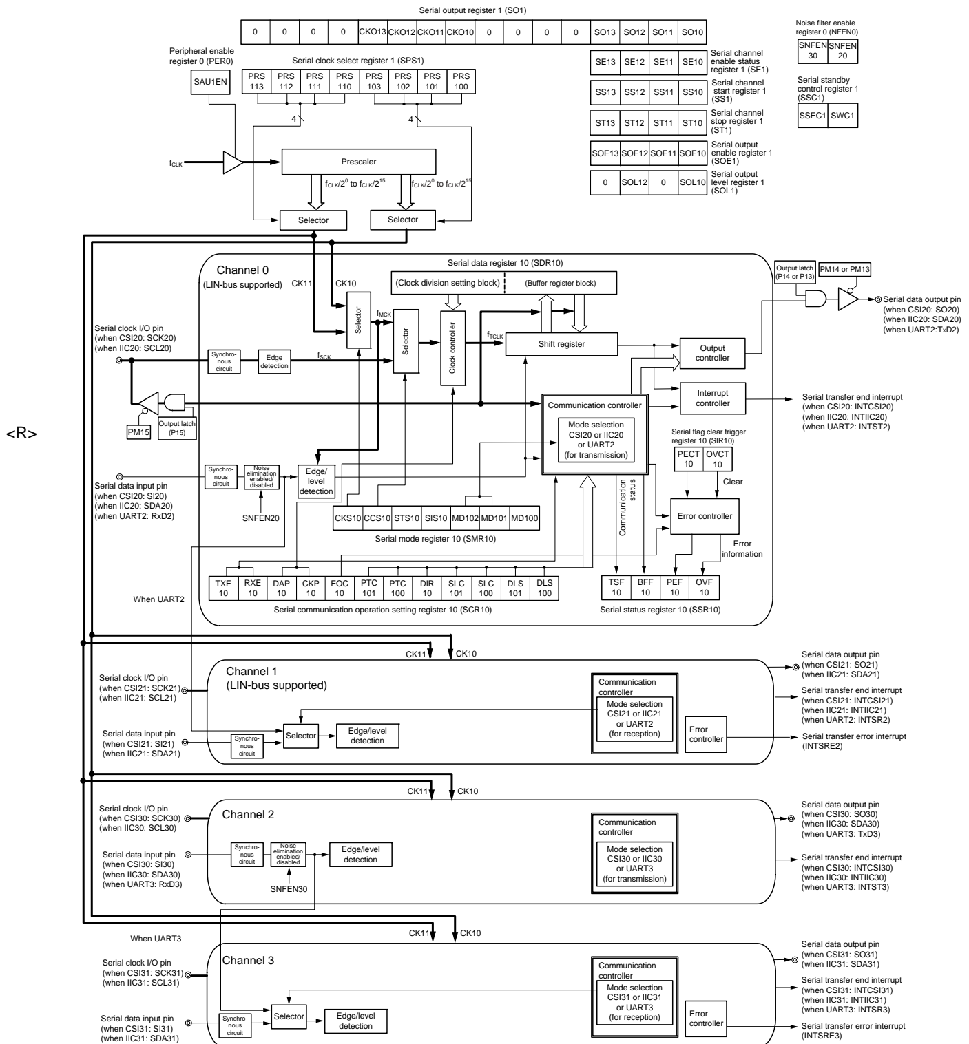
Figure 12-2. Block Diagram of Serial Array Unit 1
