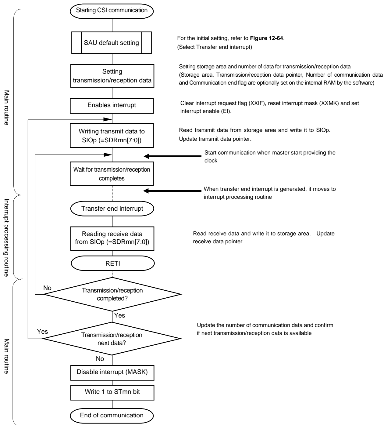
Figure 12-68. Flowchart of Slave Transmission/Reception (in Single-Transmission/Reception Mode)
