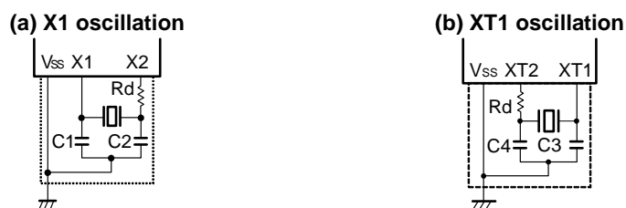
Figure 5-16. External Oscillation Circuit Example
