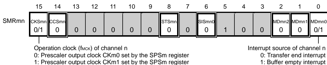
Figure 12-41. Example of Contents of Registers for Master Transmission/Reception of 3-Wire Serial I/O (CSI00, CSI01, CSI10, CSI11, CSI20, CSI21, CSI30, CSI31) (1/2)
