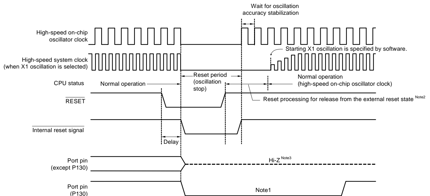
Figure 19-2. Timing of Reset by \overline{\text{RESET}} Input
