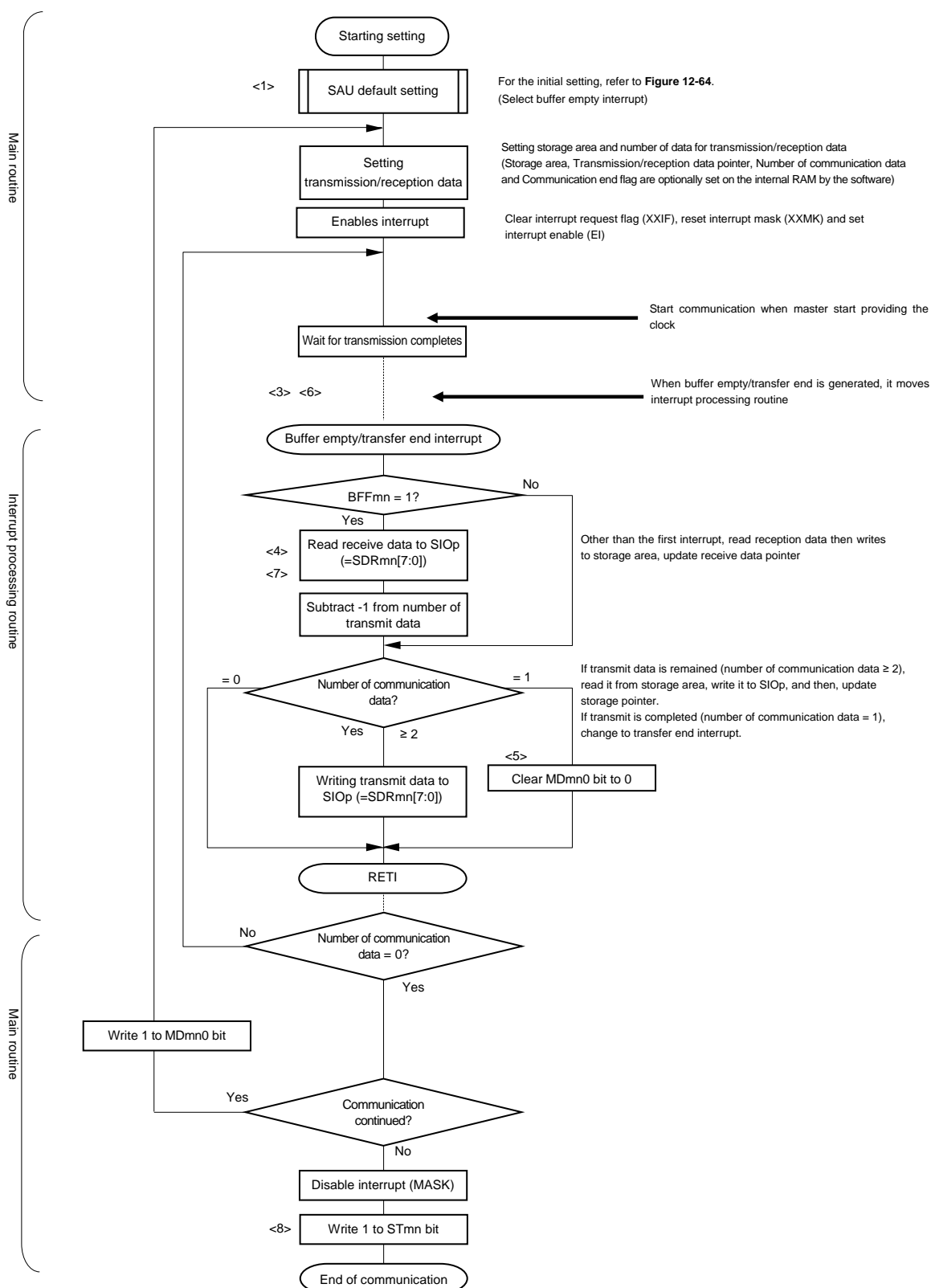
Figure 12-70. Flowchart of Slave Transmission/Reception (in Continuous Transmission/Reception Mode)
