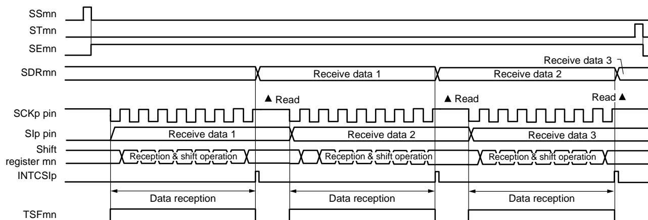
Figure 12-61. Timing Chart of Slave Reception (in Single-Reception Mode)
