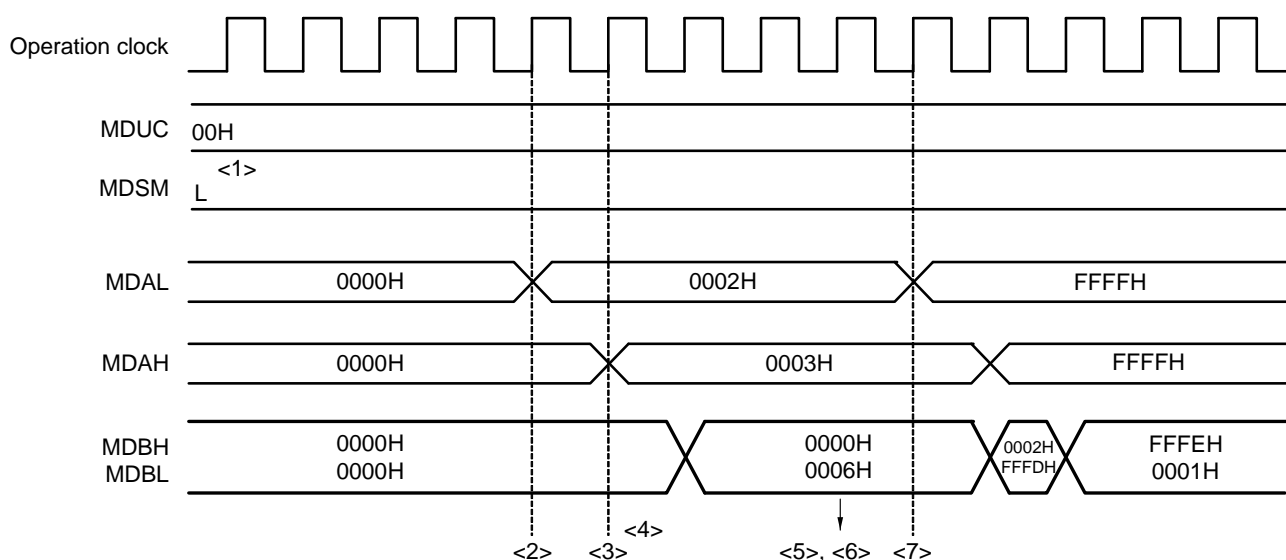
Figure 14-6. Timing Diagram of Multiplication (Unsigned) Operation ( 2 \times 3 = 6 )
