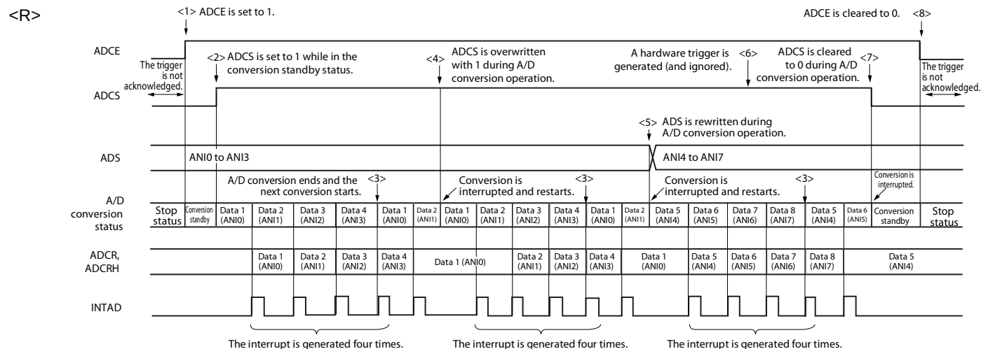
Figure 11-20. Example of Software Trigger Mode (Scan Mode, Sequential Conversion Mode) Operation Timing
