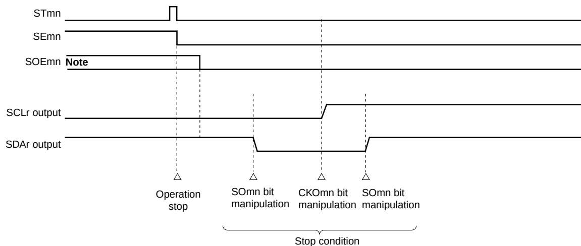
Figure 12-134. Timing Chart of Stop Condition Generation
