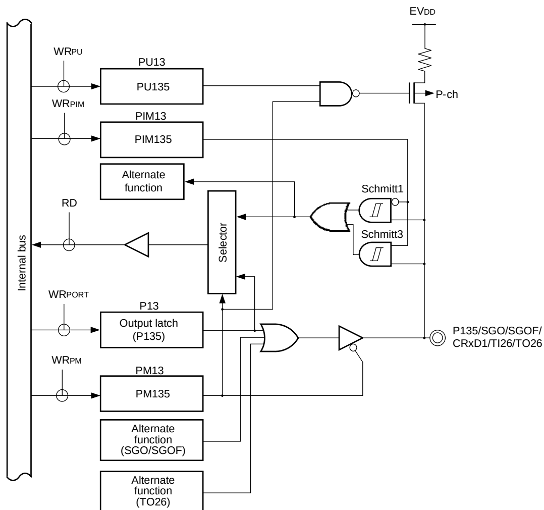
Figure 4-46. Block Diagram of P135
