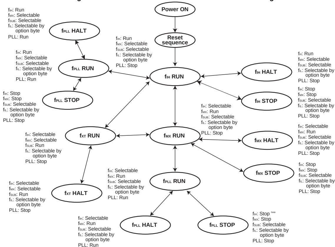
Figure 5-20. CPU Clock Status Transition us Transition Diagram
