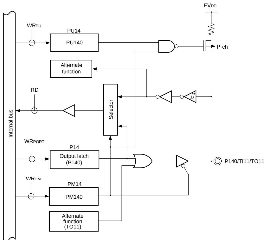
Figure 4-49. Block Diagram of P140
