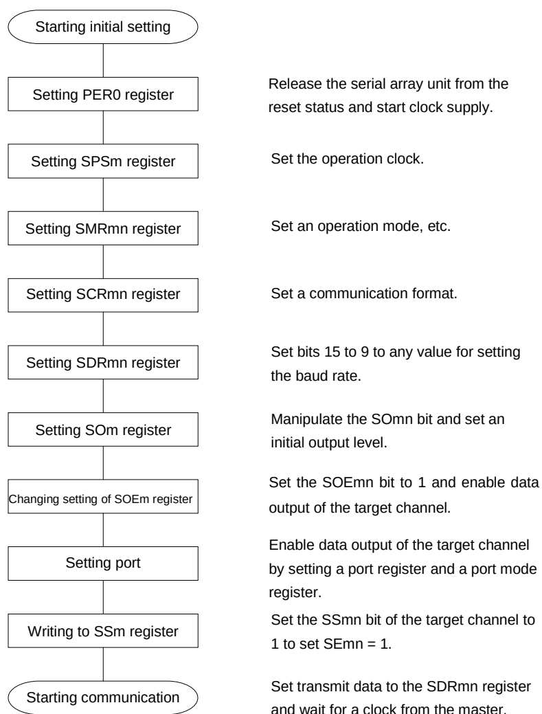
Figure 12-53. Initial Setting Procedure for Slave Transmission
