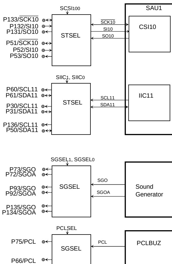
Figure 4-60. Serial unit, SG, and PCL connection (2/2)
