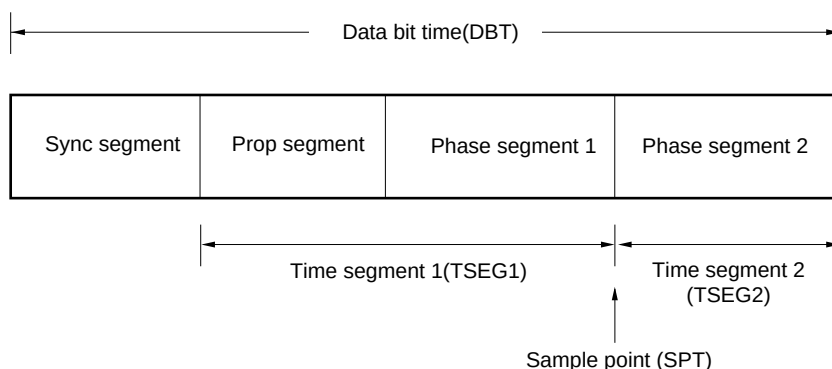
Figure 14-18. Segment Setting
