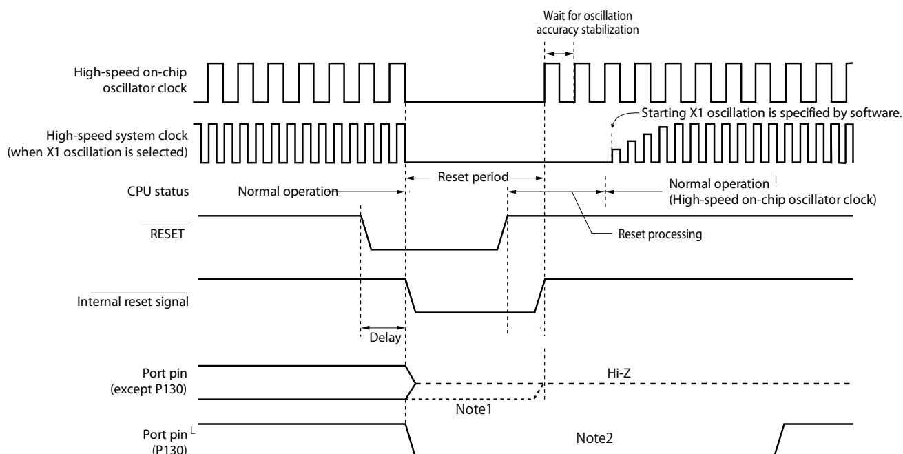
Figure 22-2. Timing of Reset by \overline{\text{RESET}} Input
