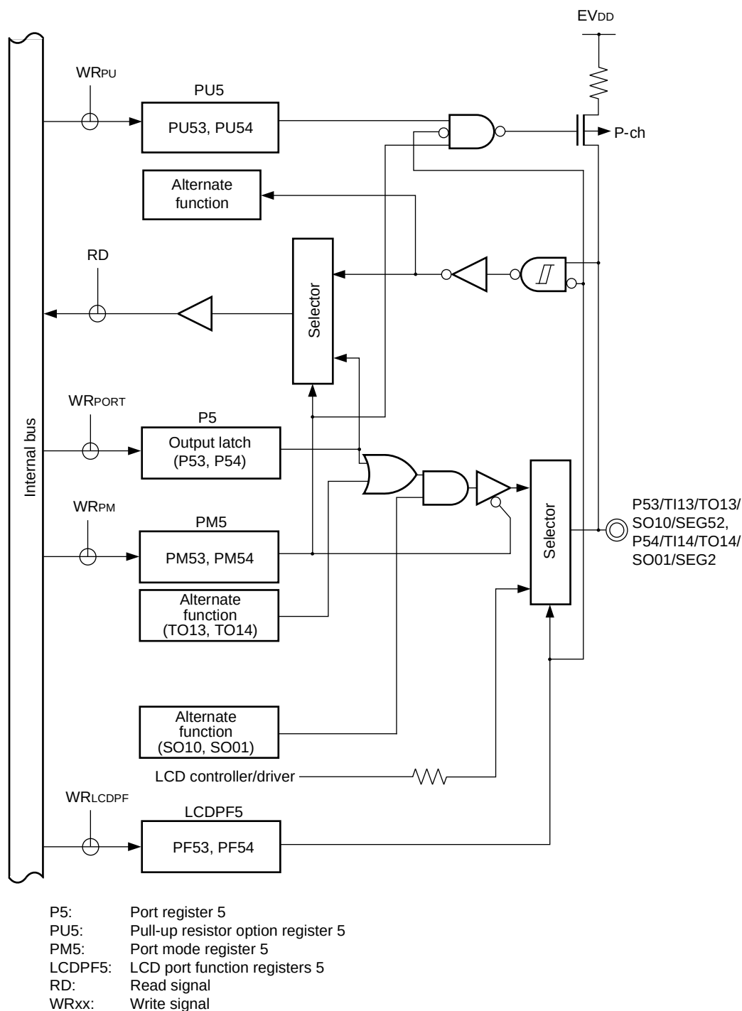
Figure 4-21. Block Diagram of P53, P54
