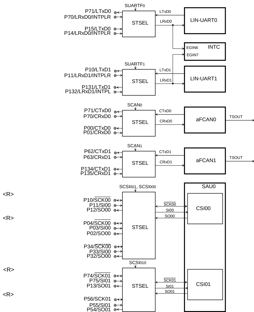
Figure 4-60. Serial unit, SG, and PCL connection (1/2)
