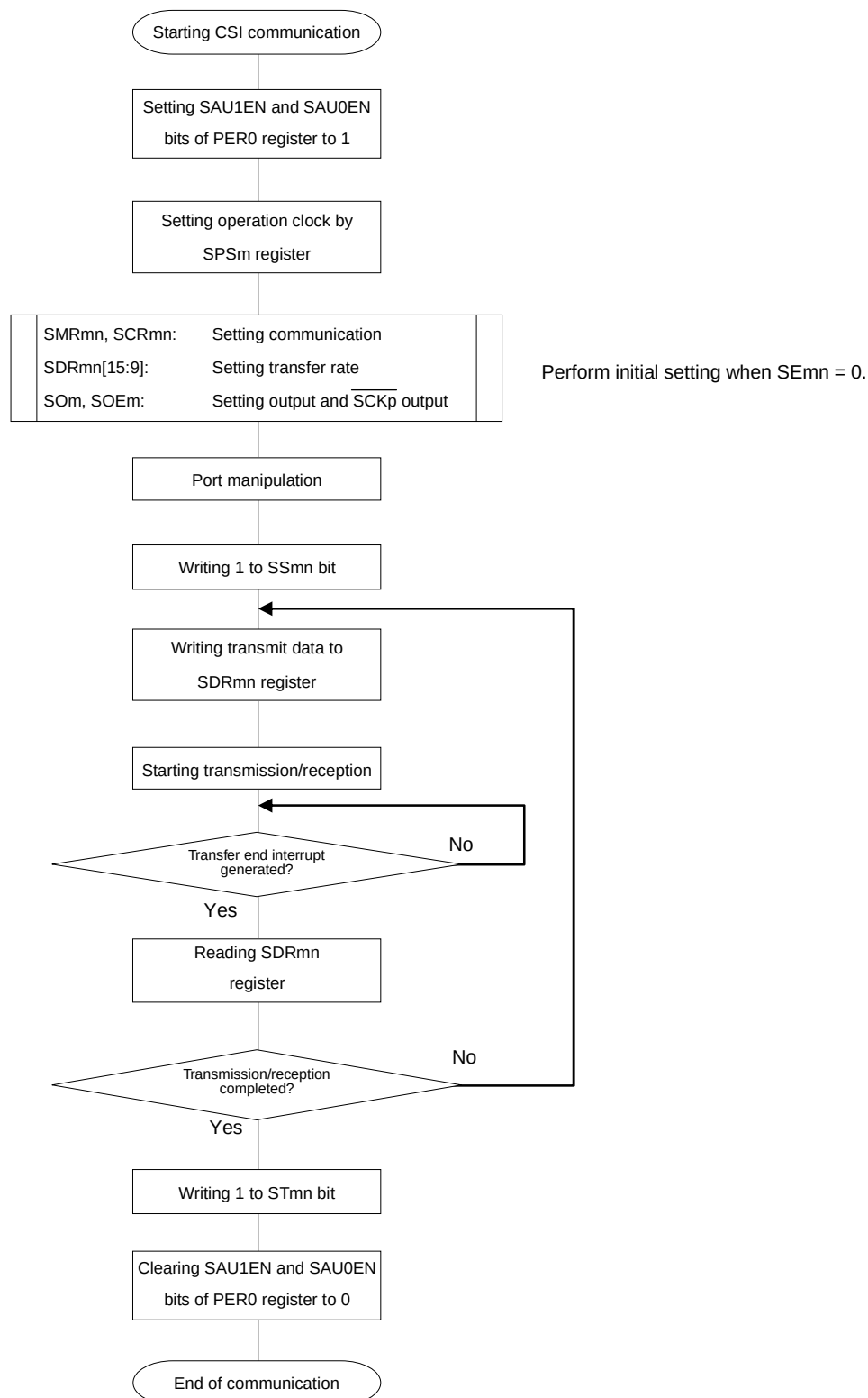
Figure 12-49. Flowchart of Master Transmission/Reception (in Single- Transmission/Reception Mode)
