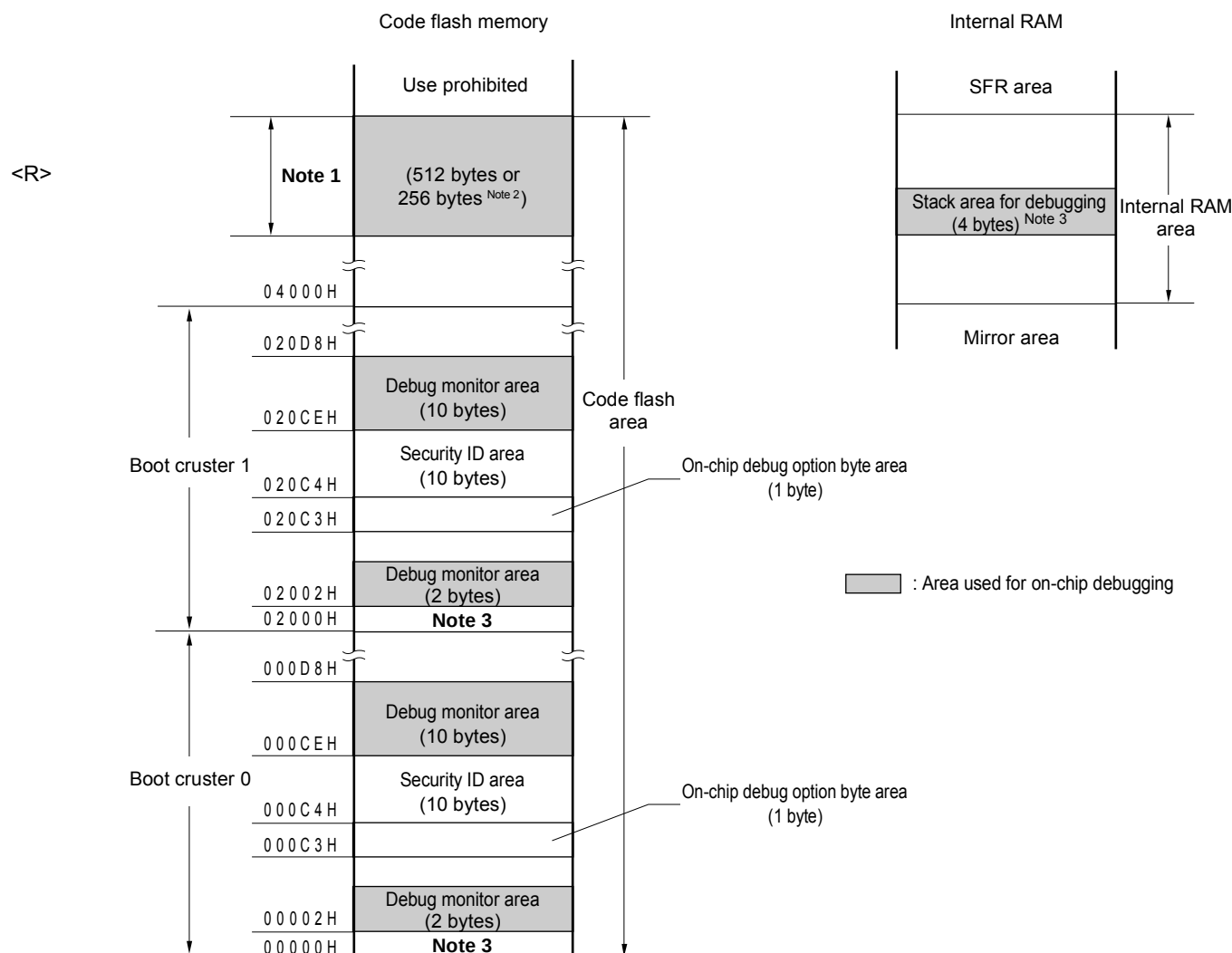
Figure 29-2. Memory Spaces Where Debug Monitor Programs Are Allocated
