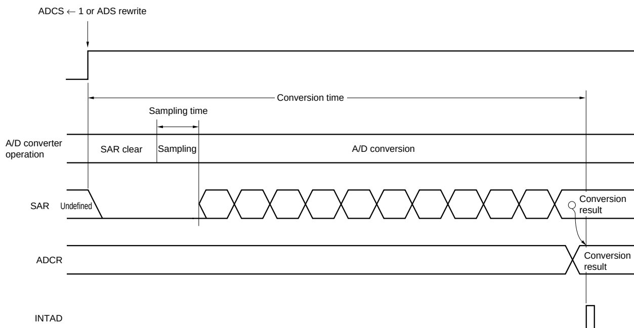
Figure 11-16. Conversion Operation of A/D Converter (Software Trigger Mode)
