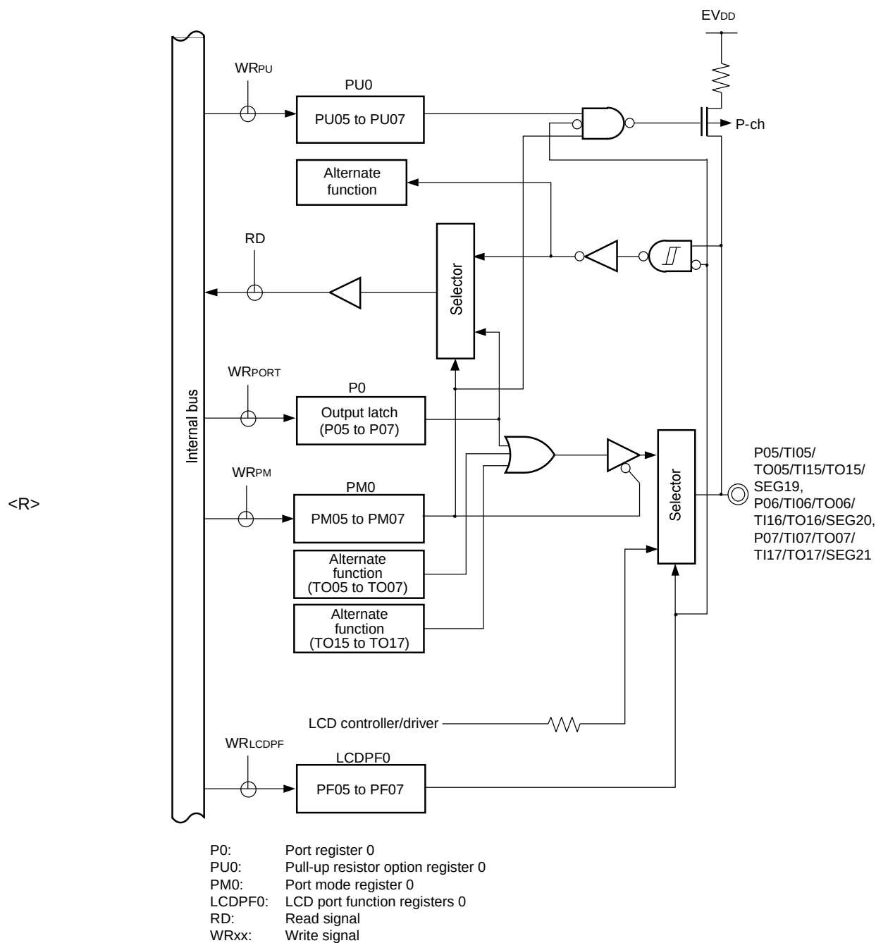
Figure 4-6. Block Diagram of P05 to P07
