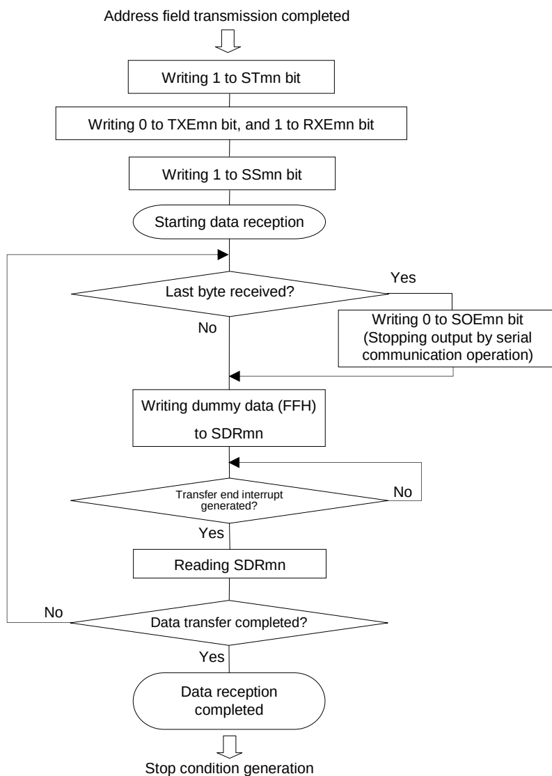
Figure 12-133. Flowchart of Data Reception
