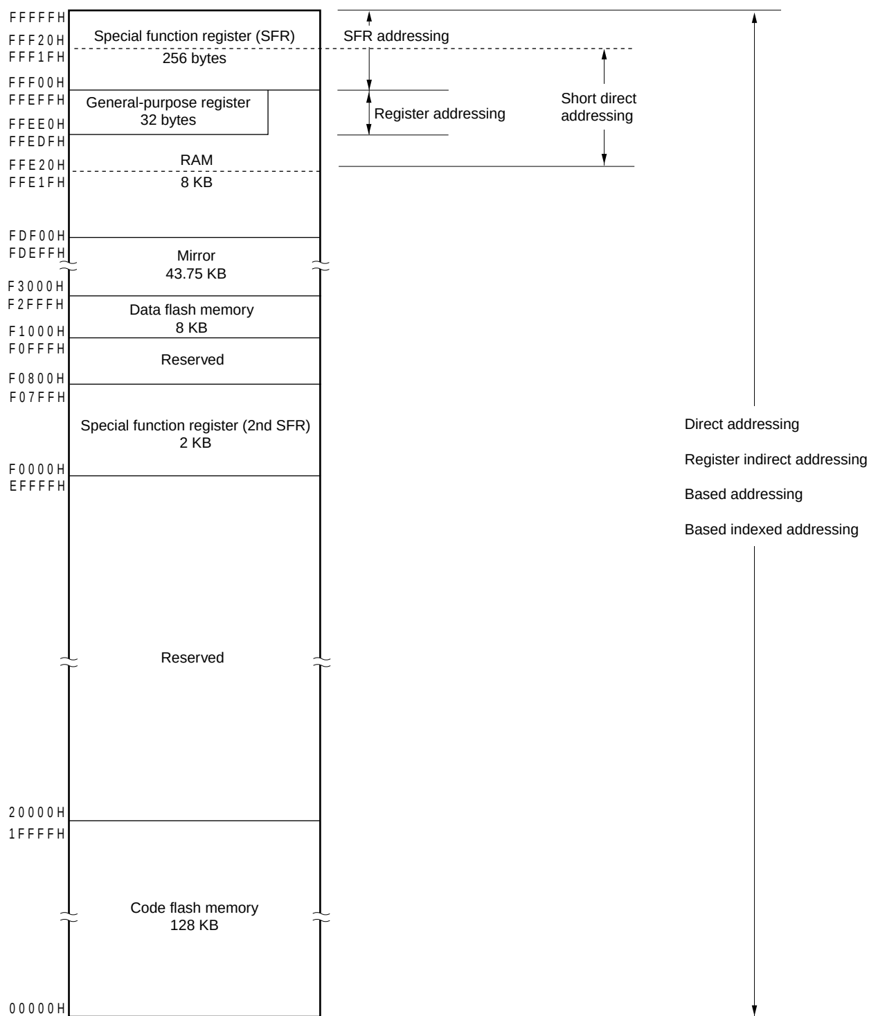
Figure 3-11. Correspondence Between Data Memory and Addressing (R5F10DMG, R5F10DPG)
