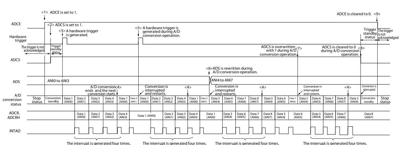
Figure 11-24. Example of Hardware Trigger No-Wait Mode (Scan Mode, Sequential Conversion Mode) Operation Timing
