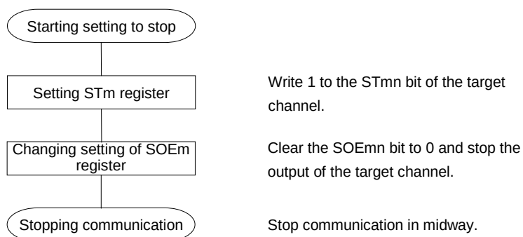
Figure 12-46. Procedure for Stopping Master Transmission/Reception
