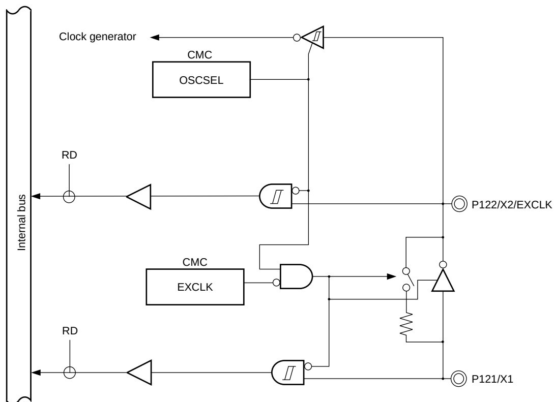
Figure 4-39. Block Diagram of P121, P122
