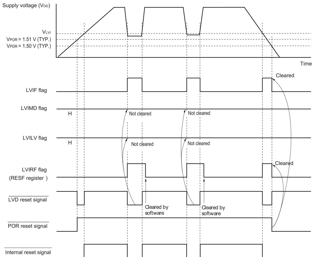
Figure 24-4. Timing of Voltage Detector Internal Reset Signal Generation (Option Byte LVIMDS1, LVIMDS0 = 1, 1)
