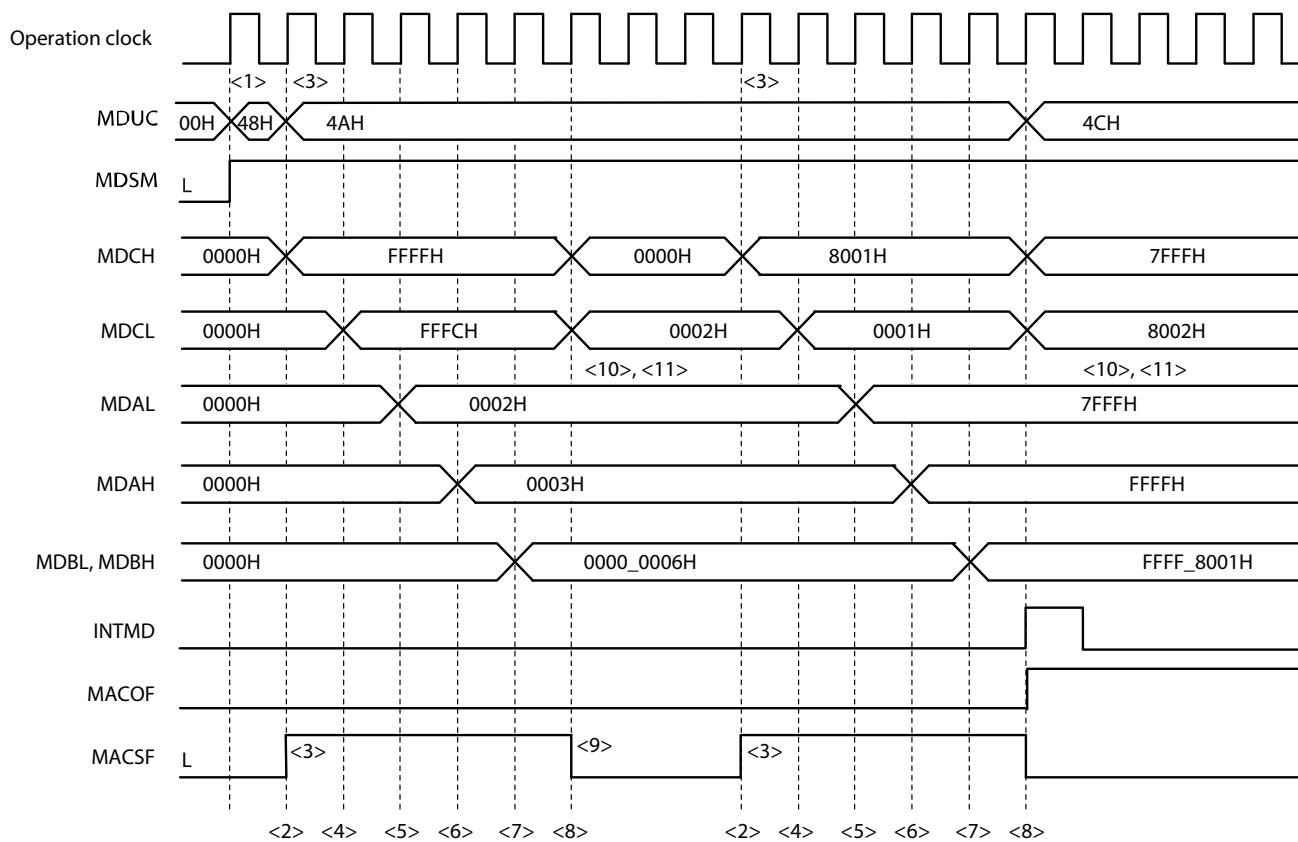
Figure 18-9. Timing Diagram of Multiply-Accumulation (signed) Operation (2 \times 3 + (-4) = 2 \rightarrow 32767 \times (-1) + (-2147483647) = -2147450882 \text{ (overflow occurs.)})
