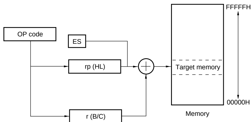
Figure 3-40 Example of ES:[HL+B], ES:[HL+C]
