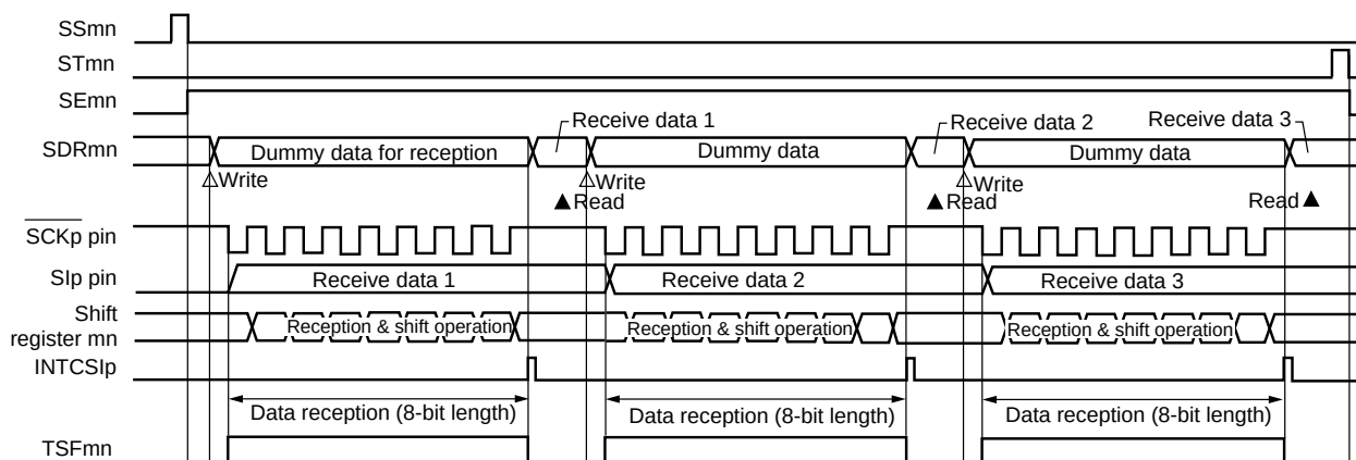
Figure 12-40. Timing Chart of Master Reception (in Single-Reception Mode)
