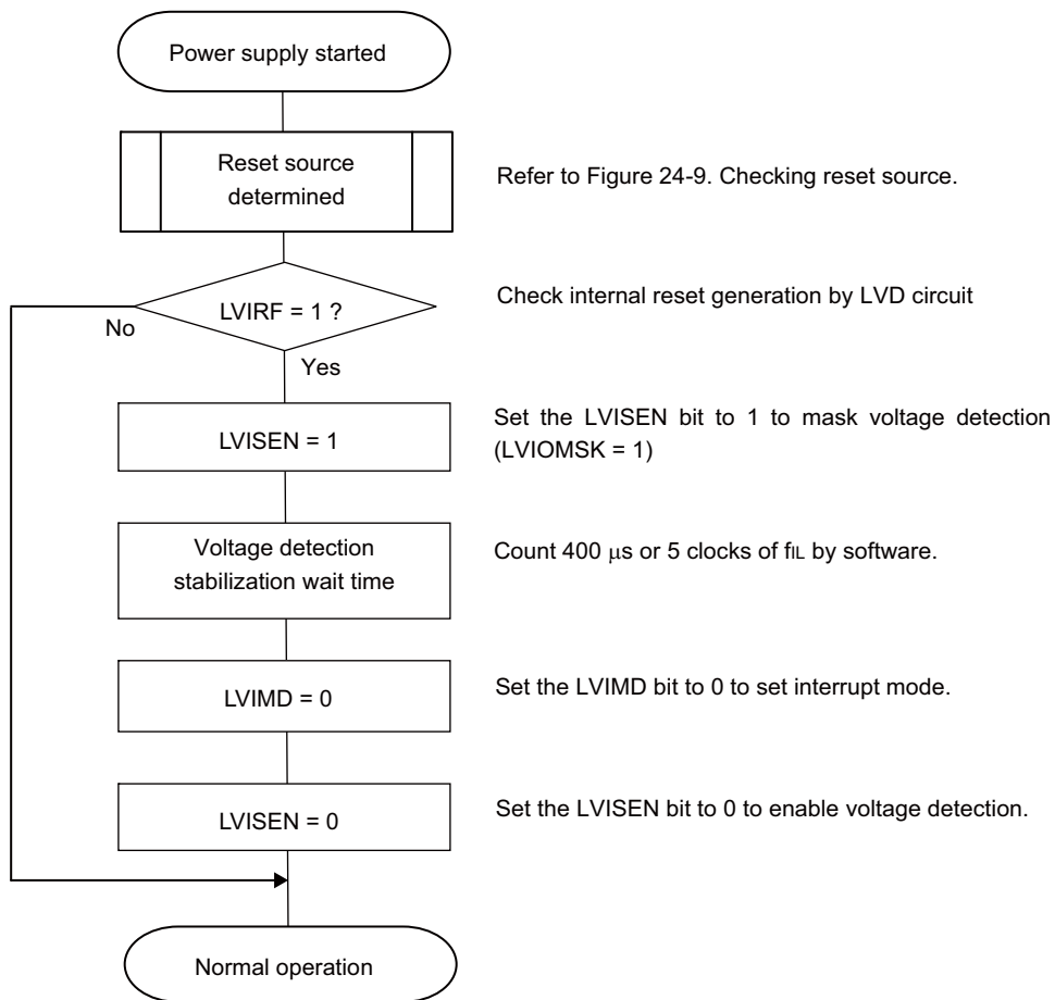
<R> Figure 24-8. Initial Setting of Interrupt and Reset Mode
