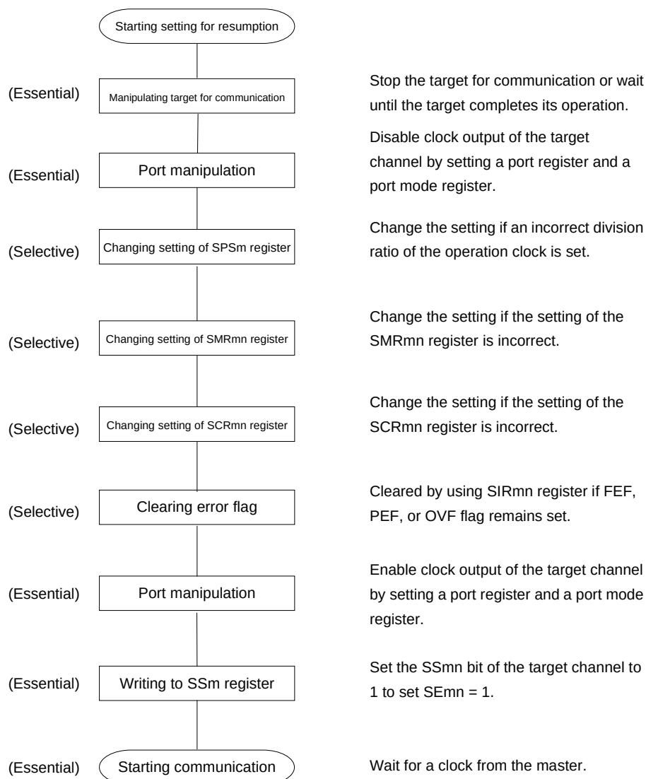
Figure 12-63. Procedure for Resuming Slave Reception
