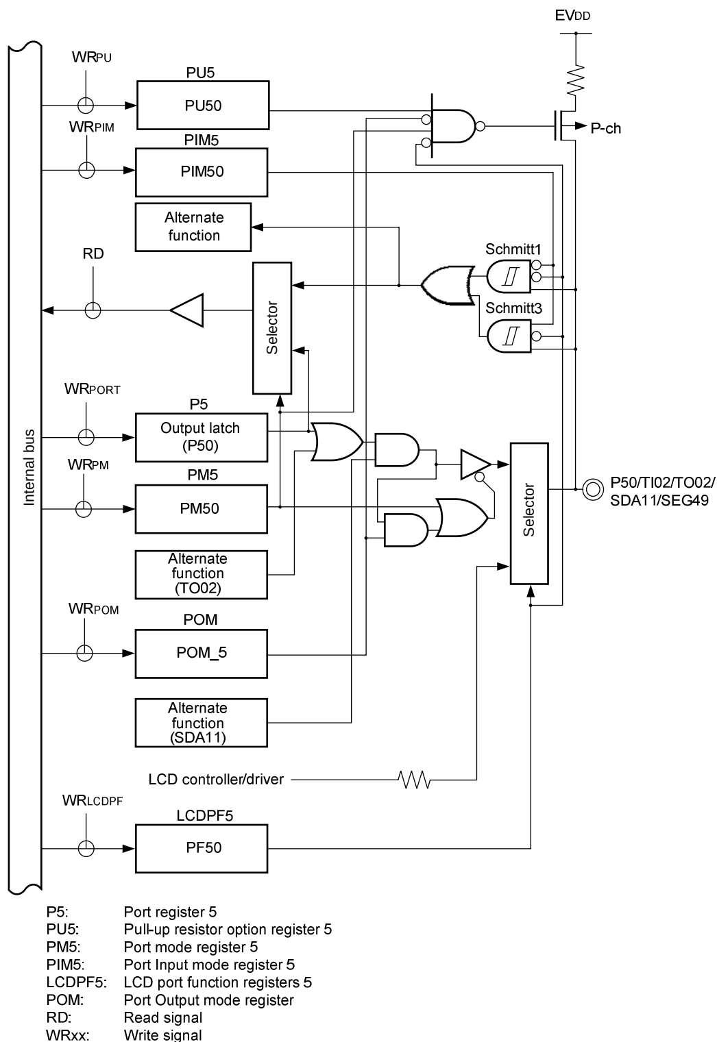
Figure 4-18. Block Diagram of P50
