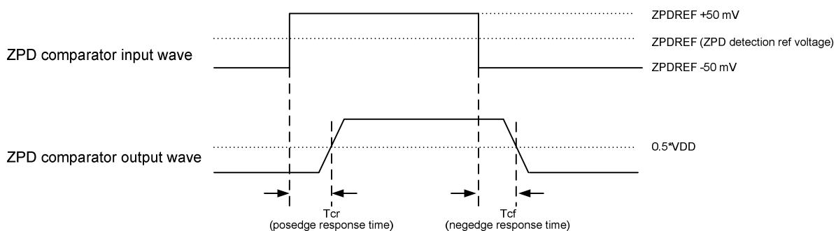
Figure 32-12. ZPD timing
