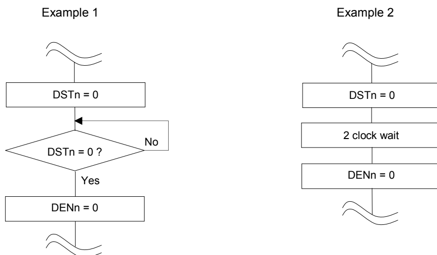
Figure 19-12. Forced Termination of DMA Transfer (1/2)
