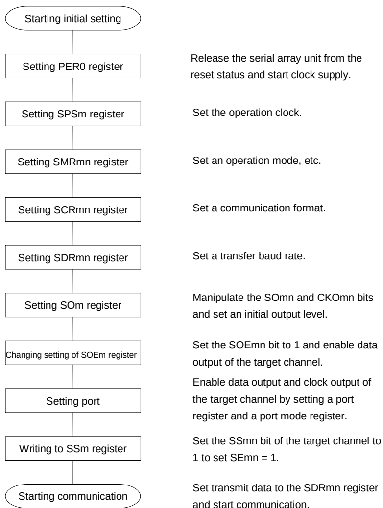
Figure 12-45. Initial Setting Procedure for Master Transmission/Reception
