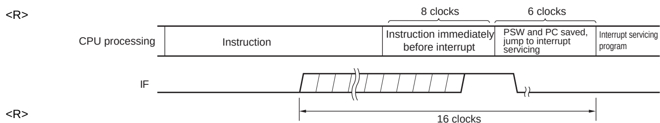
Figure 20-9. Interrupt Request Acknowledgment Timing (Maximum Time)
