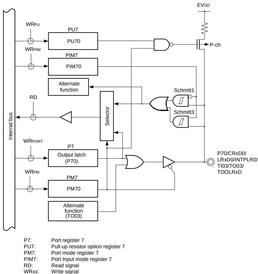
Figure 4-28. Block Diagram of P70
