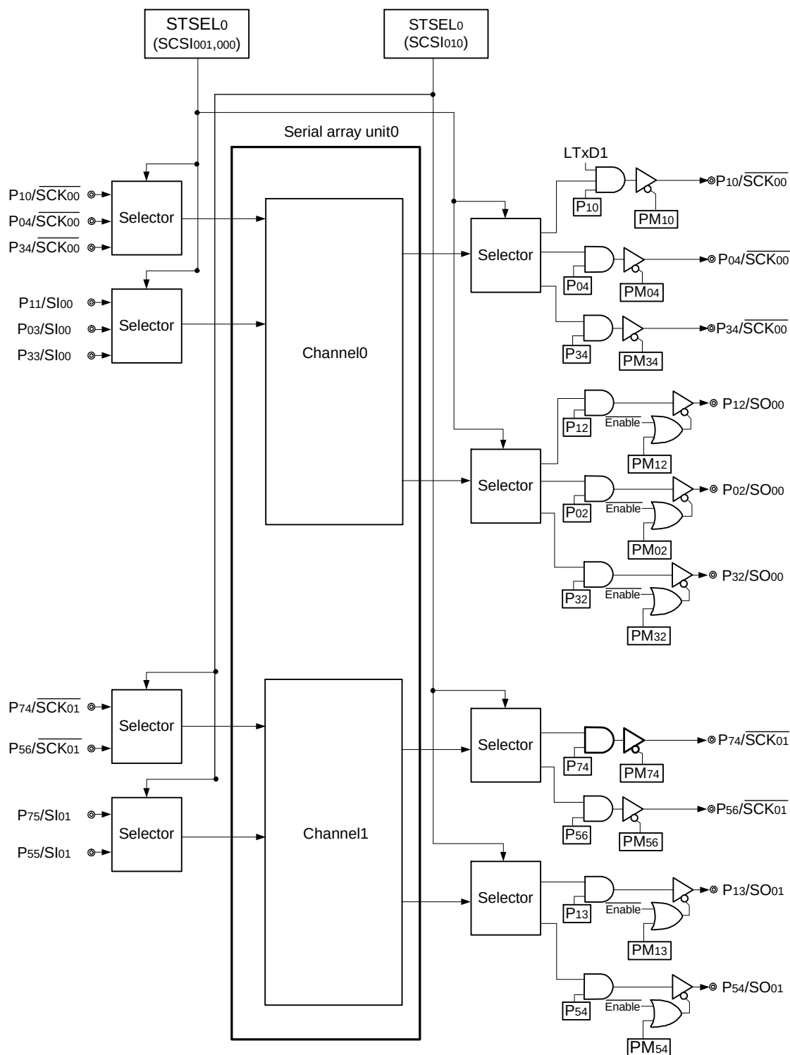
Figure 12-2. Port Configuration Diagram of Serial Array Unit 0
