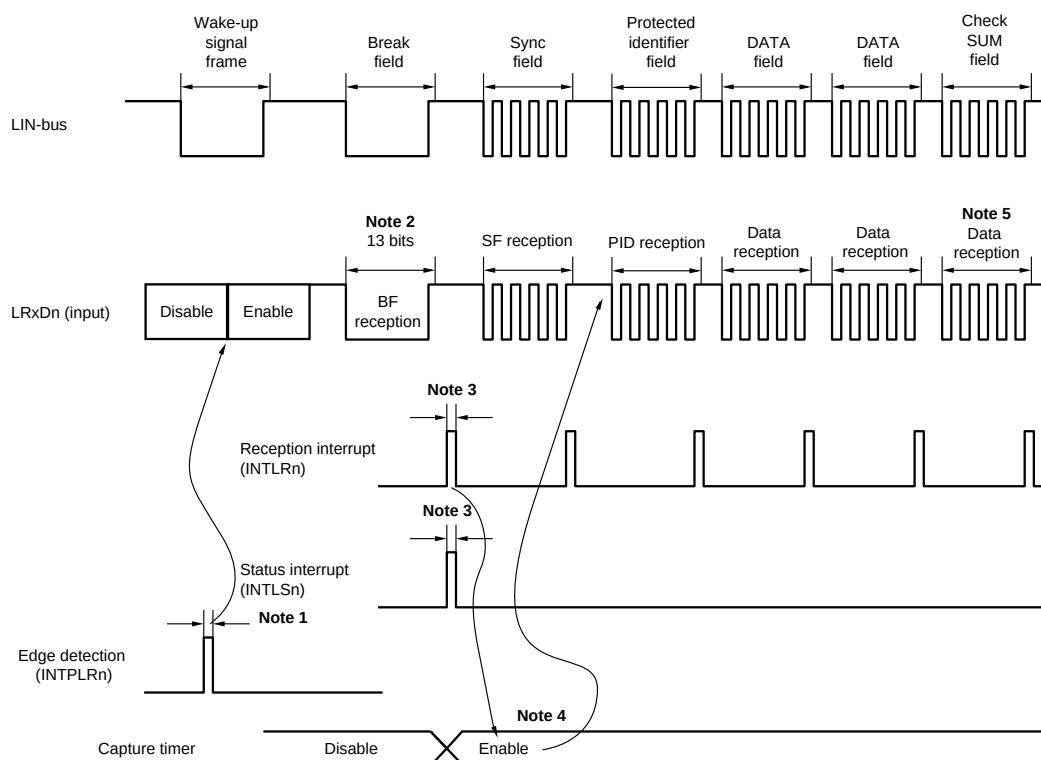
Figure 13-29. LIN Reception Manipulation Outline
