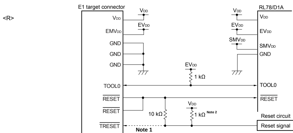
Figure 29-1. Connection Example of E1 On-chip Debugging Emulator and RL78/D1A
