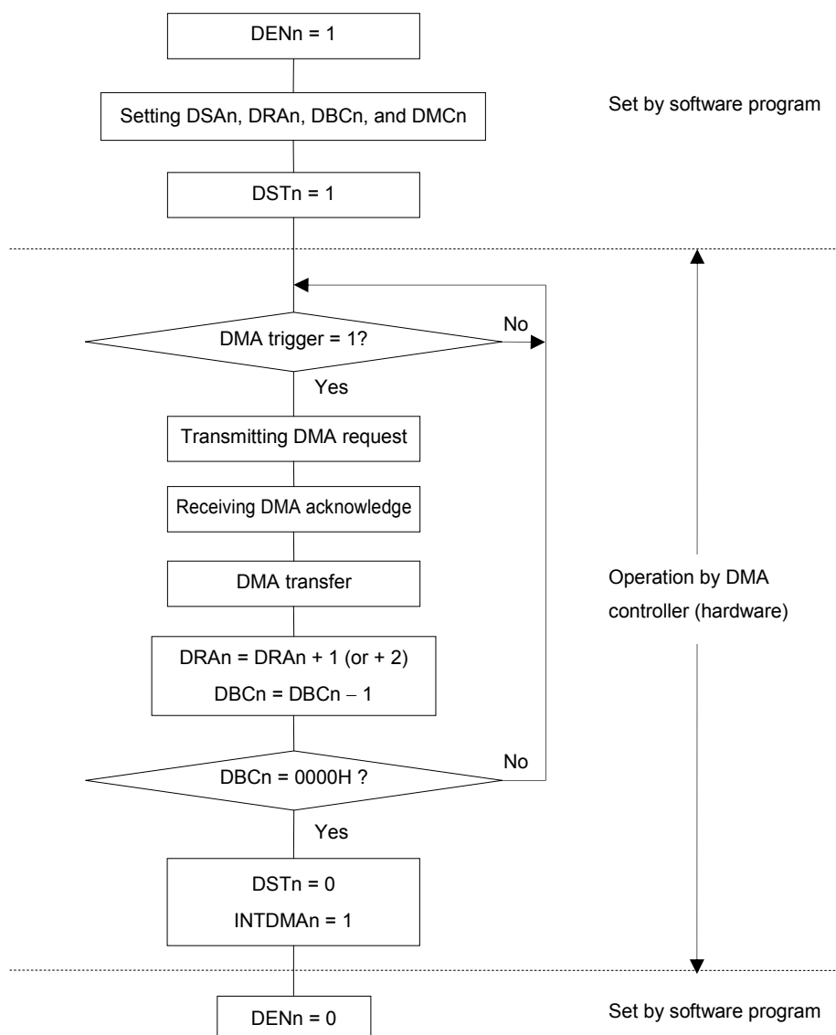
Figure 19-7. Operation Procedure
