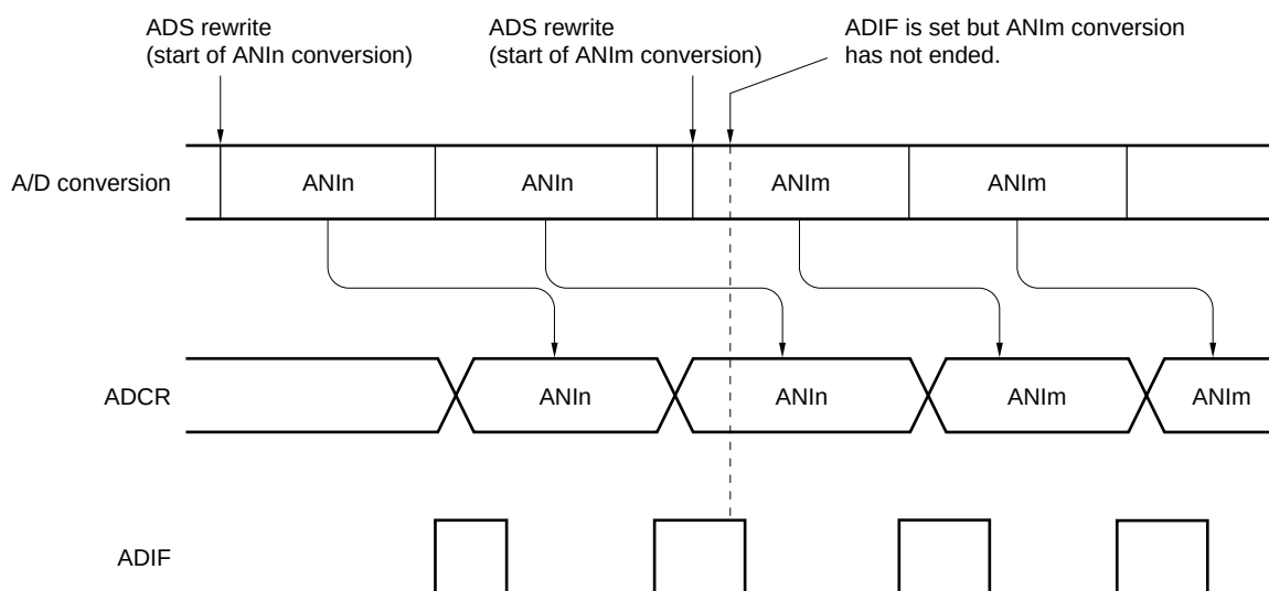
Figure 11-44. Timing of A/D Conversion End Interrupt Request Generation
