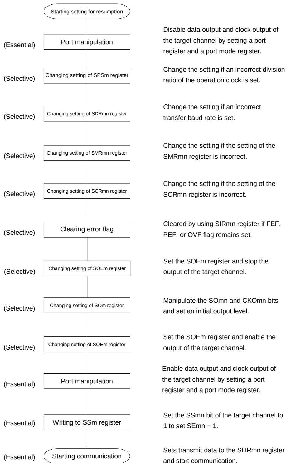
Figure 12-31. Procedure for Resuming Master Transmission
