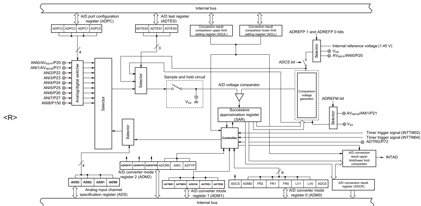
Figure 11-1. Block Diagram of A/D Converter
