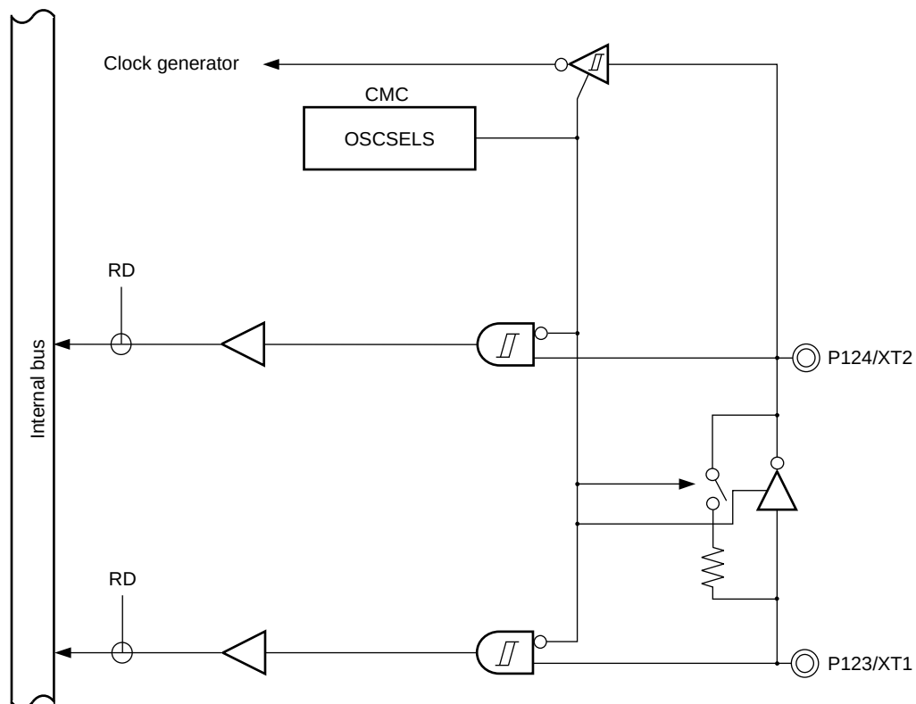
Figure 4-40. Block Diagram of P123, P124
