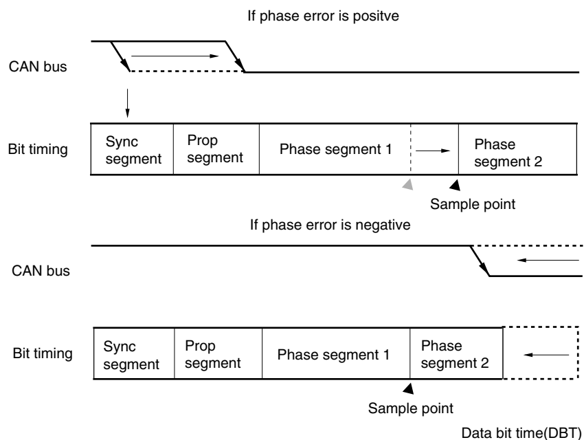
Figure 14-21. Resynchronization
