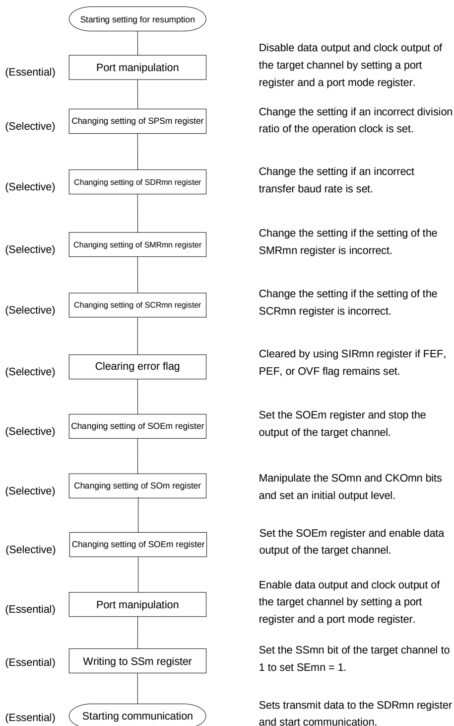
Figure 12-47. Procedure for Resuming Master Transmission/Reception
