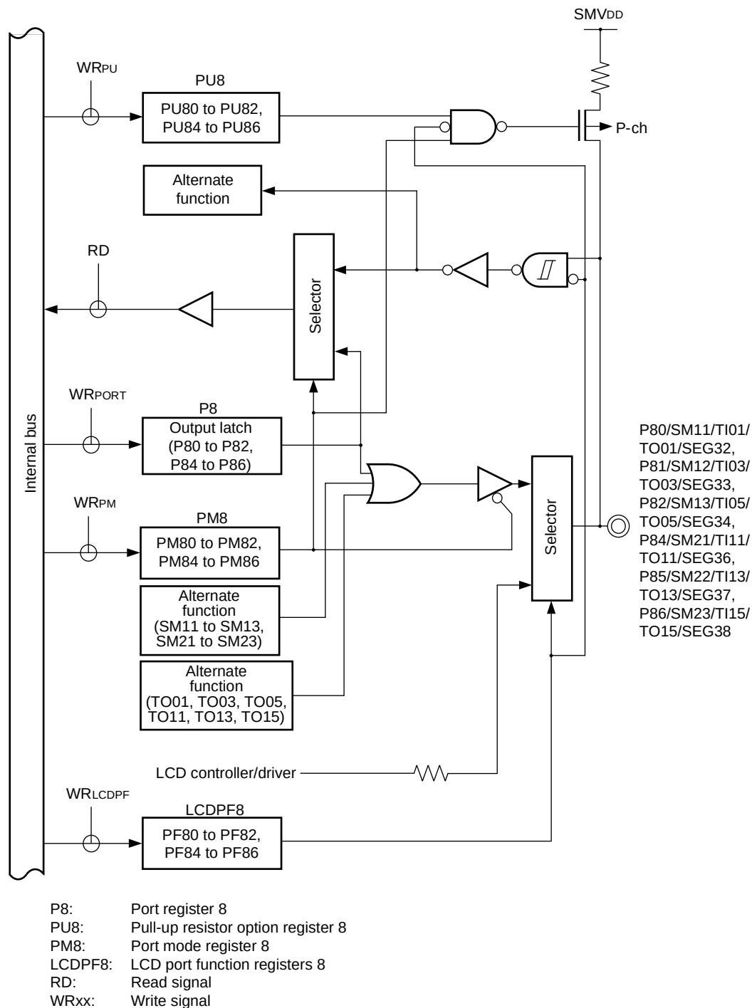
Figure 4-33. Block Diagram of P80 to P82 and P84 to P86
