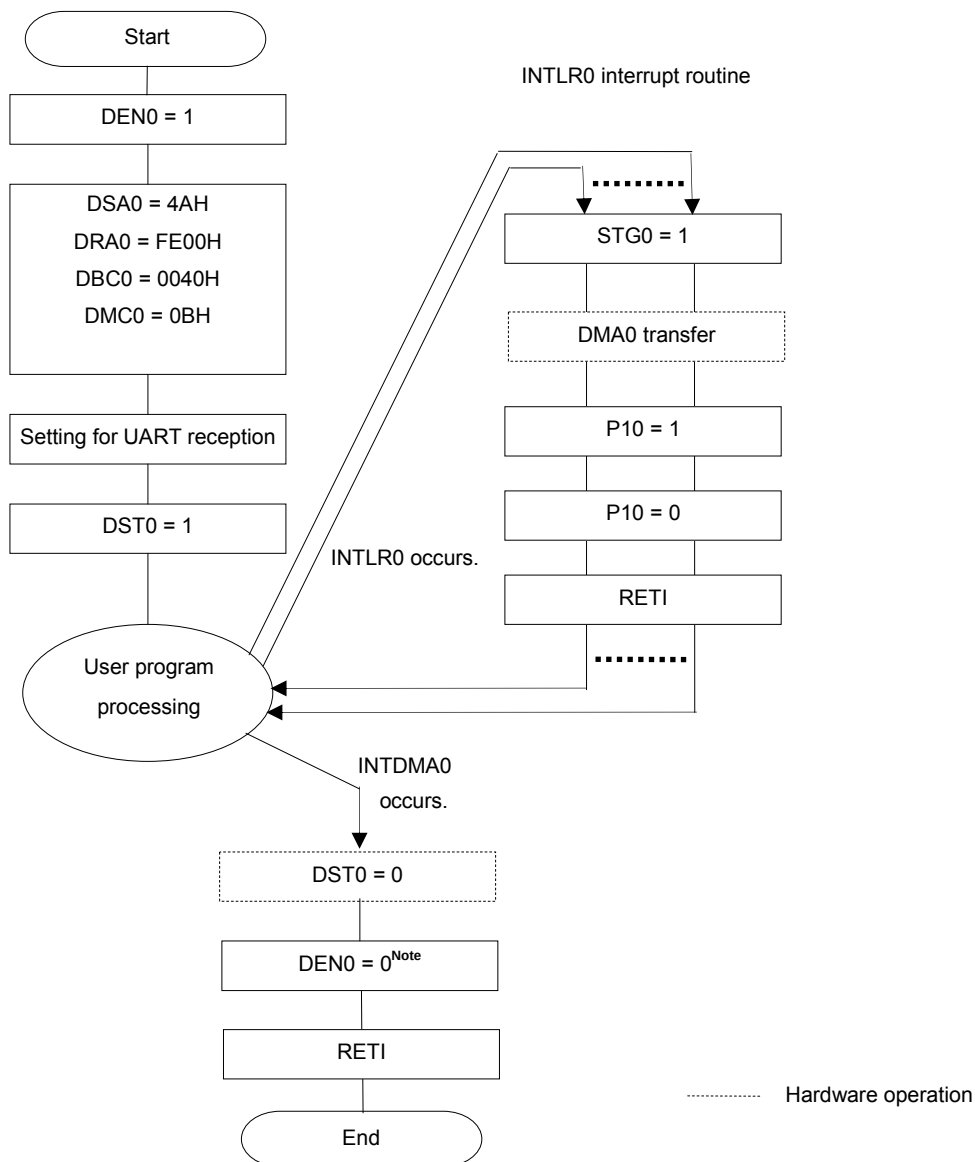
Figure 19-10. Example of Setting for UART Consecutive Reception + ACK Transmission
