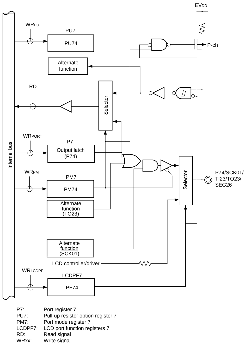
Figure 4-31. Block Diagram of P74
