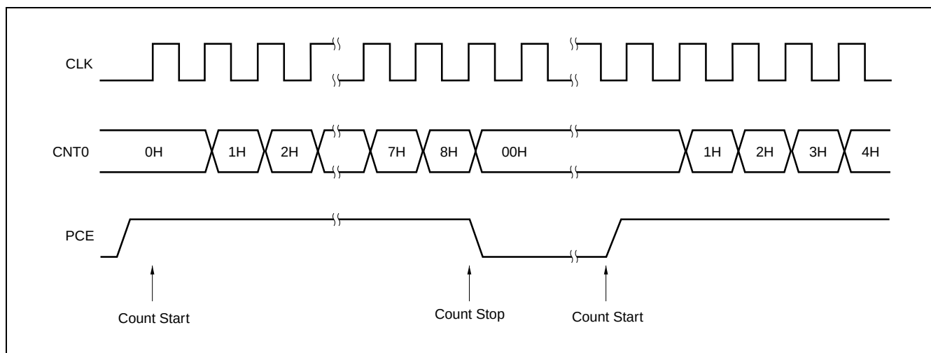
Figure 15-10. Restart Timing after Count Stop (Count Start—Count Stop—Count Start)
