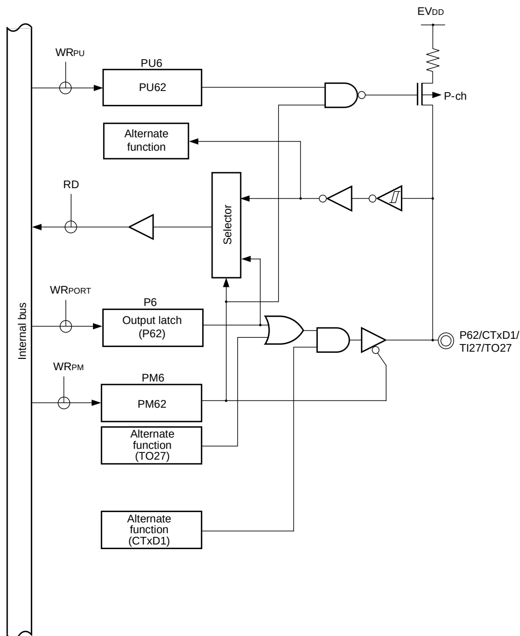
Figure 4-24. Block Diagram of P62
