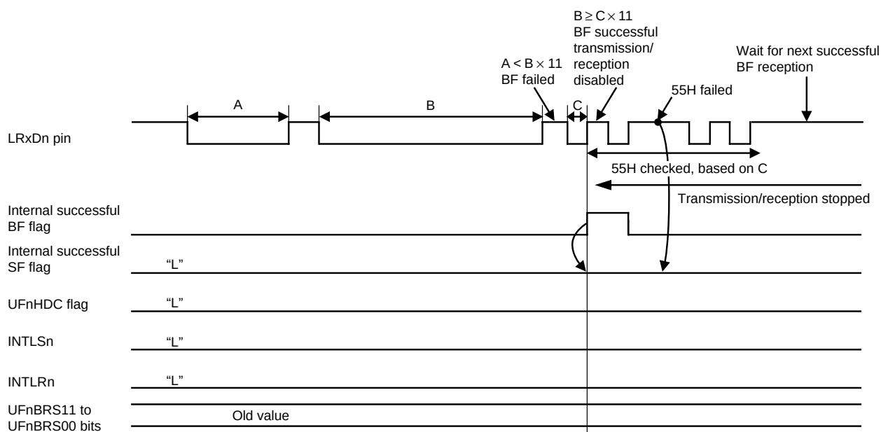
Figure 13-56. Example of BF/SF Reception Failure
