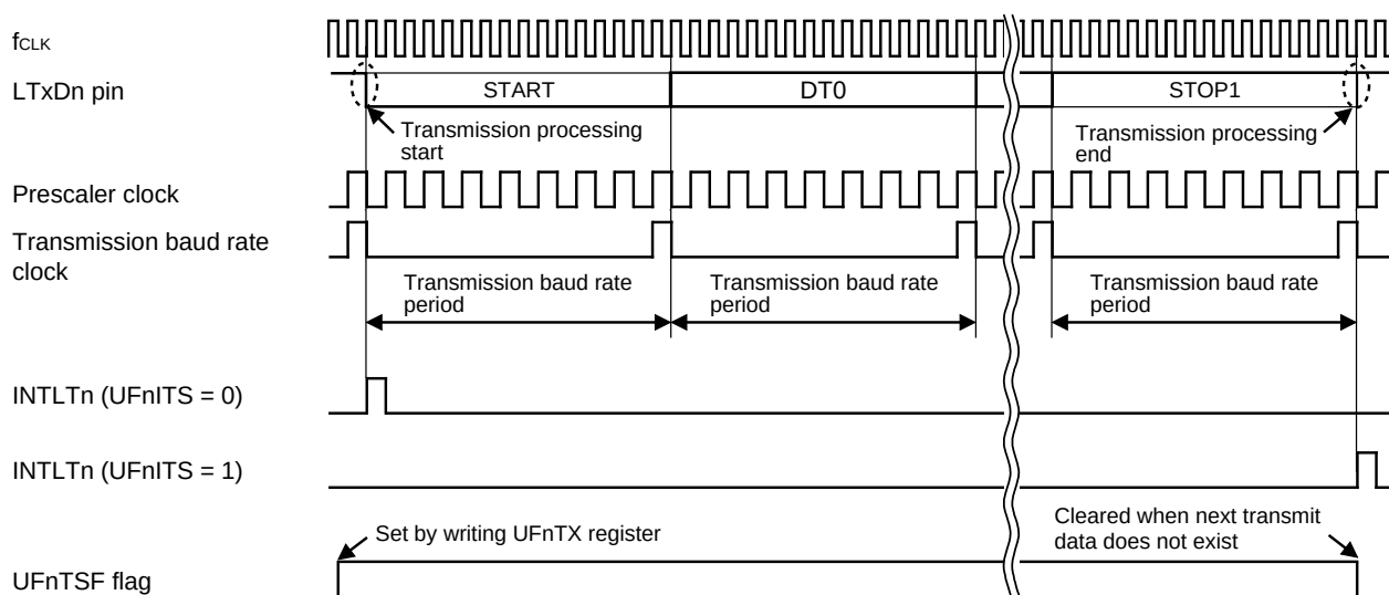
Figure 13-23. Data Transmission Timing Chart
