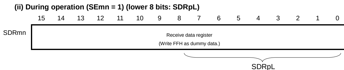
Figure 12-36. Example of Contents of Registers for Master Reception of 3-Wire Serial I/O (CSI00, CSI01, CSI10) (2/2)
