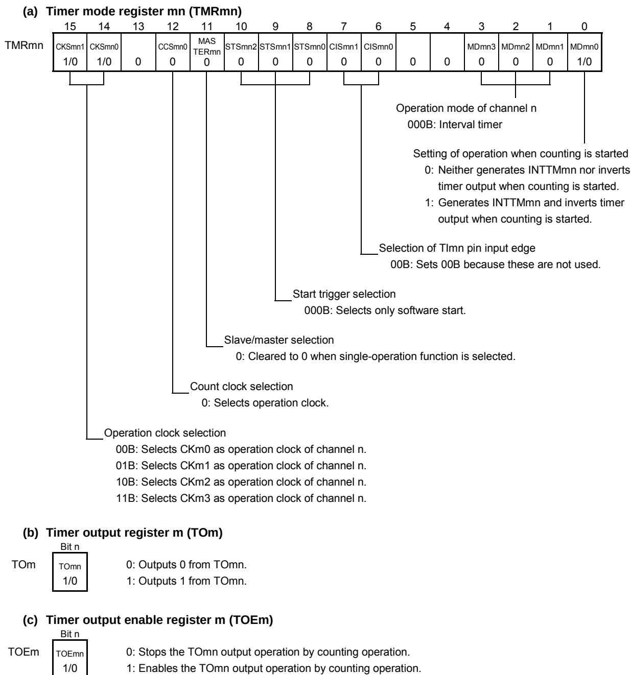
Figure 6-53. Example of Set Contents of Registers During Operation as Interval Timer/Square Wave Output (1/2)
