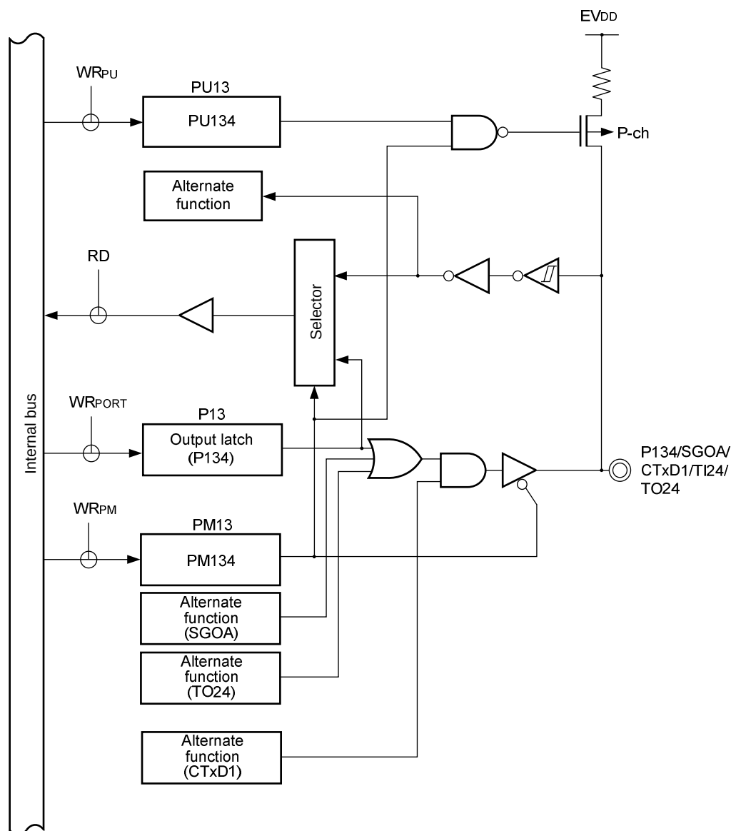
Figure 4-45. Block Diagram of P134
