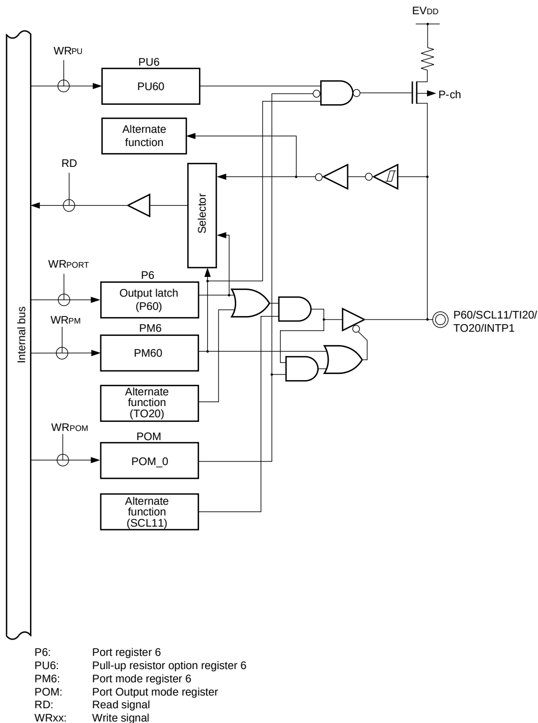
Figure 4-22. Block Diagram of P60
