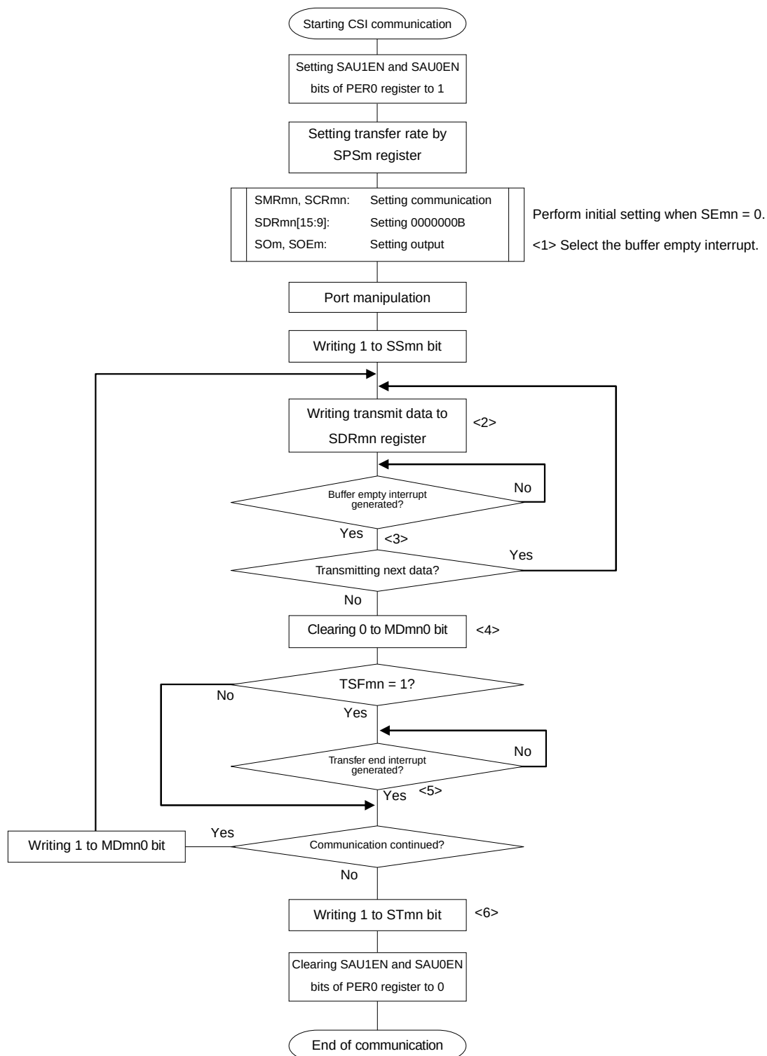
Figure 12-59. Flowchart of Slave Transmission (in Continuous Transmission Mode)
