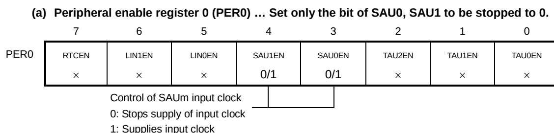
Figure 12-26. Peripheral Enable Registers 0 (PER0) Setting When Stopping the Operation by Units
