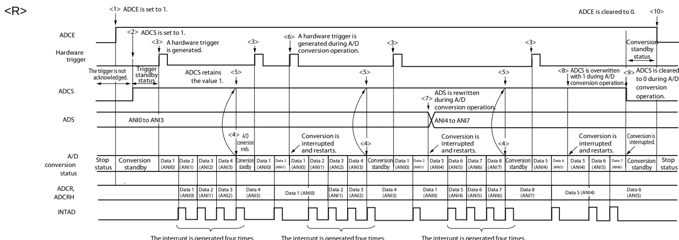
Figure 11-25. Example of Hardware Trigger No-Wait Mode (Scan Mode, One-Shot Conversion Mode) Operation Timing
