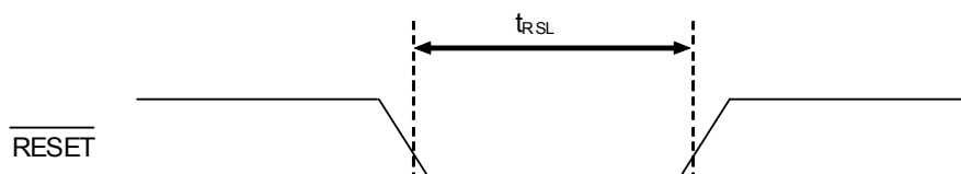
Figure 33-5. \overline{\text{RESET}} Input Timing
