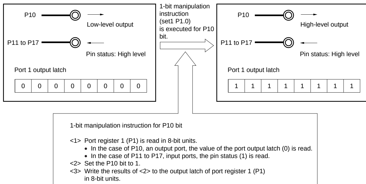
Figure 4-72. Bit Manipulation Instruction (P10)
