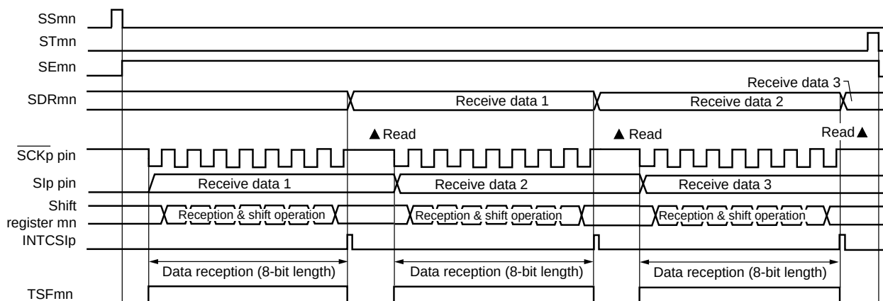
Figure 12-64. Timing Chart of Slave Reception (in Single-Reception Mode)
