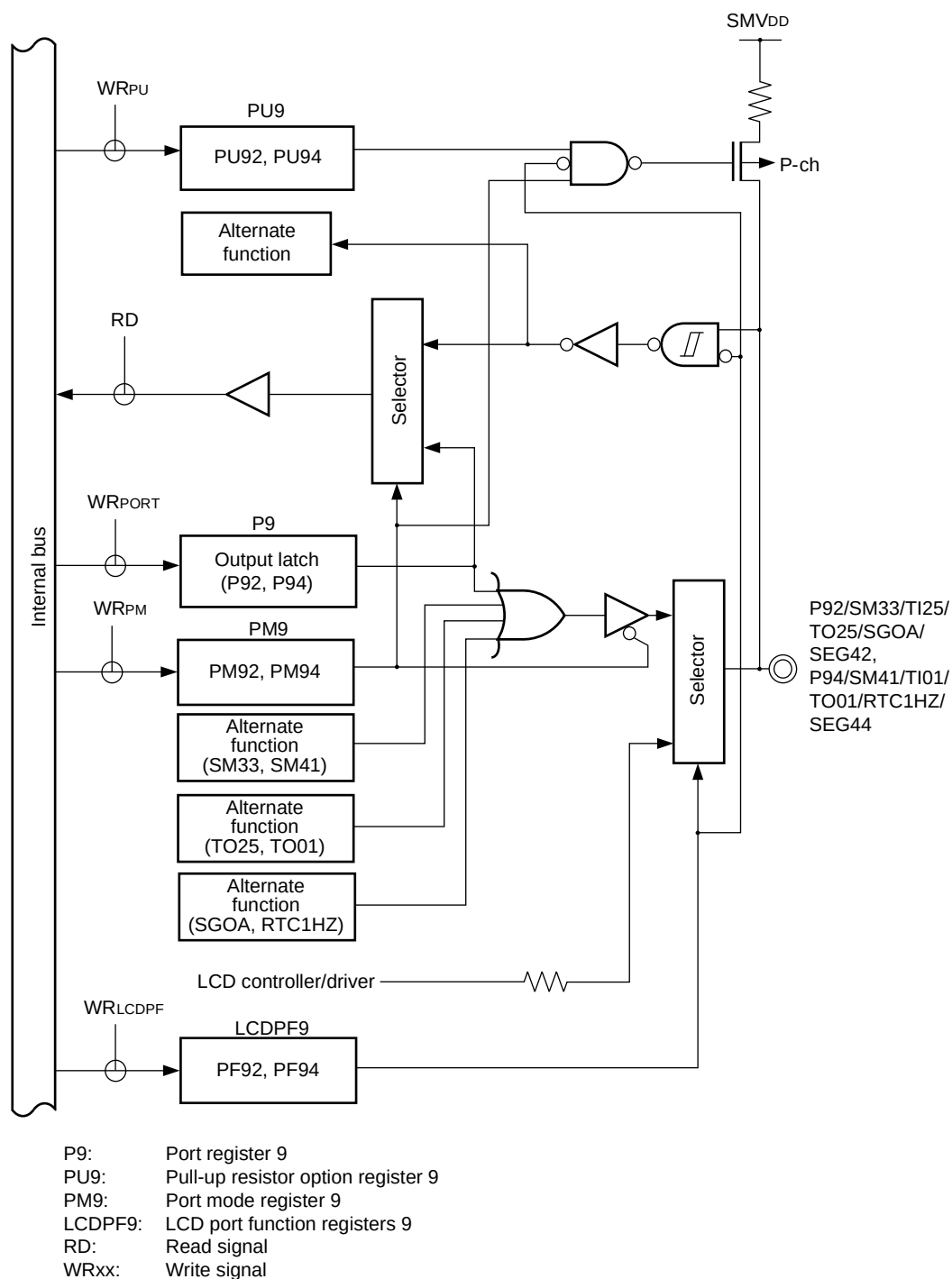
Figure 4-36. Block Diagram of P92, P94
