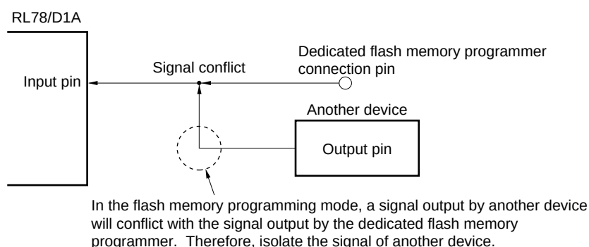
Figure 28-5. Signal Conflict ( \overline{\text{RESET}} Pin)
