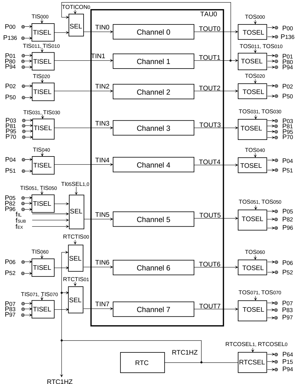
Figure 4-59. Timer Array unit and RTC I/O connection (1/3)
