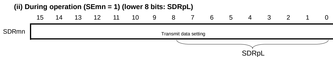
Figure 12-28. Example of Contents of Registers for Master Transmission of 3-Wire Serial I/O (CSI00, CSI01, CSI10) (2/2)
