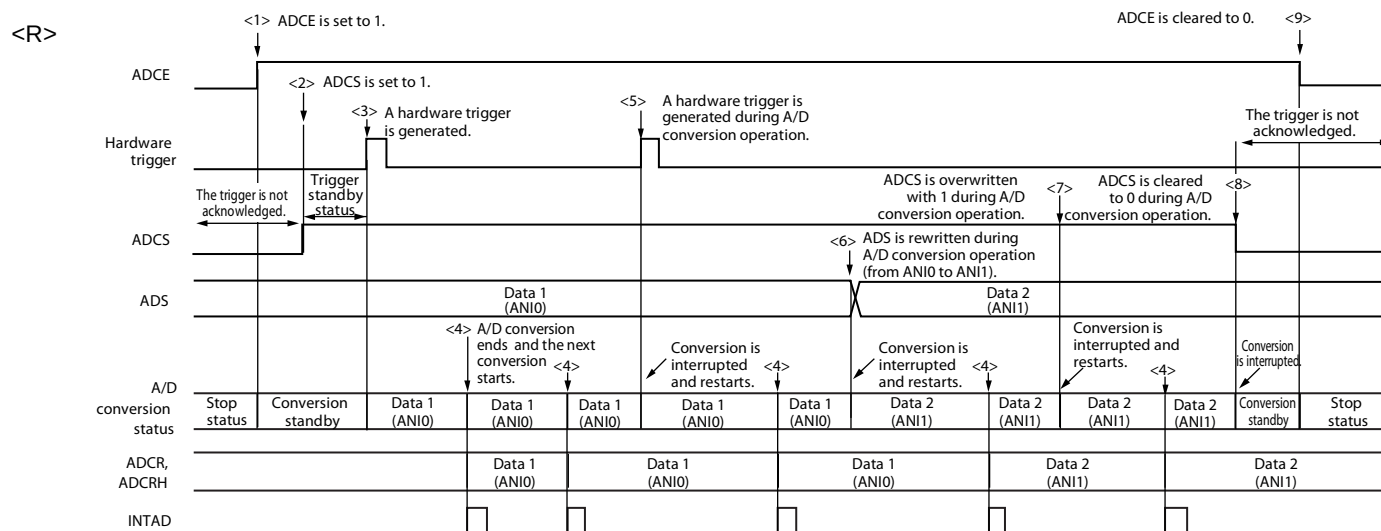
Figure 11-22. Example of Hardware Trigger No-Wait Mode (Select Mode, Sequential Conversion Mode) Operation Timing
