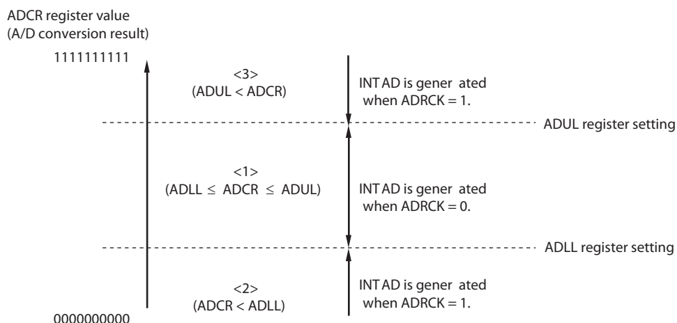
Figure 11-8. ADRCK Bit Interrupt Signal Generation Range
