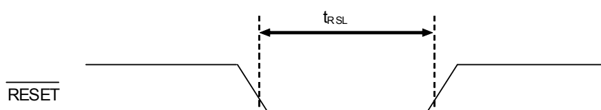
Figure 32-5. \overline{\text{RESET}} Input Timing
