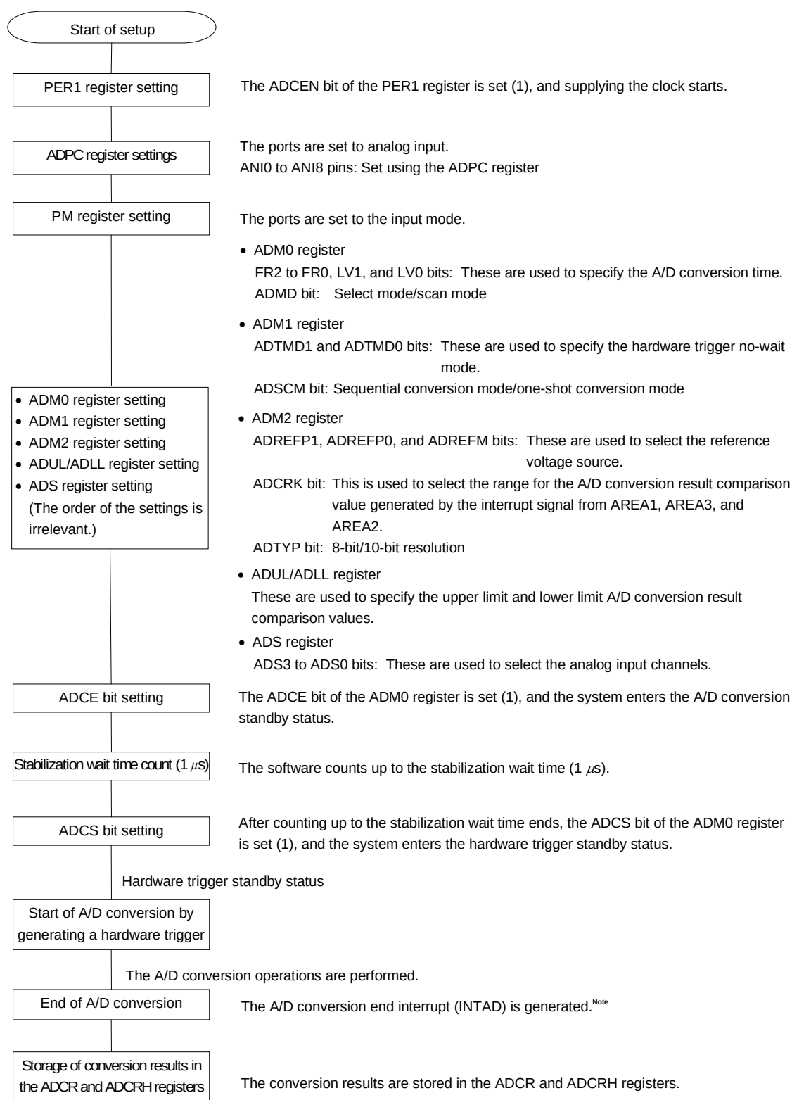
Figure 11-31. Setting up Hardware Trigger No-Wait Mode
