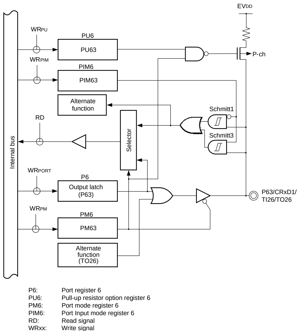
Figure 4-25. Block Diagram of P63
