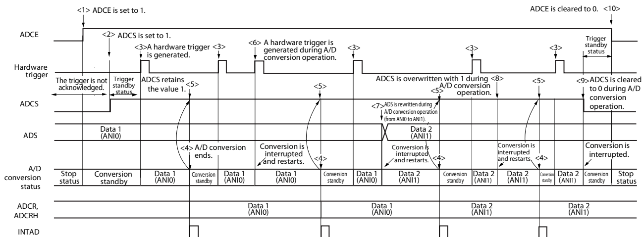
Figure 11-23. Example of Hardware Trigger No-Wait Mode (Select Mode, One-Shot Conversion Mode) Operation Timing
