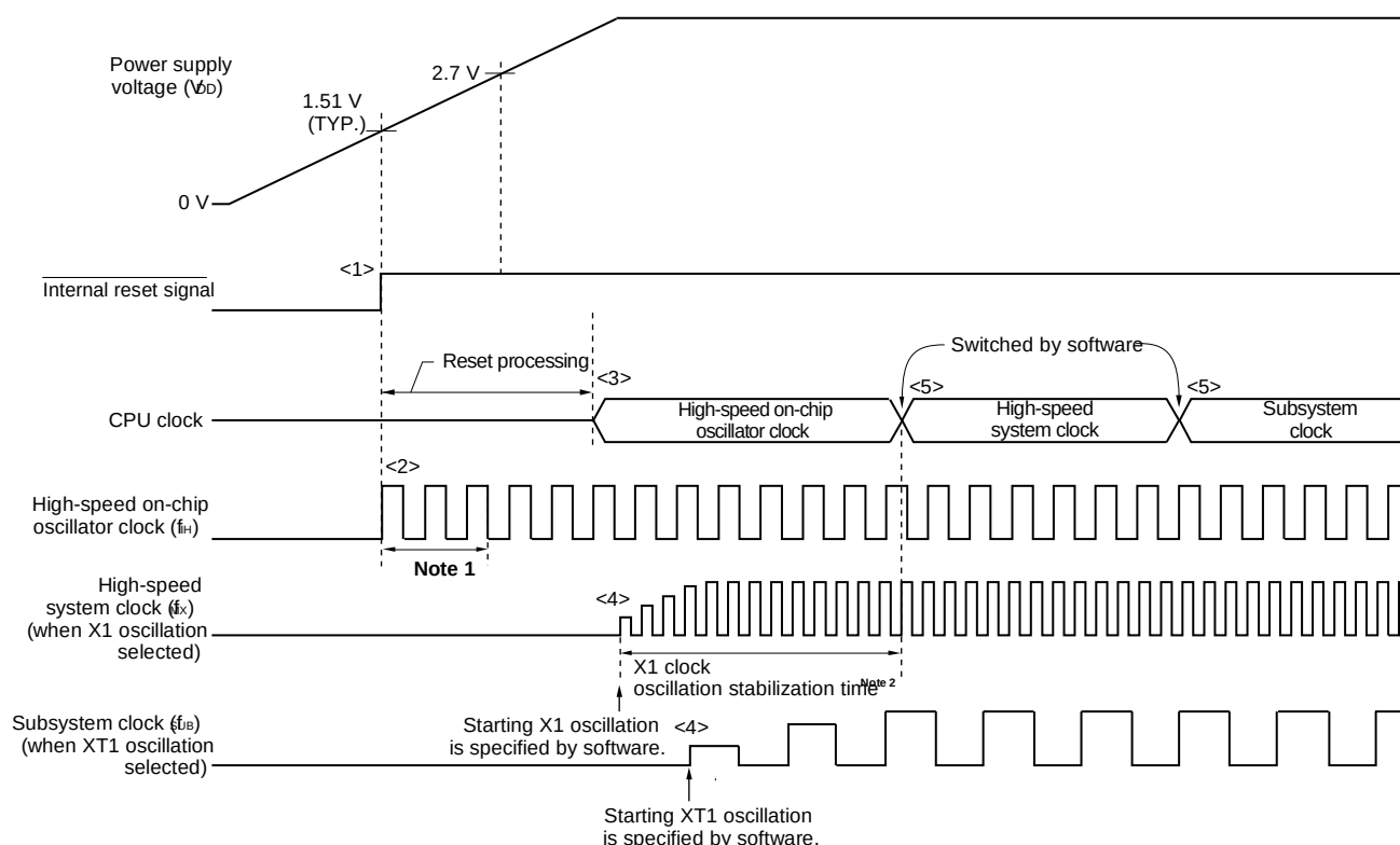
Figure 5-19. Clock Generator Operation When Power Supply Voltage Is Turned On
