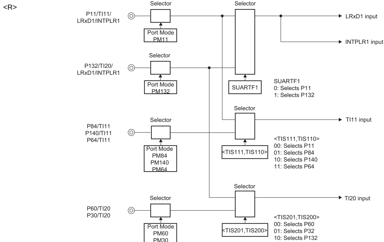
Figure 13-31. Port Configuration of LIN Reception Manipulation
