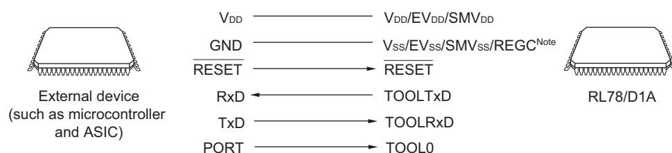
Figure 28-4. Communication with External Device
