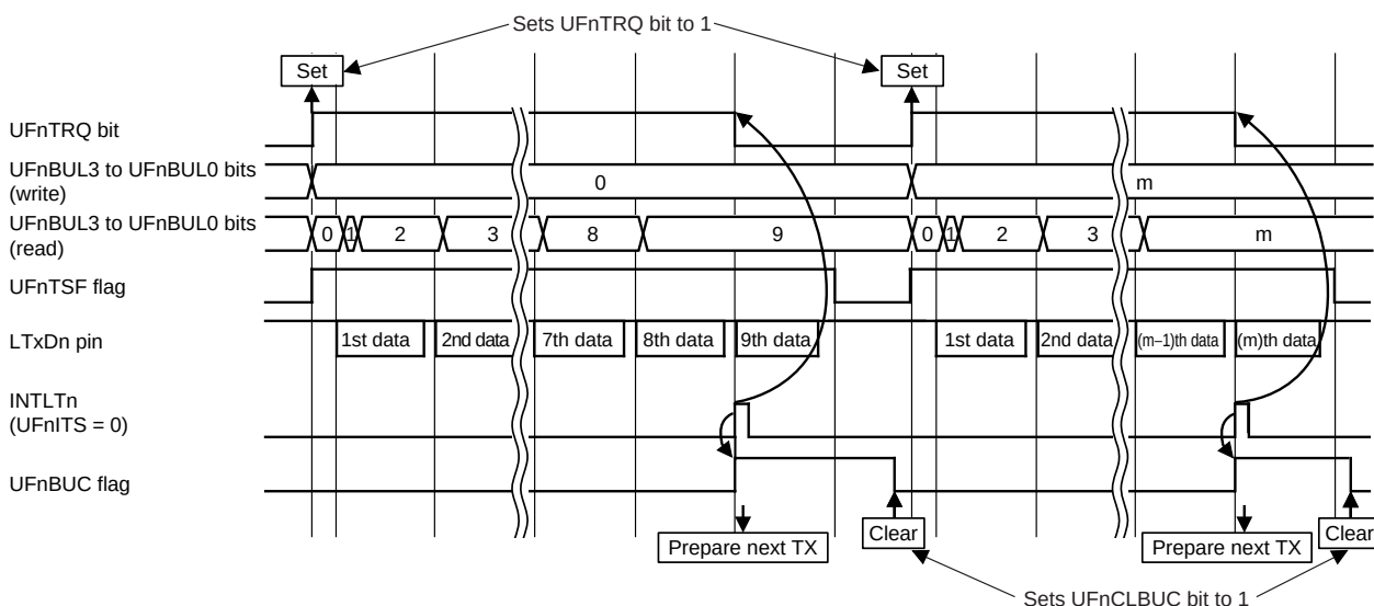
Figure 13-50. UART Buffer Mode Transmission Example (UFnITS = 0)
