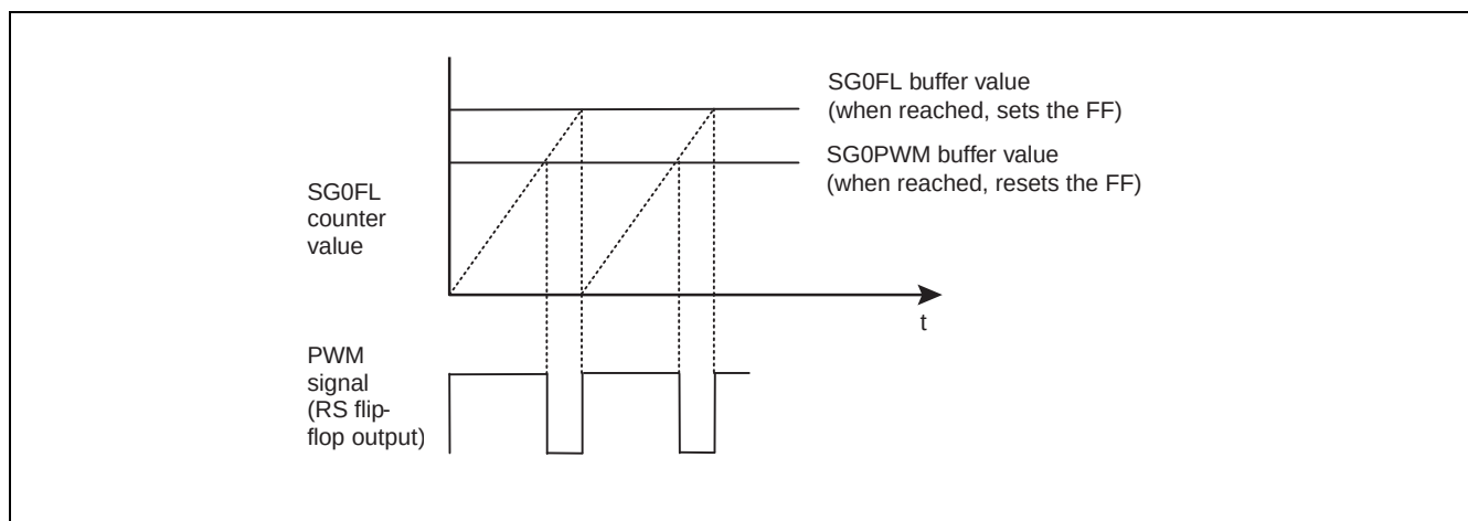
Figure 17-6. PWM Signal Generation
