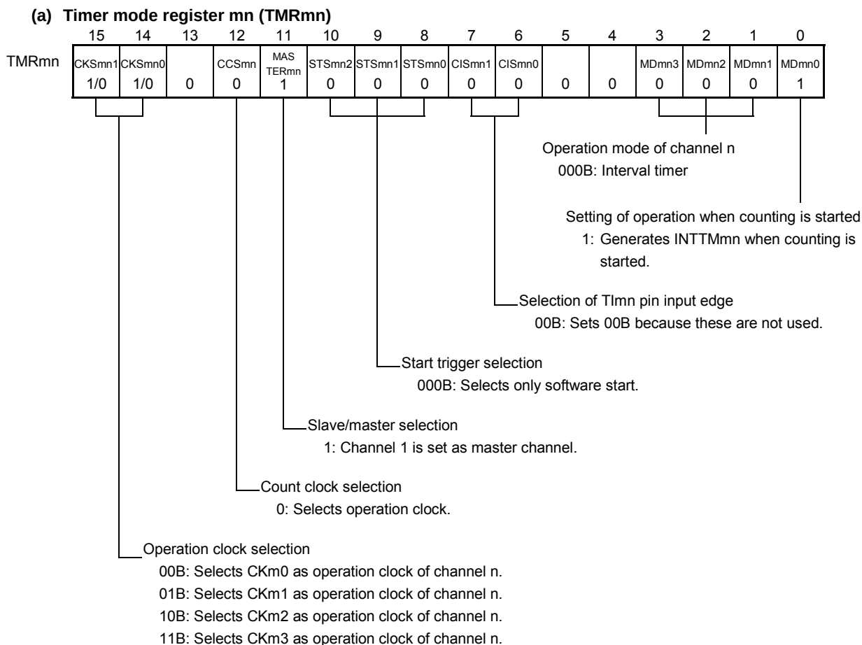
Figure 6-83. Example of Set Contents of Registers When Multiple PWM Output Function (Master Channel) Is Used (1/2)
