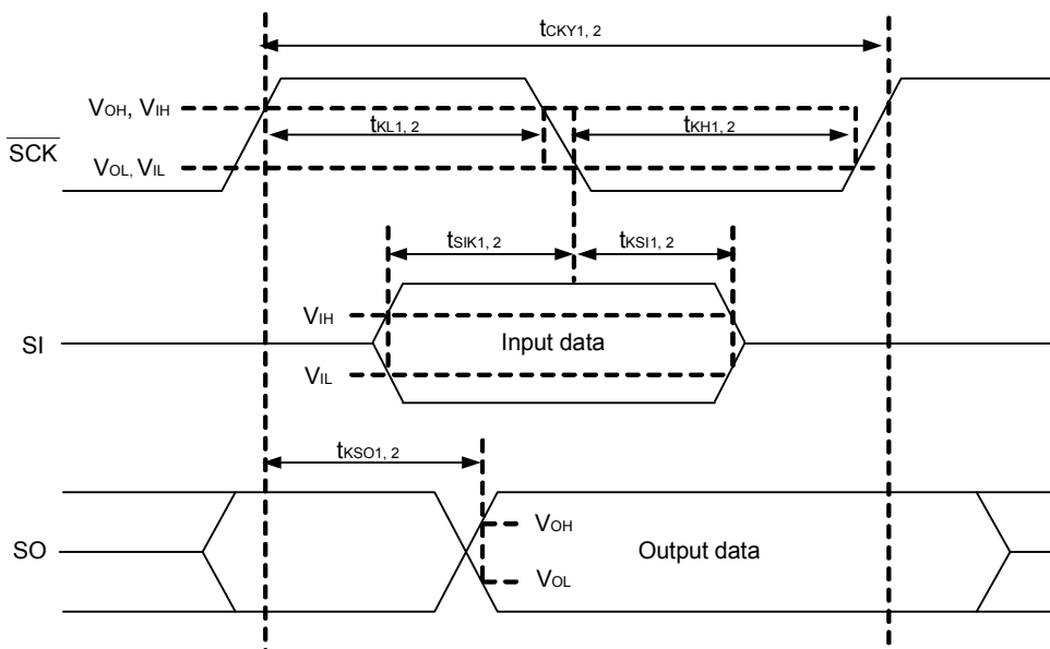
Figure 32-8. CSI mode serial transfer timing (When DAPmn = 0 and CKPmn = 1, or DAPmn = 1 and CKPmn = 0.)
