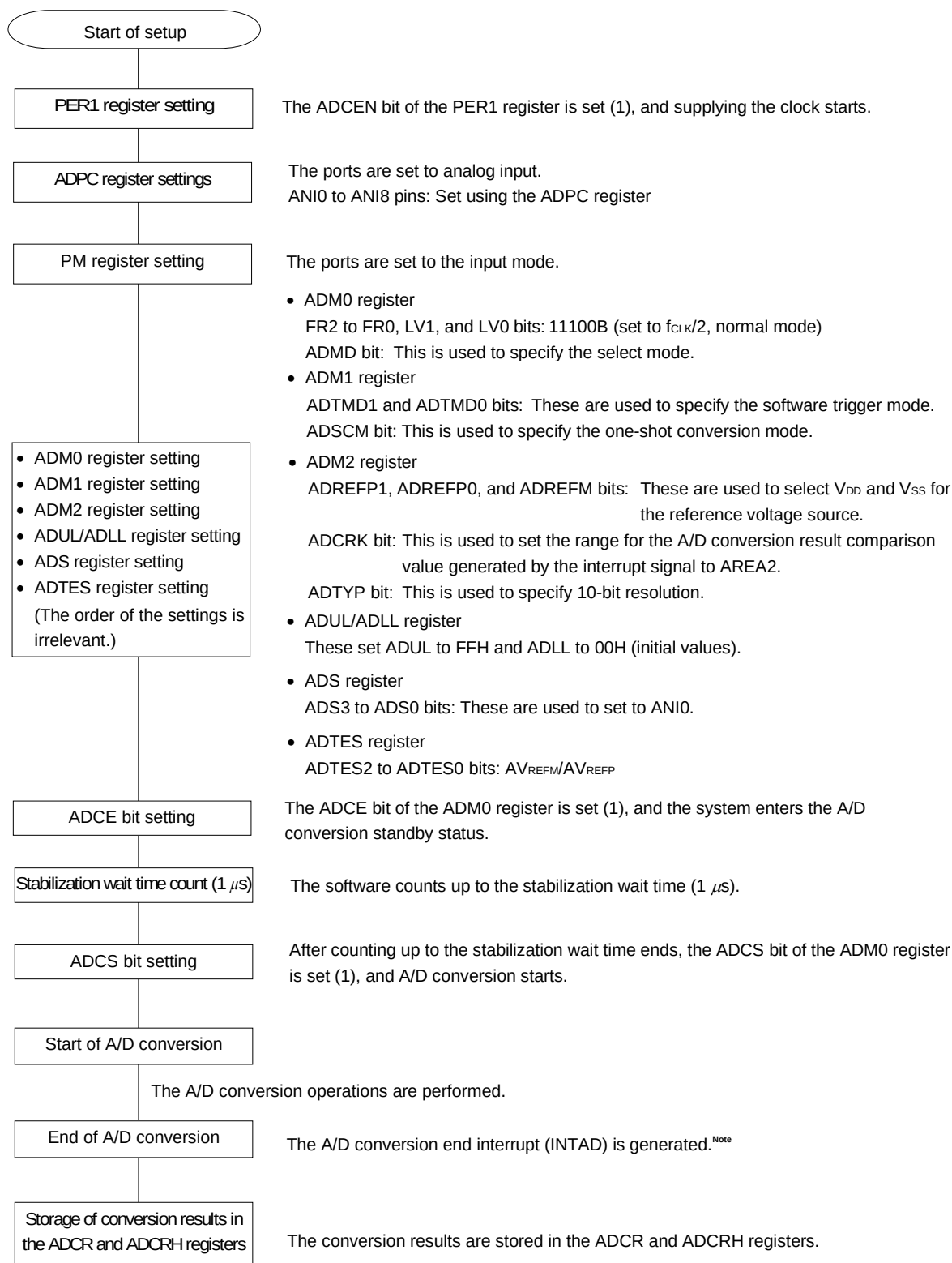
Figure 11-33. Setting up Test Trigger Mode
