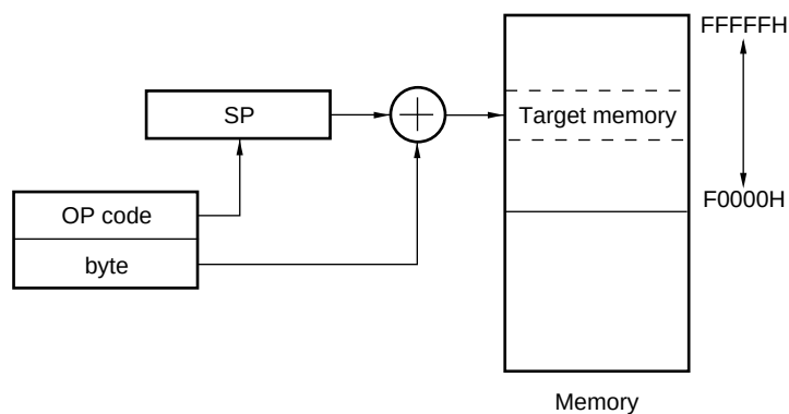
Figure 3-32. Example of [SP+byte]
