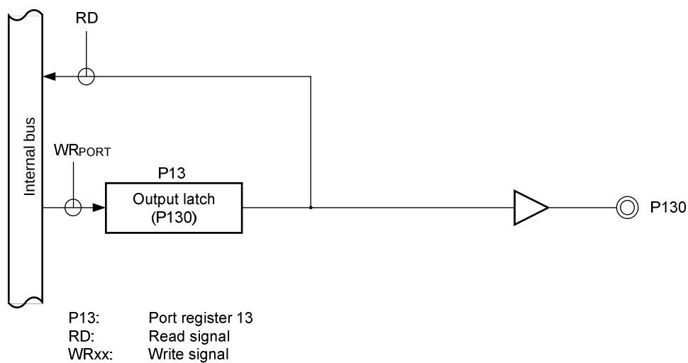
Figure 4-41. Block Diagram of P130
