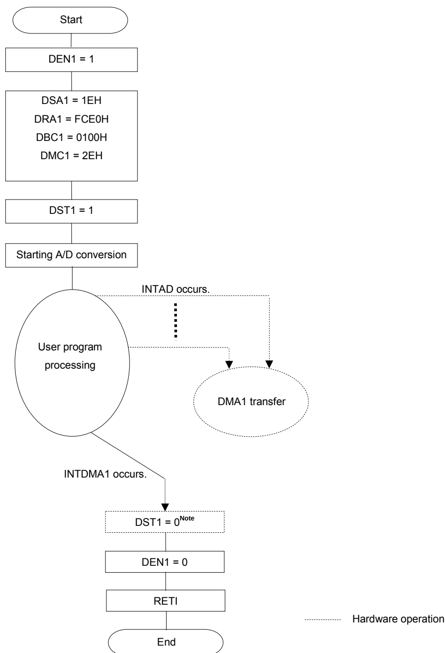
Figure 19-9. Example of Setting of Consecutively Capturing A/D Conversion Results
