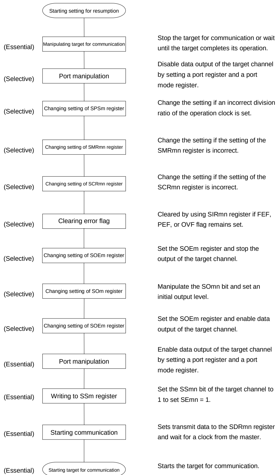
Figure 12-55. Procedure for Resuming Slave Transmission
