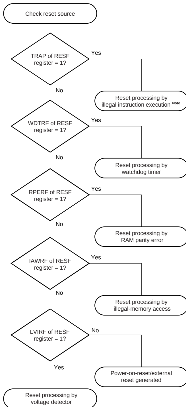
Figure 24-9. Checking reset source
