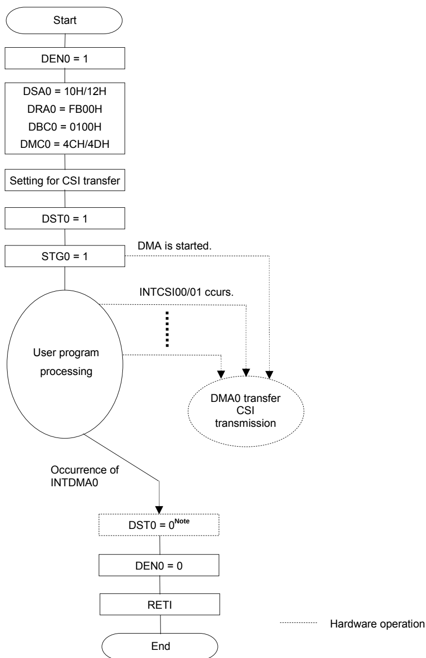
Figure 19-8. Example of Setting for CSI Consecutive Transmission
