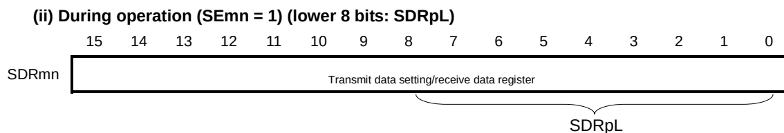
Figure 12-44. Example of Contents of Registers for Master Transmission/Reception of 3-Wire Serial I/O (CSI00, CSI01, CSI10) (2/2)
