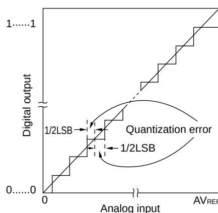
Figure 11-38. Quantization Error
