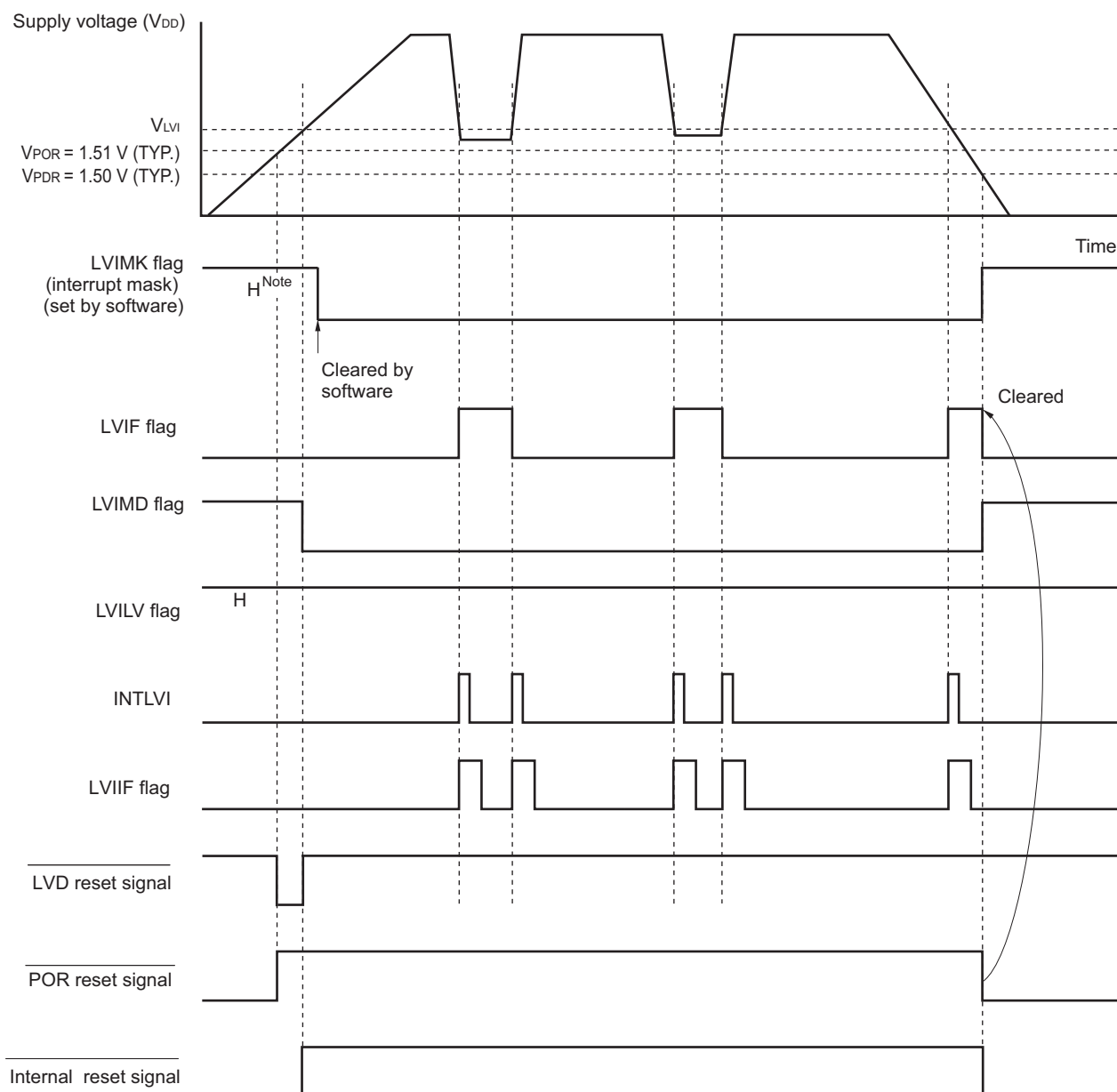
Figure 24-5. Timing of Voltage Detector Internal Interrupt Signal Generation (Option Byte LVIMDS1, LVIMDS0 = 0, 1)
