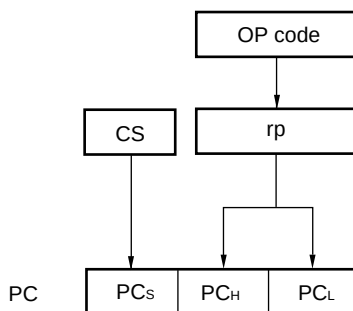
Figure 3-23. Outline of Register Direct Addressing
