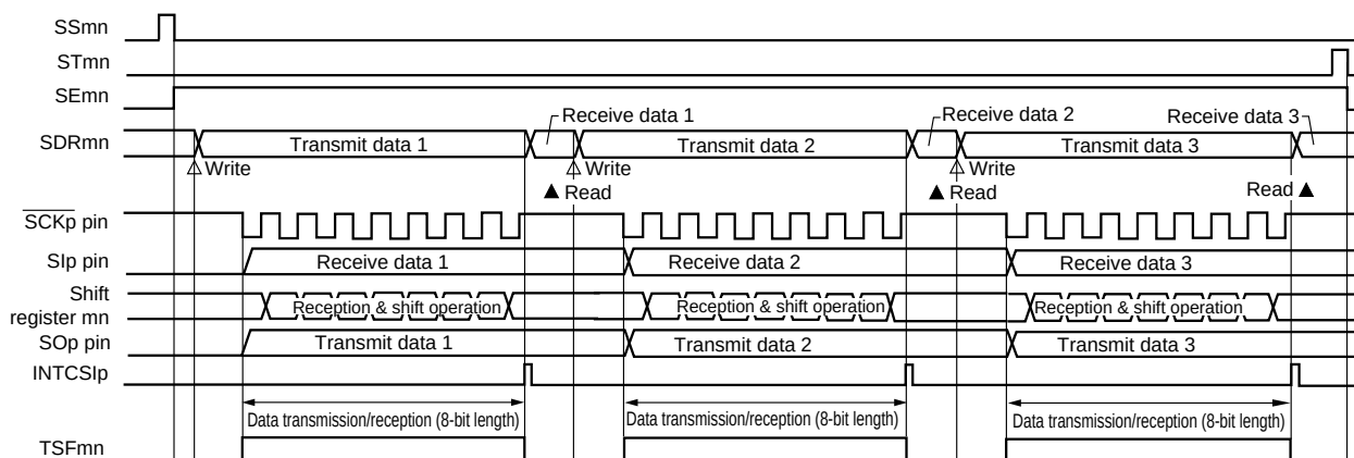
Figure 12-70. Timing Chart of Slave Transmission/Reception (in Single-Transmission/Reception Mode) (Type 1: DAPmn = 0, CKPmn = 0)
