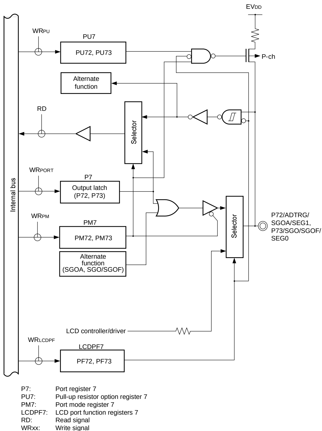
Figure 4-30. Block Diagram of P72, P73
