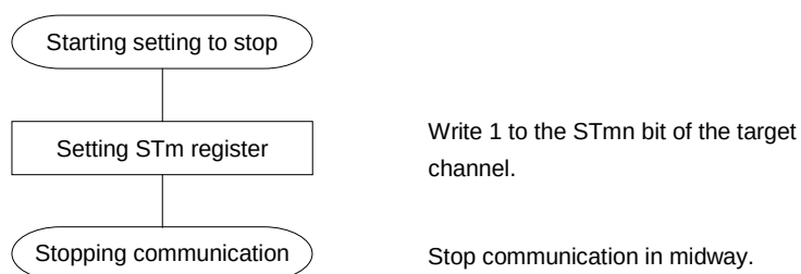
Figure 12-62. Procedure for Stopping Slave Reception
