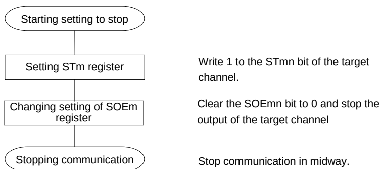
Figure 12-30. Procedure for Stopping Master Transmission
