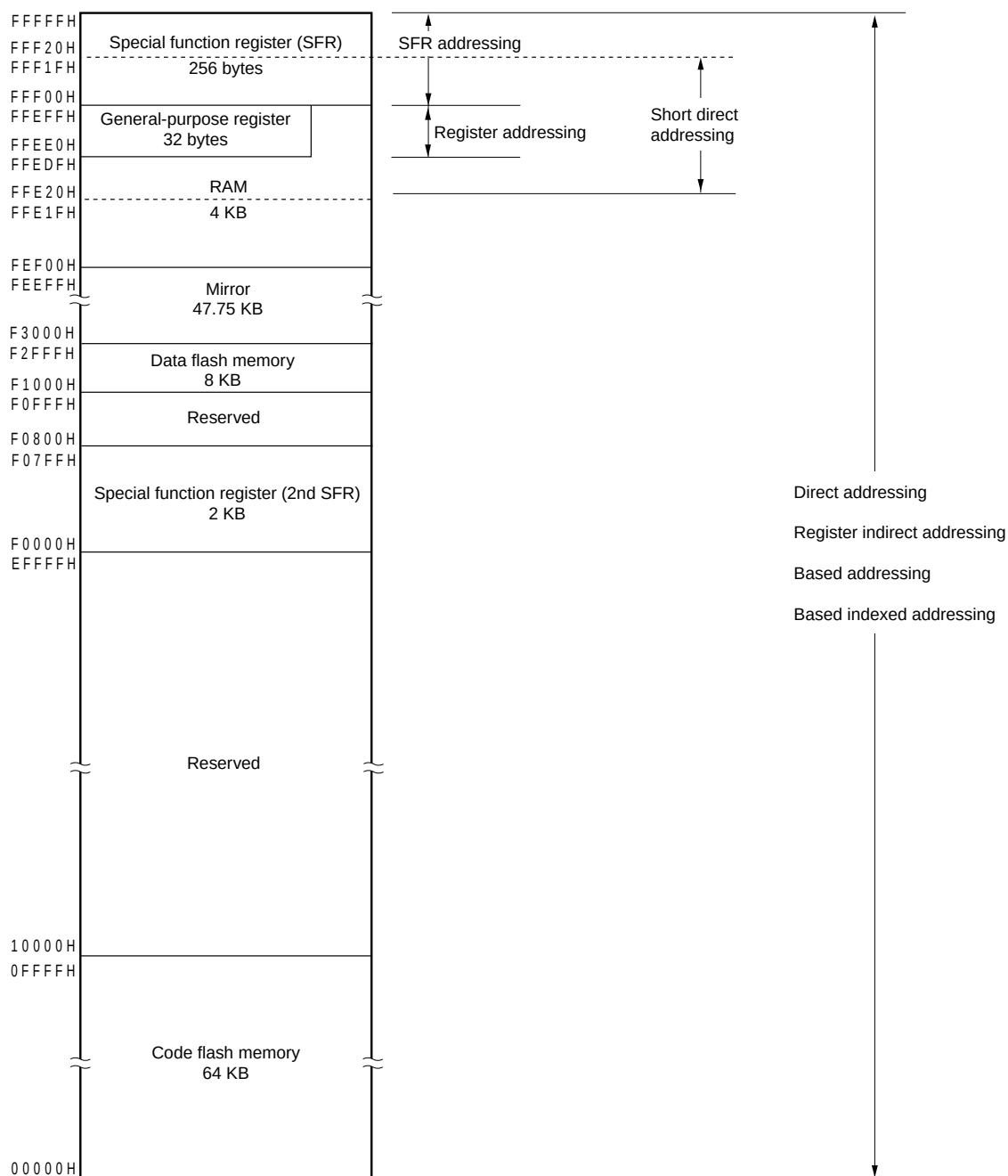
Figure 3-10. Correspondence Between Data Memory and Addressing (R5F10DGE, R5F10DLE, R5F10CME, R5F10DME, R5F10DPE)
