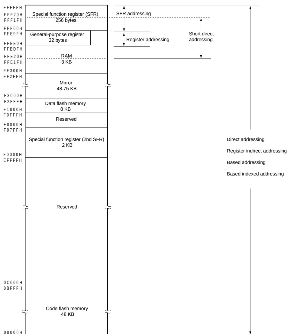
Figure 3-9. Correspondence Between Data Memory and Addressing (R5F10CGD, R5F10DGD, R5F10CLD, R5F10DLD, R5F10CMD, R5F10DMD)
