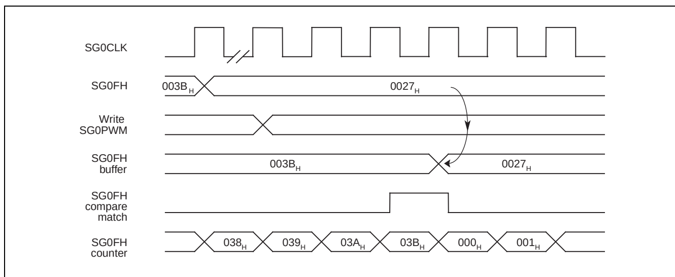
Figure 17-5. Update Timing of the Frequency Buffers
