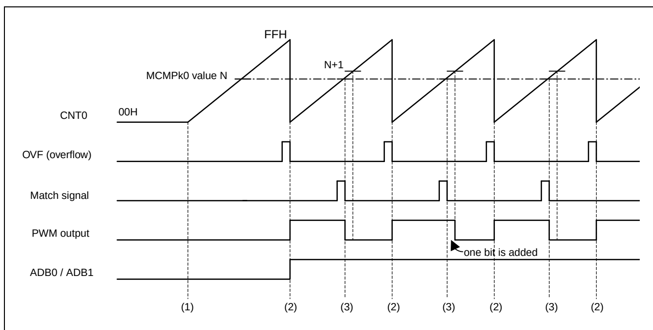
Figure 15-9. Output Timing with 1-bit Addition
