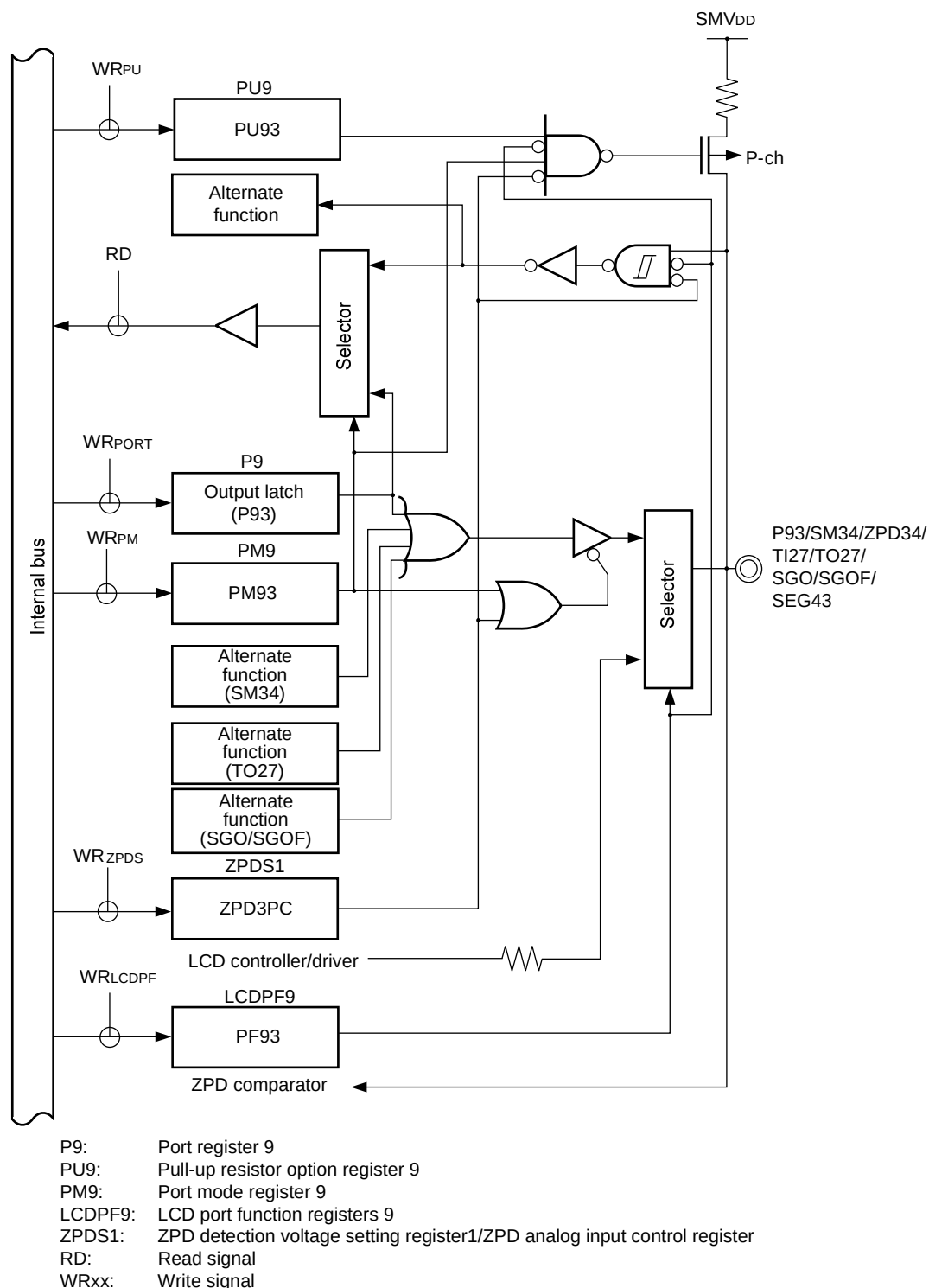
Figure 4-37. Block Diagram of P93
