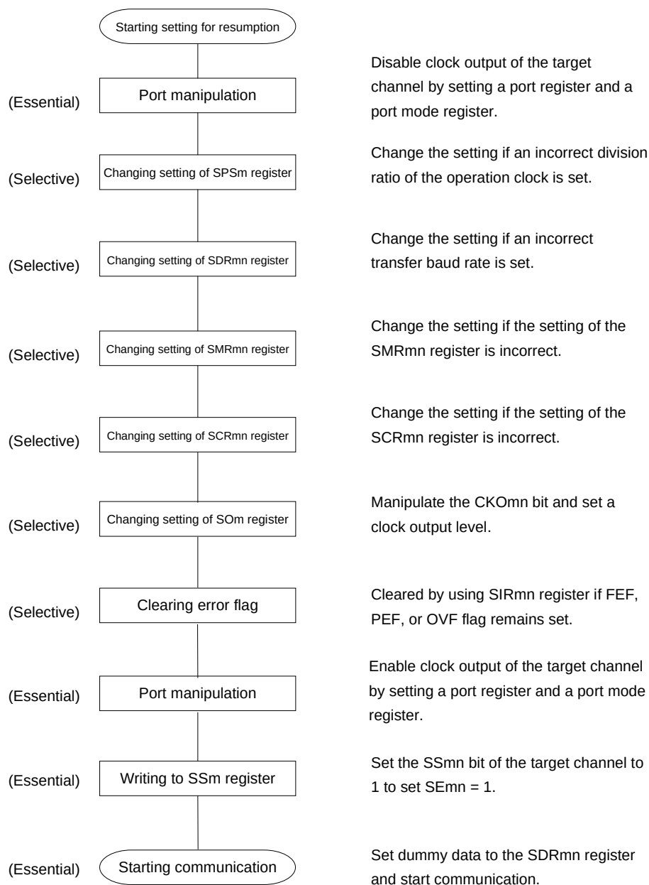
Figure 12-39. Procedure for Resuming Master Reception
