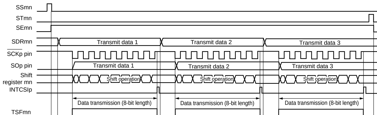
Figure 12-56. Timing Chart of Slave Transmission (in Single-Transmission Mode)
