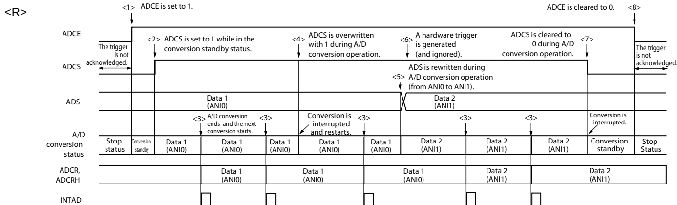
Figure 11-18. Example of Software Trigger Mode (Select Mode, Sequential Conversion Mode) Operation Timing
