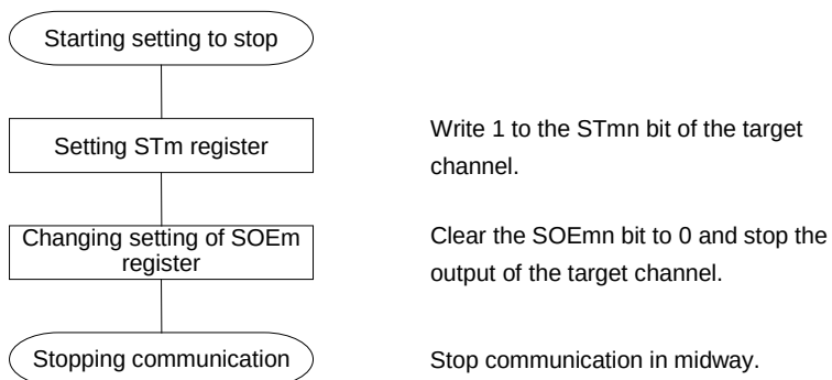
Figure 12-68. Procedure for Stopping Slave Transmission/Reception
