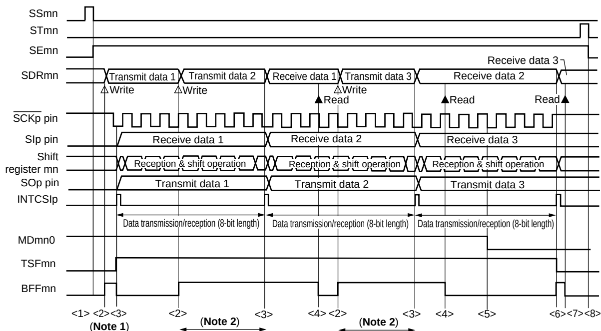
Figure 12-72. Timing Chart of Slave Transmission/Reception (in Continuous Transmission/Reception Mode) (Type 1: DAPmn = 0, CKPmn = 0)
