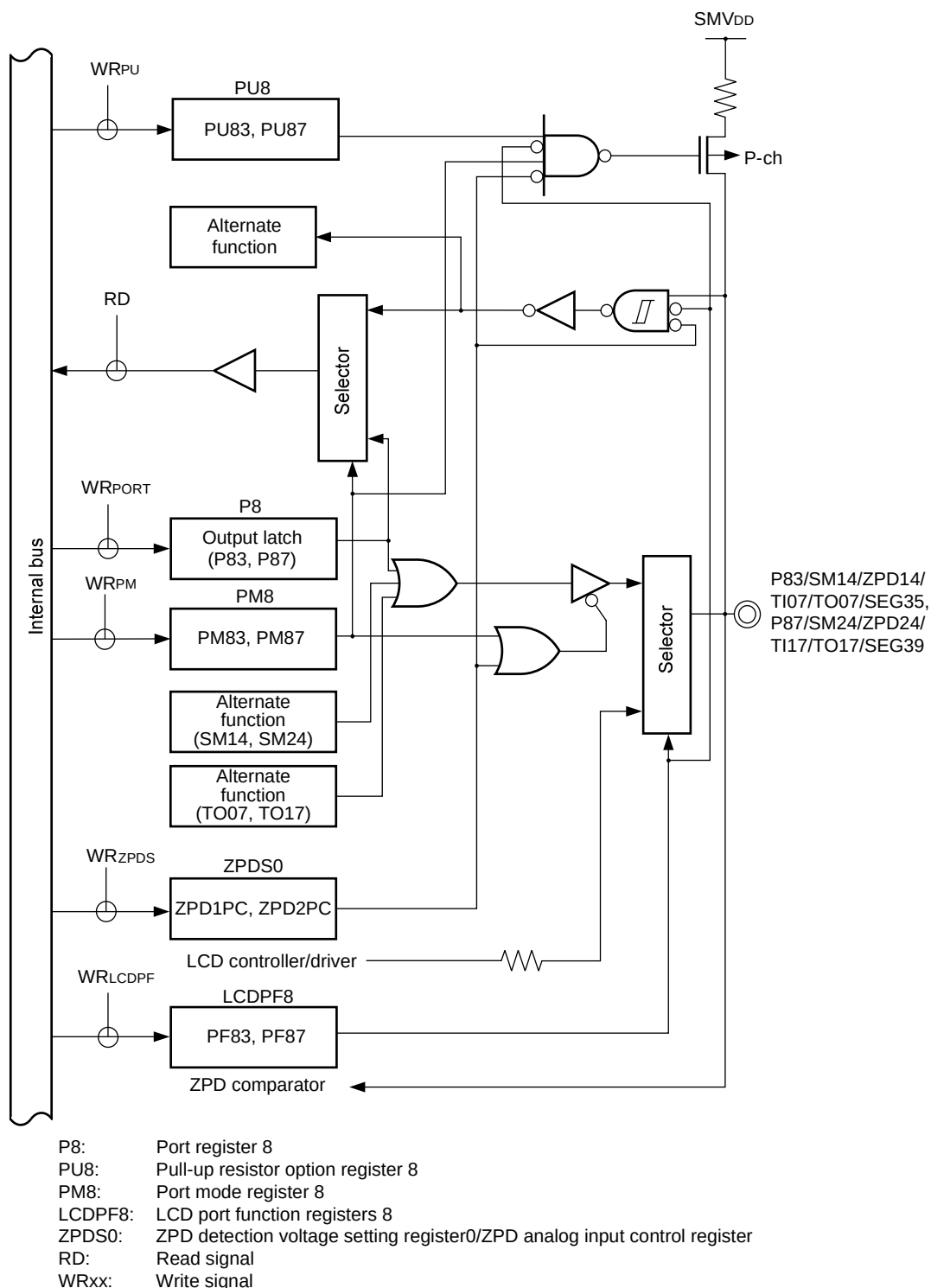
Figure 4-34. Block Diagram of P83, P87
