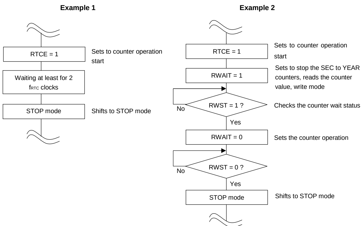
Figure 7-21. Procedure for Shifting to STOP Mode After Setting RTCE bit to 1
