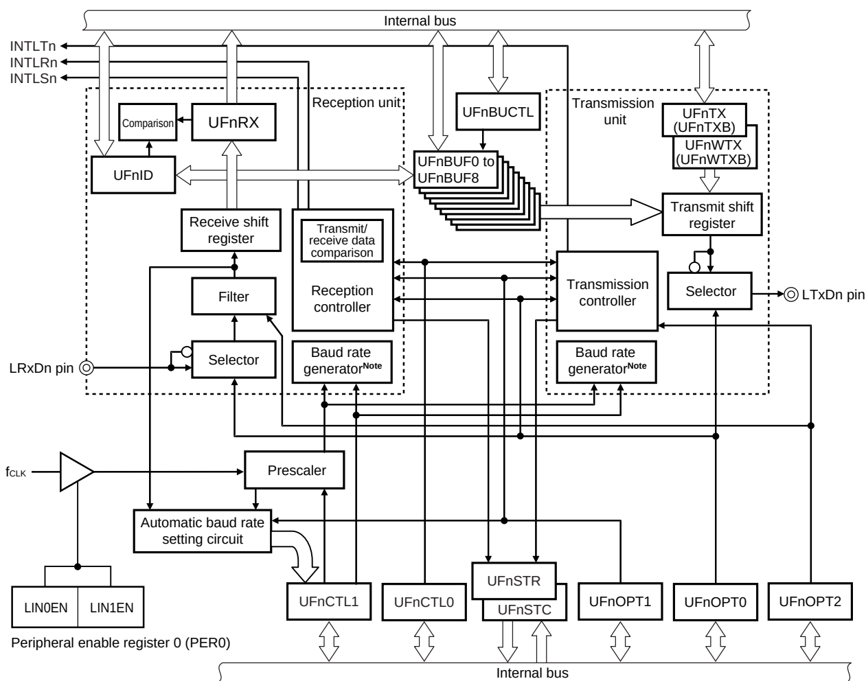
Figure 13-1. Block Diagram of Asynchronous Serial Interface LIN-UART
