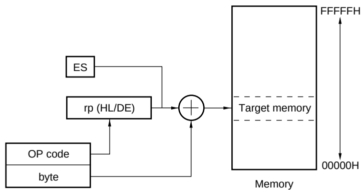
Figure 3-36. Example of ES:[HL + byte], ES:[DE + byte]
