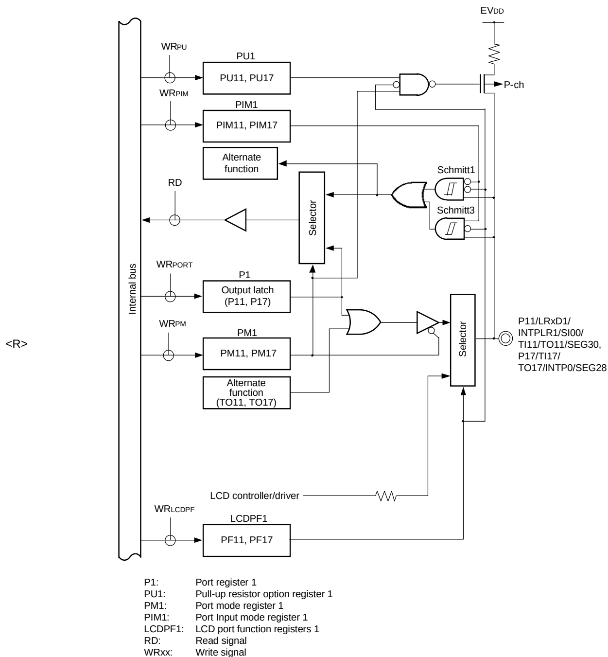
Figure 4-8. Block Diagram of P11, P17
