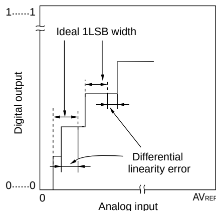
Figure 11-42. Differential Linearity Error
