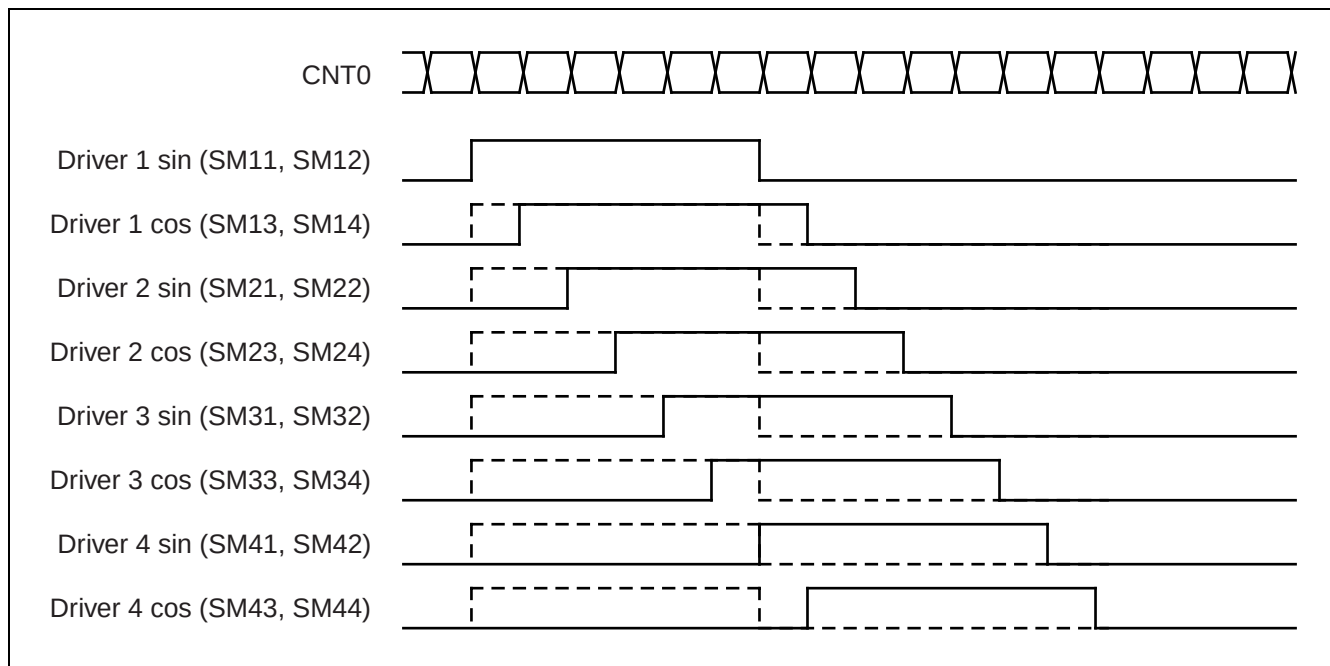
Figure 15-11. Output Timing of Signals SM11 to SM44
