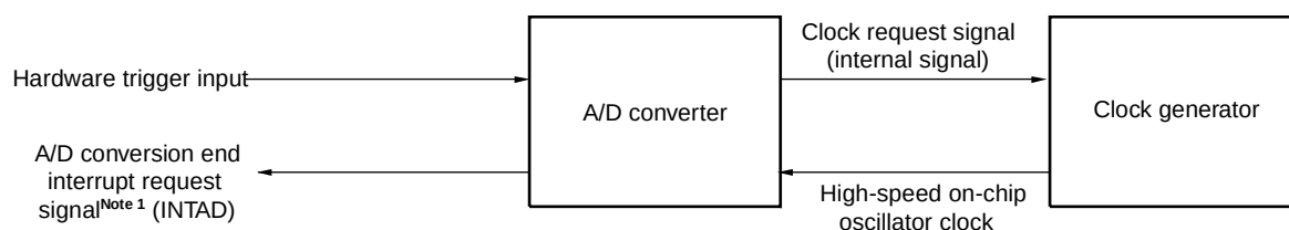
Figure 11-34. Block Diagram When Using SNOOZE Mode Function
