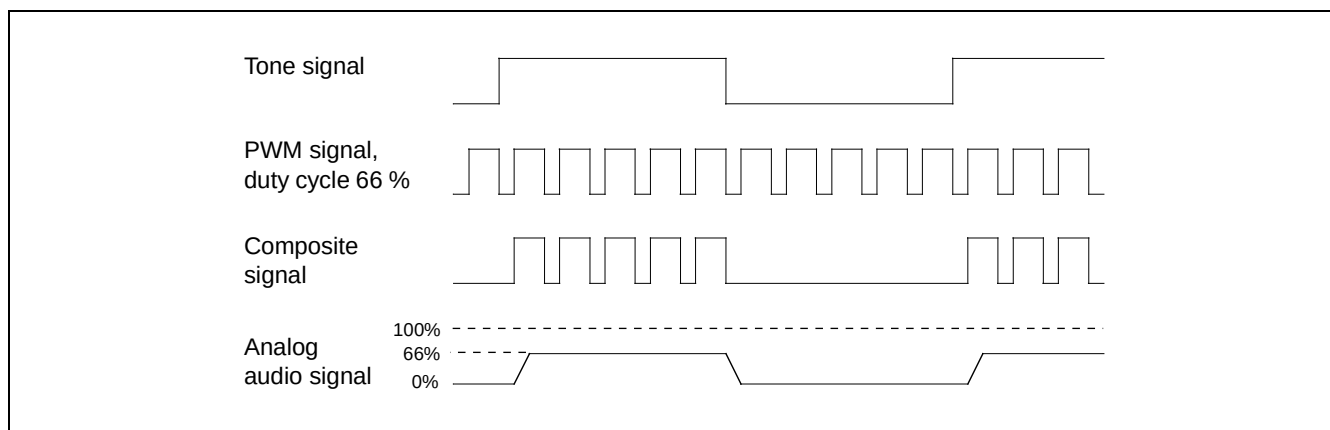
Figure 17-2. Generation of the Composite Output Signal
