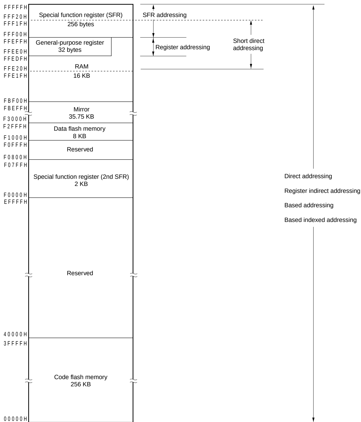
Figure 3-12. Correspondence Between Data Memory and Addressing (R5F10DMJ, R5F10TPJ, R5F10DPJ)
