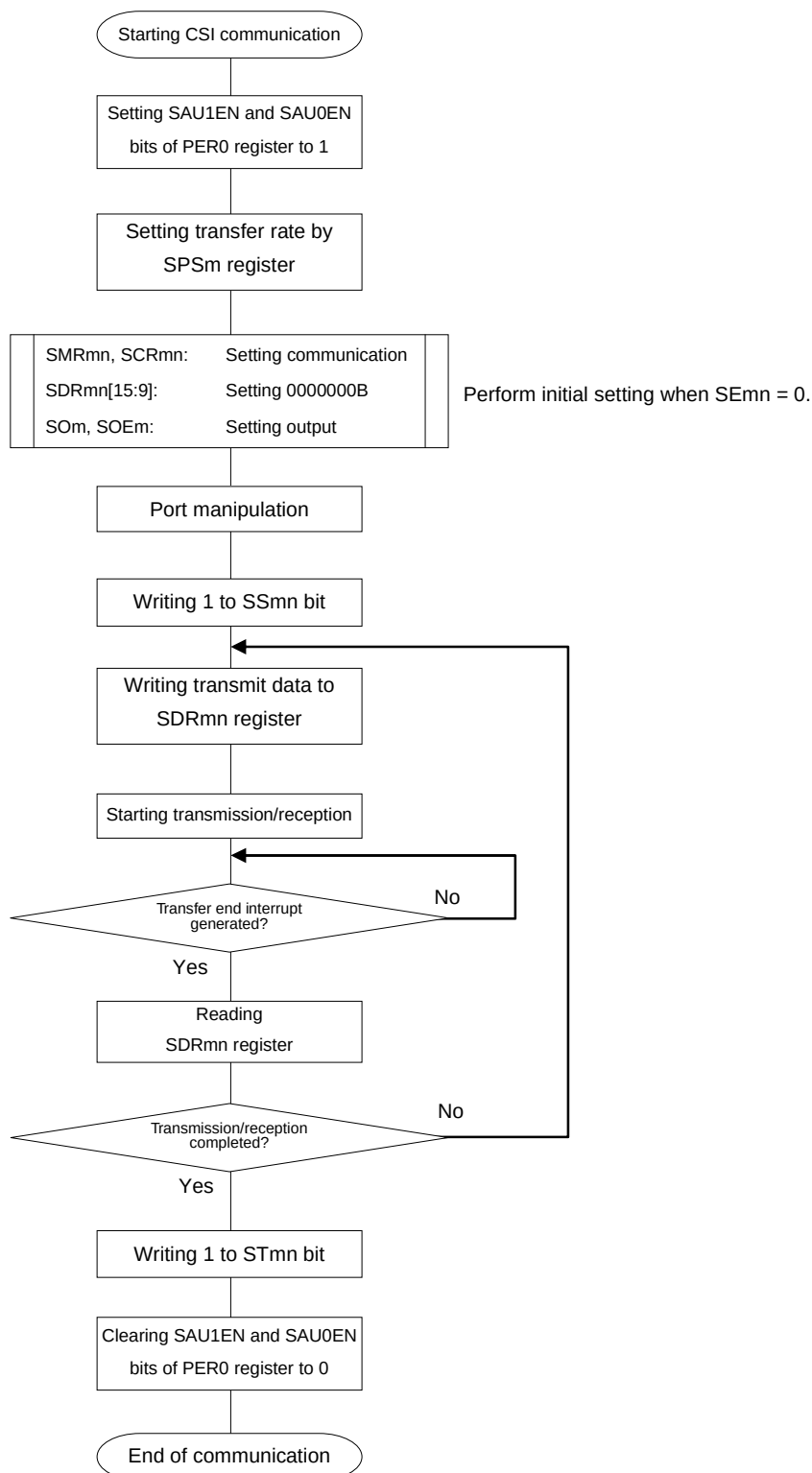
Figure 12-71. Flowchart of Slave Transmission/Reception (in Single- Transmission/Reception Mode)
