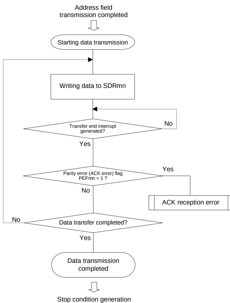
Figure 12-130. Flowchart of Data Transmission
