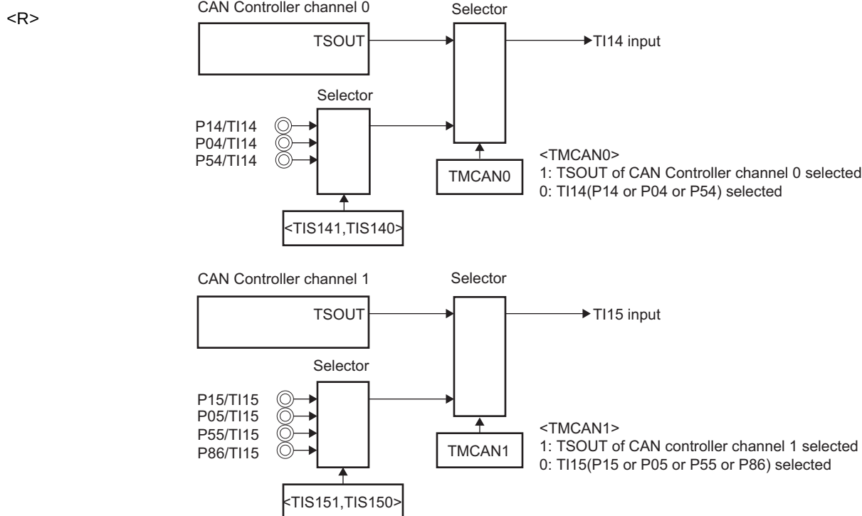
Figure 14-62. Switching source of input
