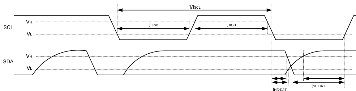
Figure 33-10. Simplified IC mode serial transfer timing
