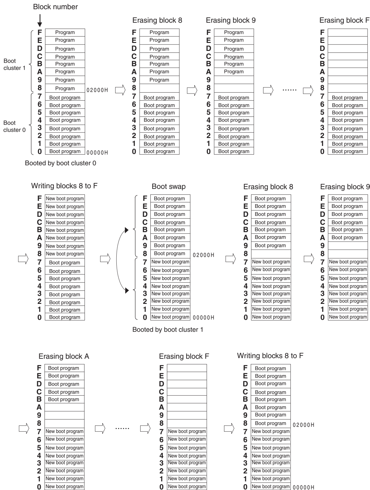
Figure 28-12. Example of Executing Boot Swapping
