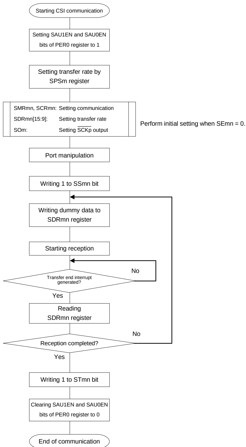
Figure 12-41. Flowchart of Master Reception (in Single-Reception Mode)
