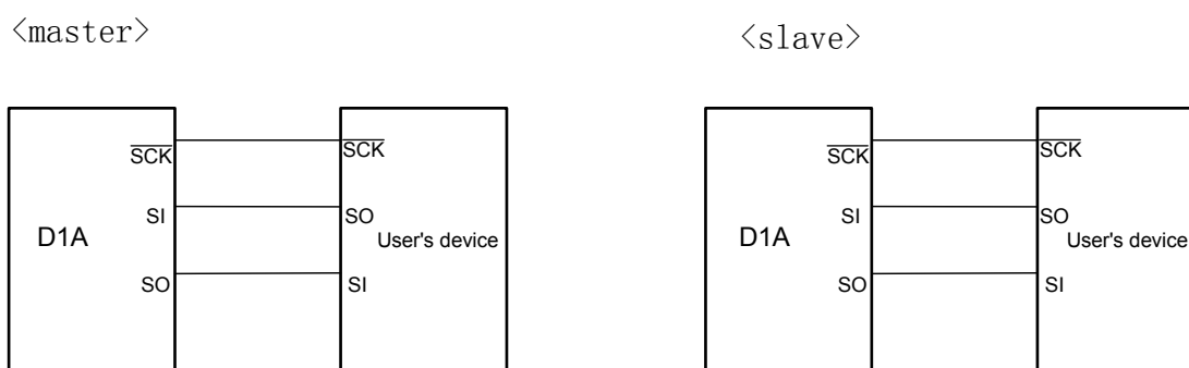
Figure 32-6. CSI mode connection diagram
