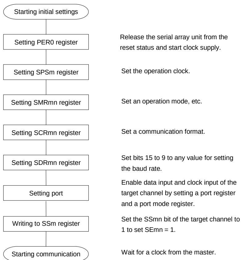
Figure 12-61. Initial Setting Procedure for Slave Reception
