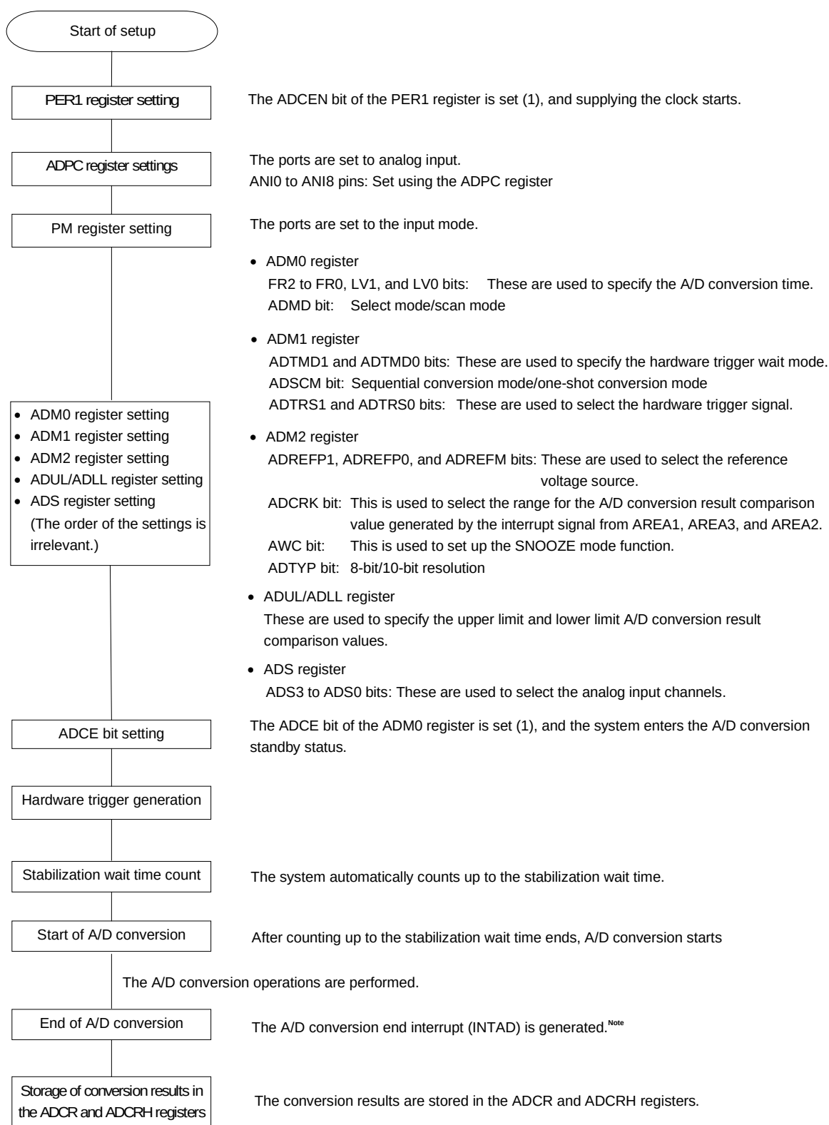
Figure 11-32. Setting up Hardware Trigger Wait Mode
