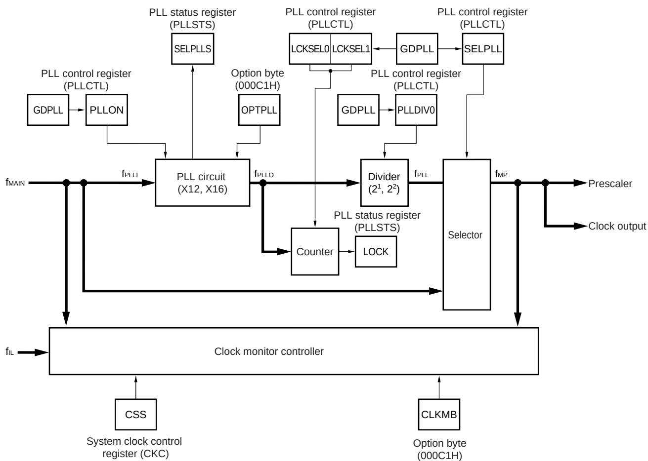
Figure 5-2. Block Diagram of PLL Circuit
