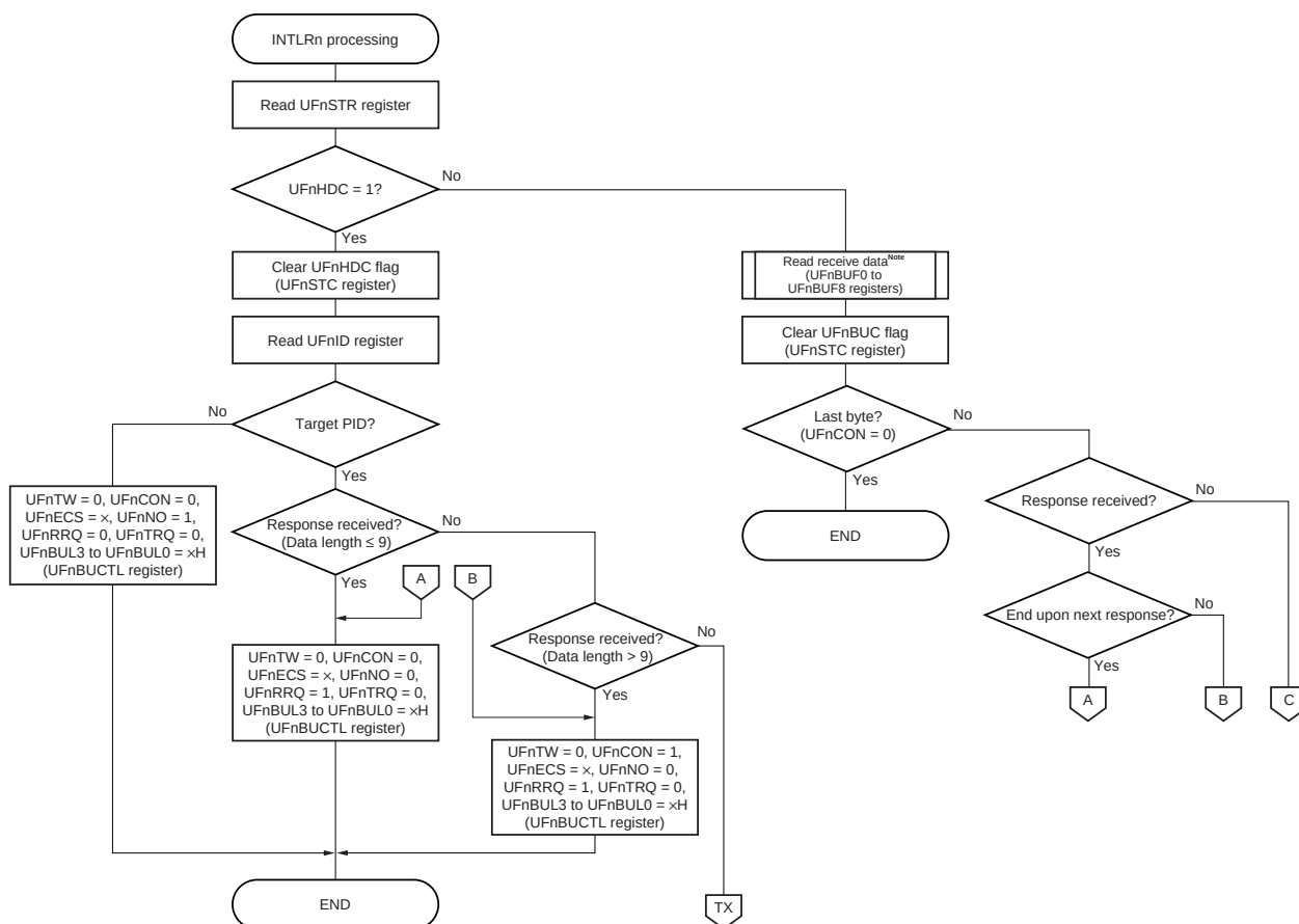
Figure 13-64. Multi-Byte Transmission/Reception Processing Flow Example (1/2)
