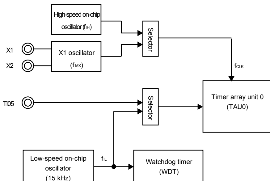
Figure 25-13. Configuration of Frequency Detection Function
