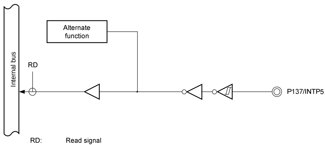
Figure 4-48. Block Diagram of P137
