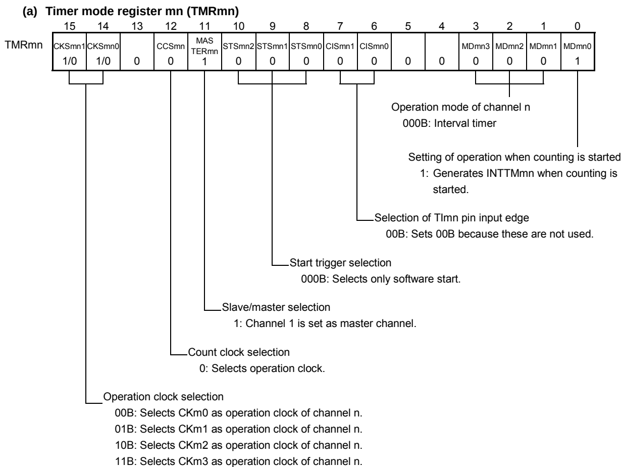
Figure 6-73. Example of Set Contents of Registers When PWM Function (Master Channel) Is Used (1/2)
