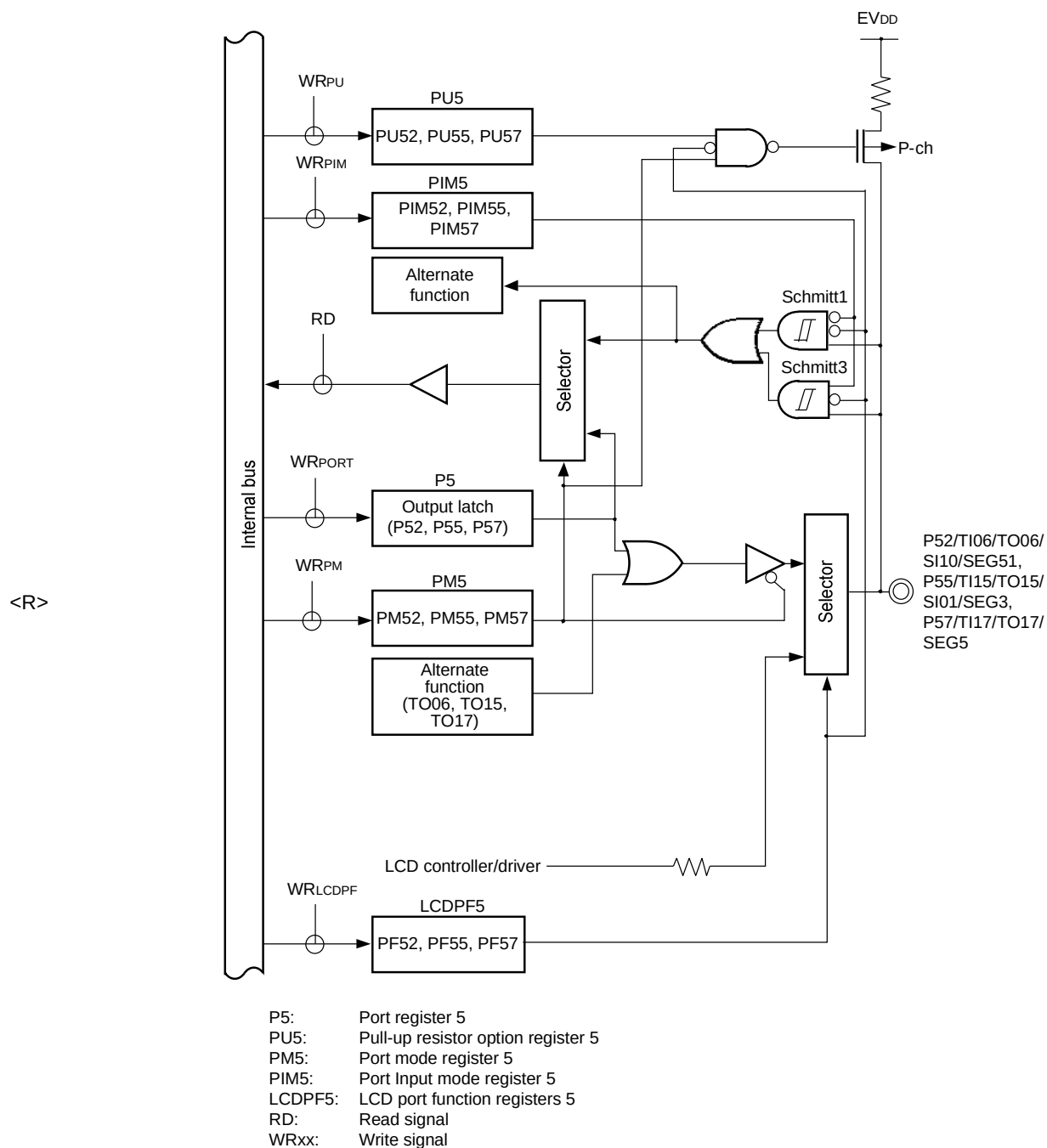
Figure 4-20. Block Diagram of P52, P55, P57
