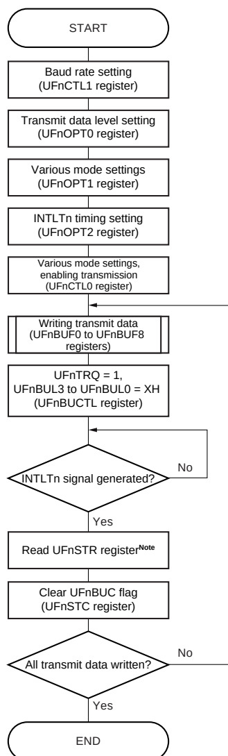
Figure 13-49. UART Buffer Mode Transmission Processing Flow
