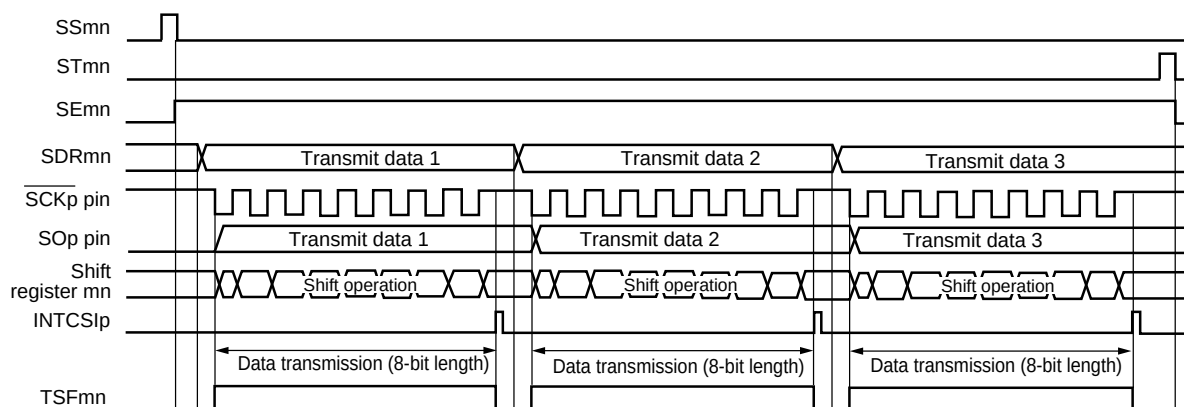
Figure 12-32. Timing Chart of Master Transmission (in Single-Transmission Mode) (Type 1: DAPmn = 0, CKPmn = 0)
