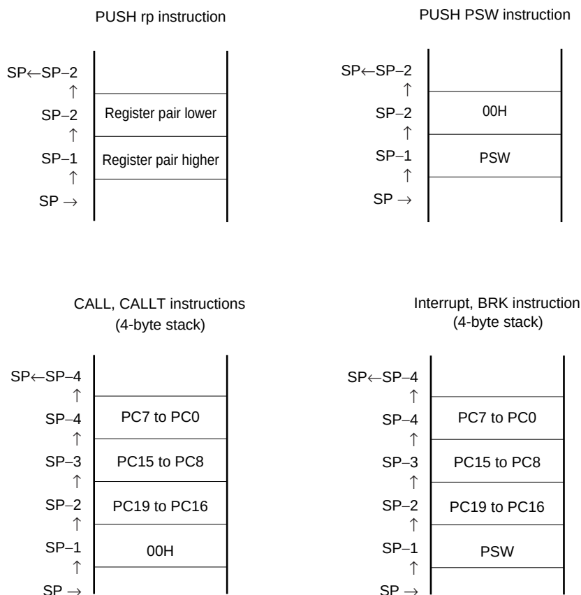
Figure 3-16. Data to Be Saved to Stack Memory
