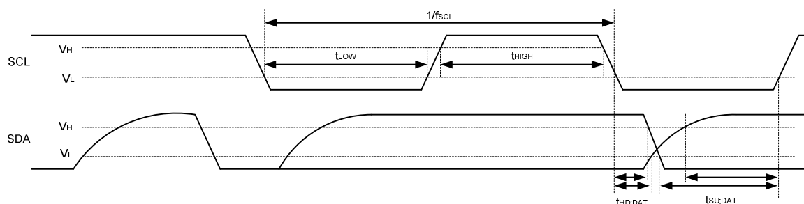
Figure 32-10. Simplified I 2 C mode serial transfer timing
