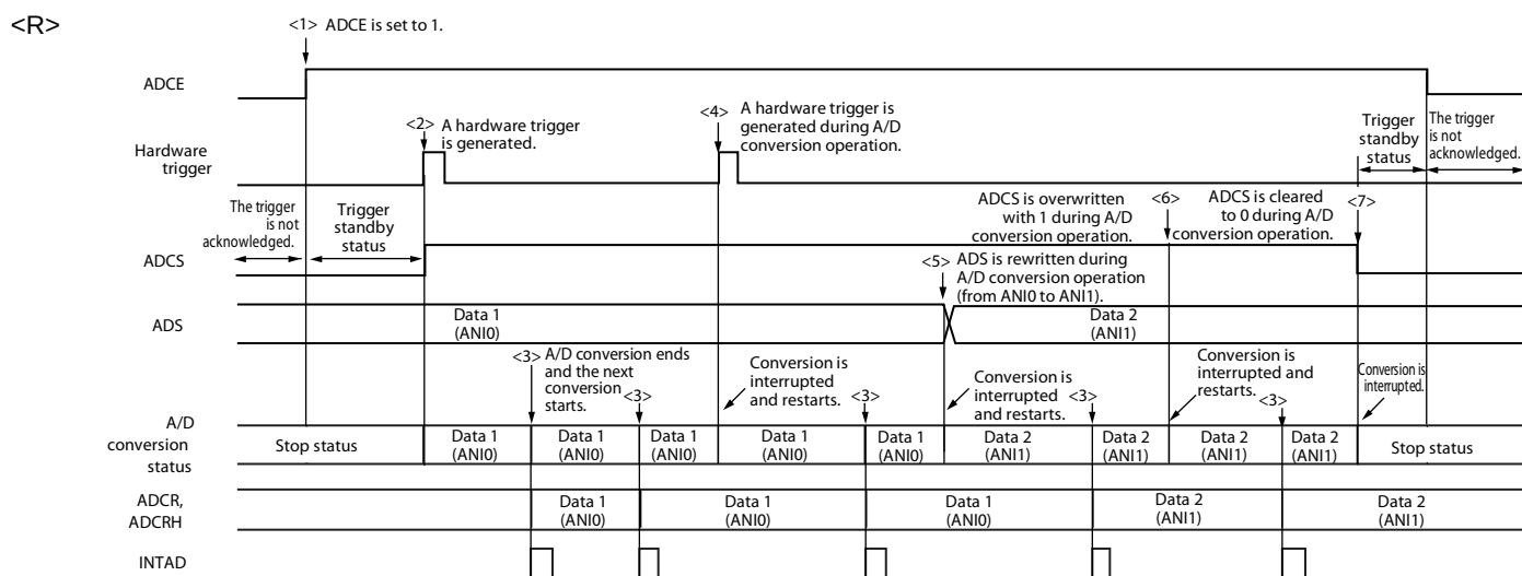
Figure 11-26. Example of Hardware Trigger Wait Mode (Select Mode, Sequential Conversion Mode) Operation Timing
