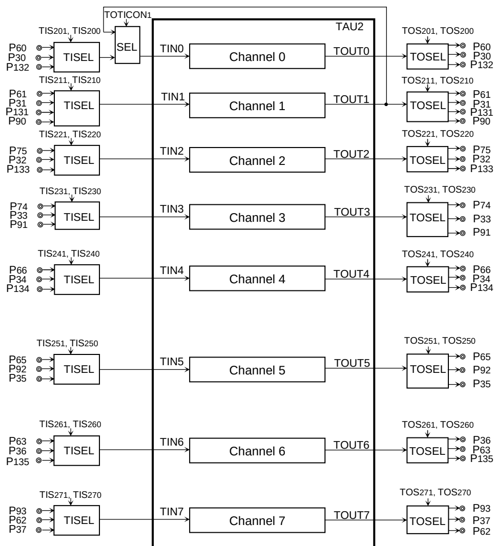
Figure 4-59. Timer Array unit and RTC I/O connection (3/3)
