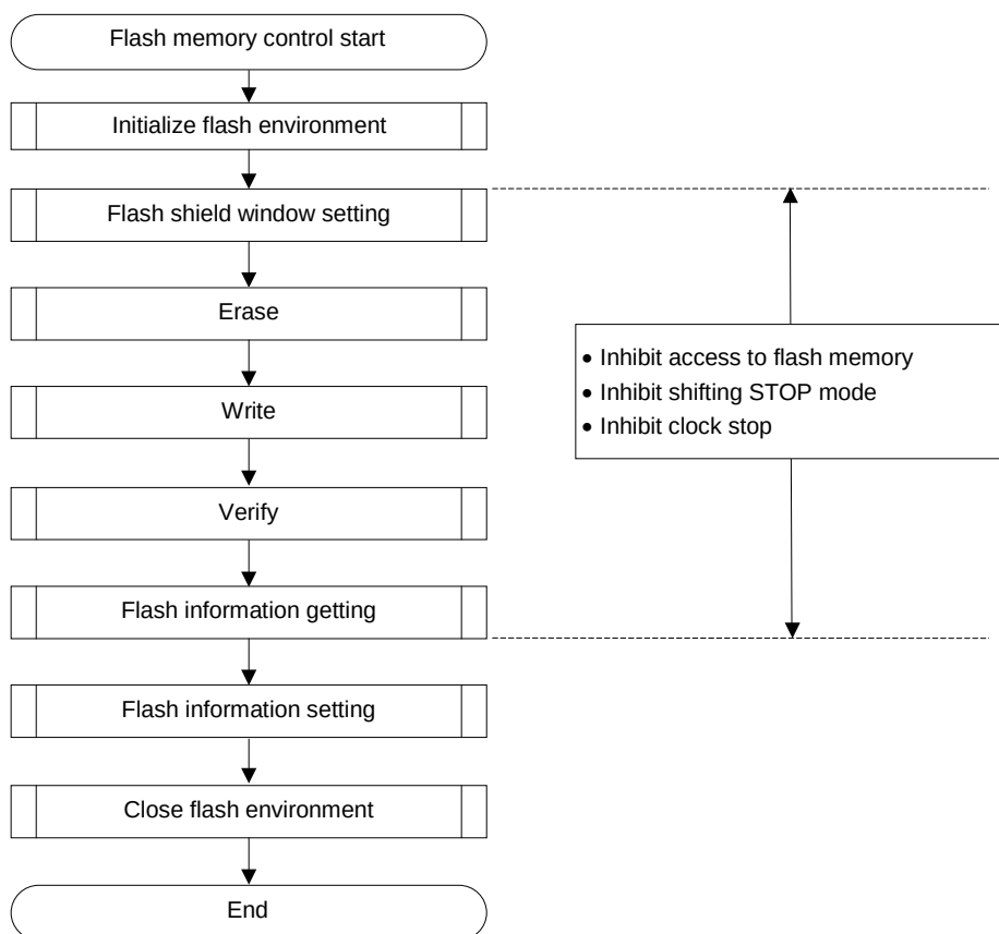
Figure 28-10. Flow of Self Programming (Rewriting Flash Memory)
