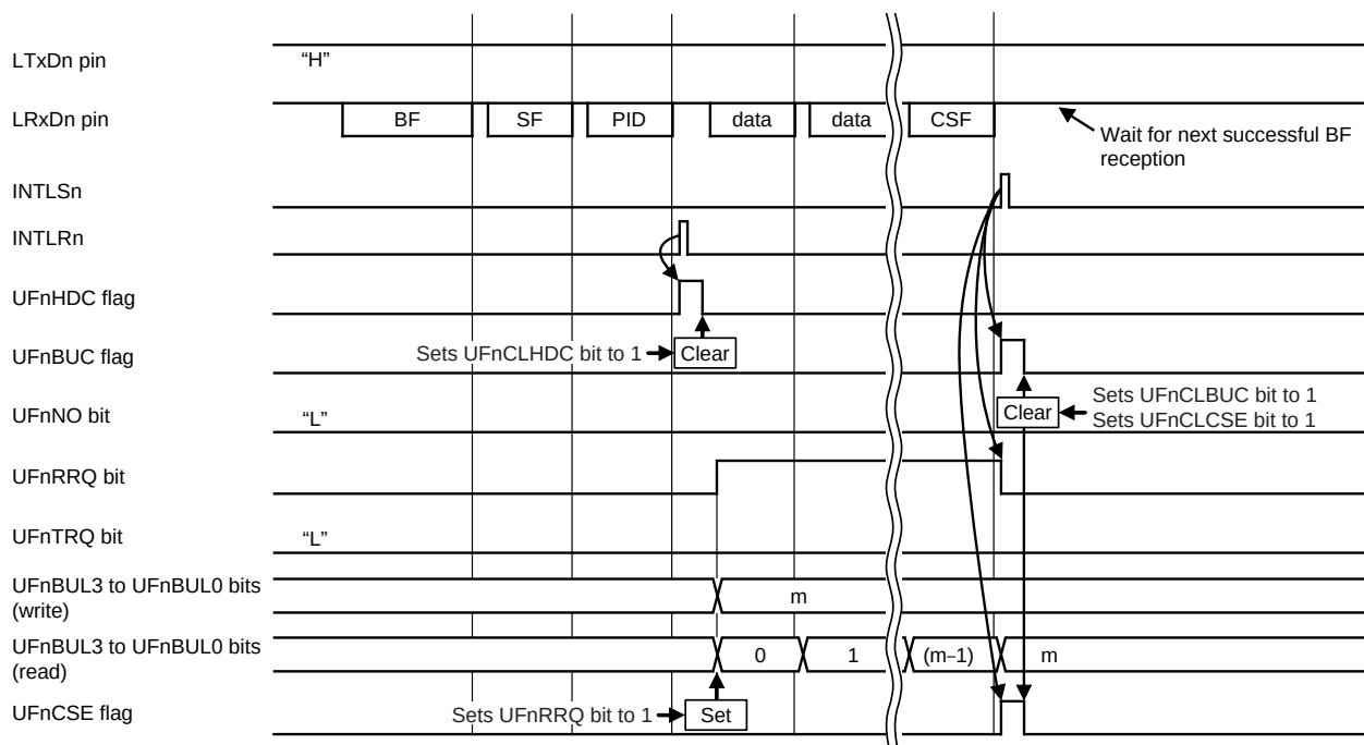
Figure 13-63. Automatic Checksum Error Occurrence Example (Response Reception)
