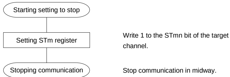
Figure 12-38. Procedure for Stopping Master Reception
