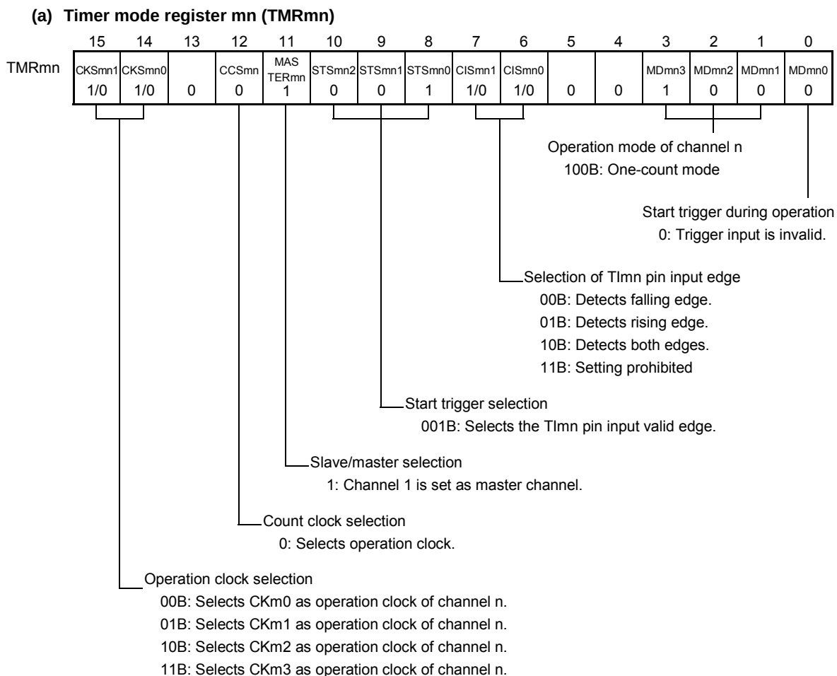
Figure 6-78. Example of Set Contents of Registers When One-Shot Pulse Output Function Is Used (Master Channel) (1/2)
