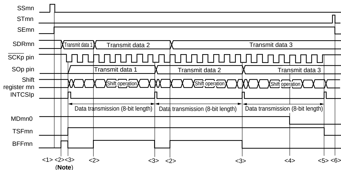
Figure 12-58. Timing Chart of Slave Transmission (in Continuous Transmission Mode)
