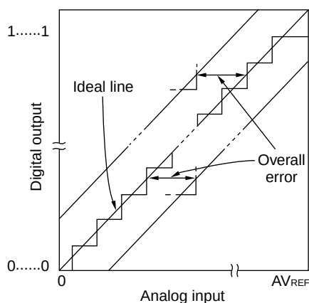
Figure 11-37. Overall Error
