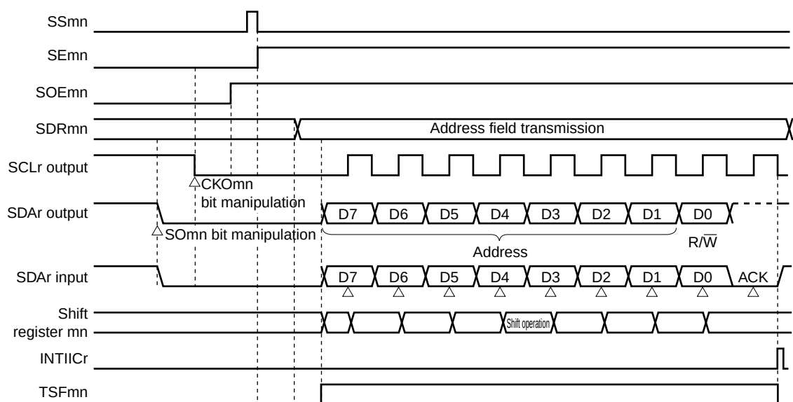
Figure 12-126. Timing Chart of Address Field Transmission
