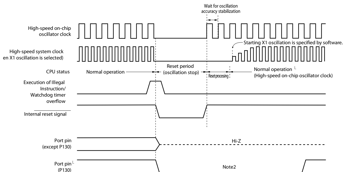
Figure 22-3. Timing of Reset Due to Execution of Illegal Instruction or Watchdog Timer Overflow
