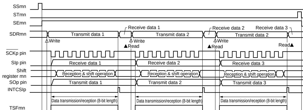
Figure 12-48. Timing Chart of Master Transmission/Reception (in Single-Transmission/Reception Mode) (Type 1: DAPmn = 0, CKPmn = 0)
