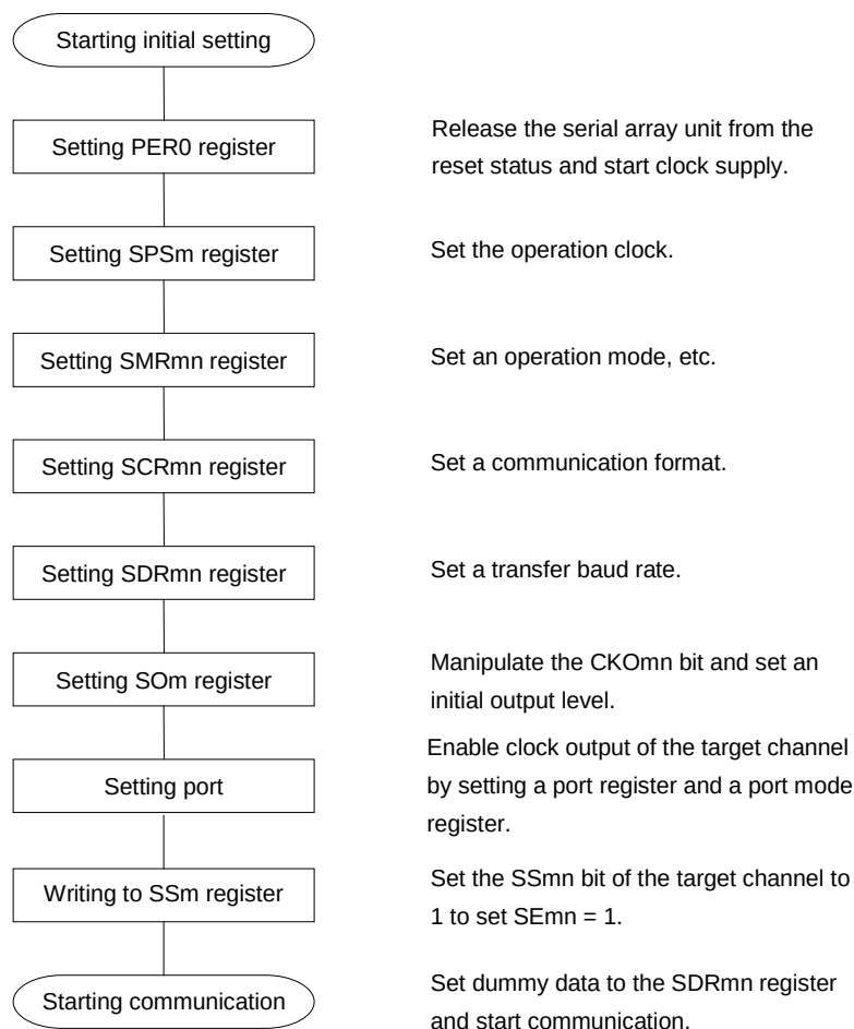
Figure 12-37. Initial Setting Procedure for Master Reception
