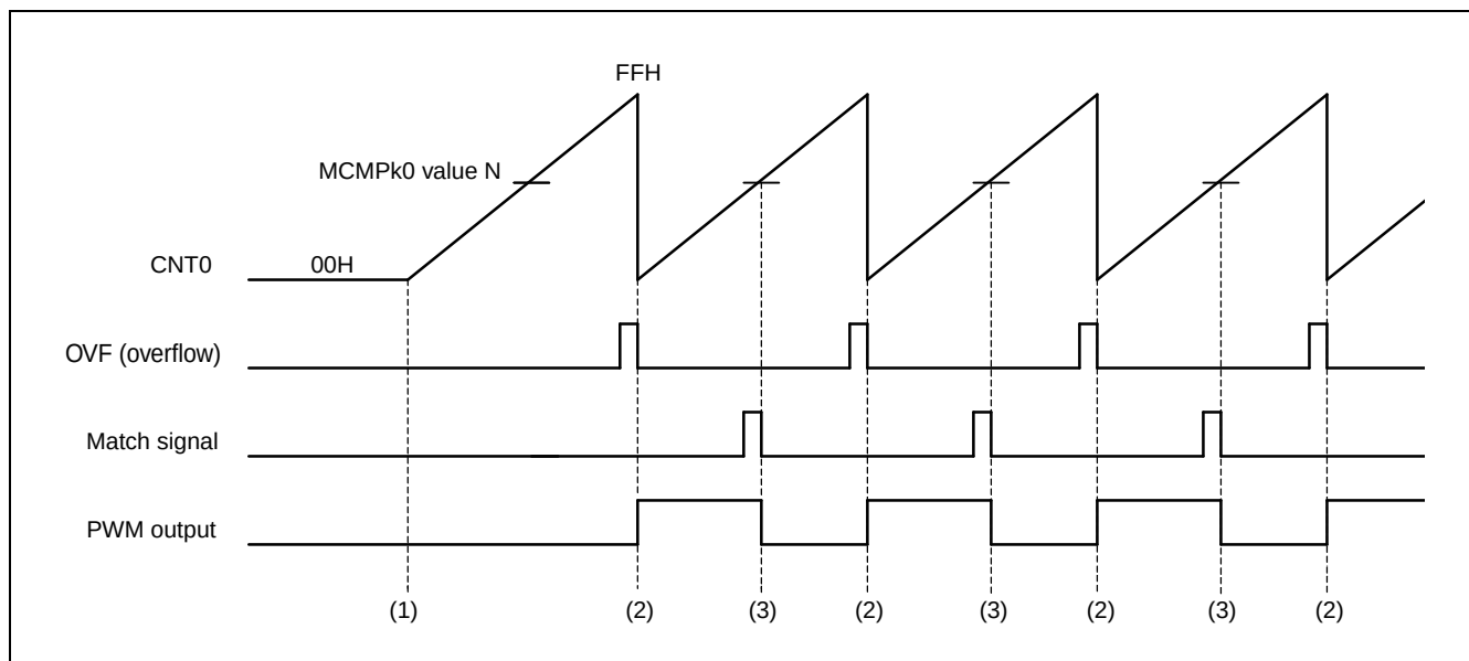
Figure 15-9. Output Timing with 1-bit Addition
