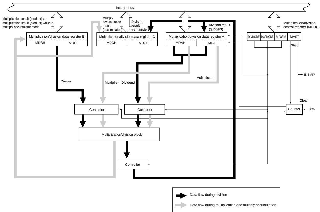
Figure 18-1. Block Diagram of Multiplier and Divider/Multiply-Accumulator
