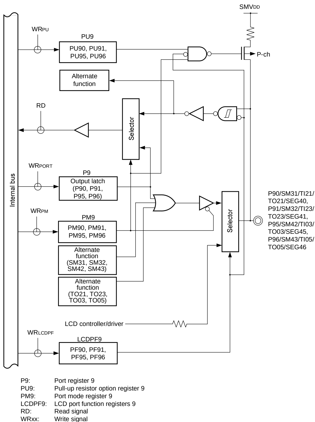
Figure 4-35. Block Diagram of P90, P91, P95, and P96
