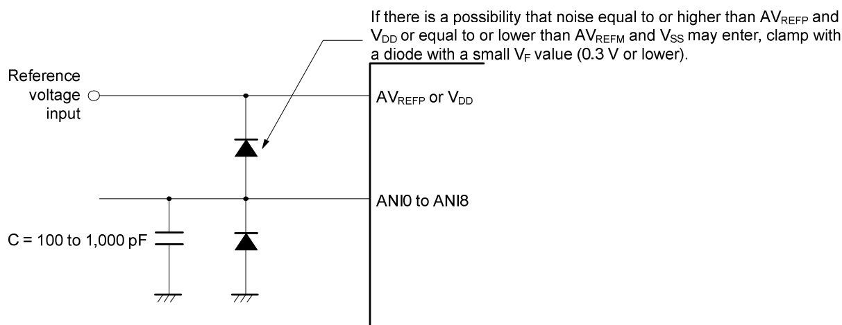
Figure 11-43. Analog Input Pin Connection
