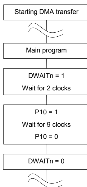
Figure 19-11. Example of Setting for Holding DMA Transfer Pending by DWAITn Bit
