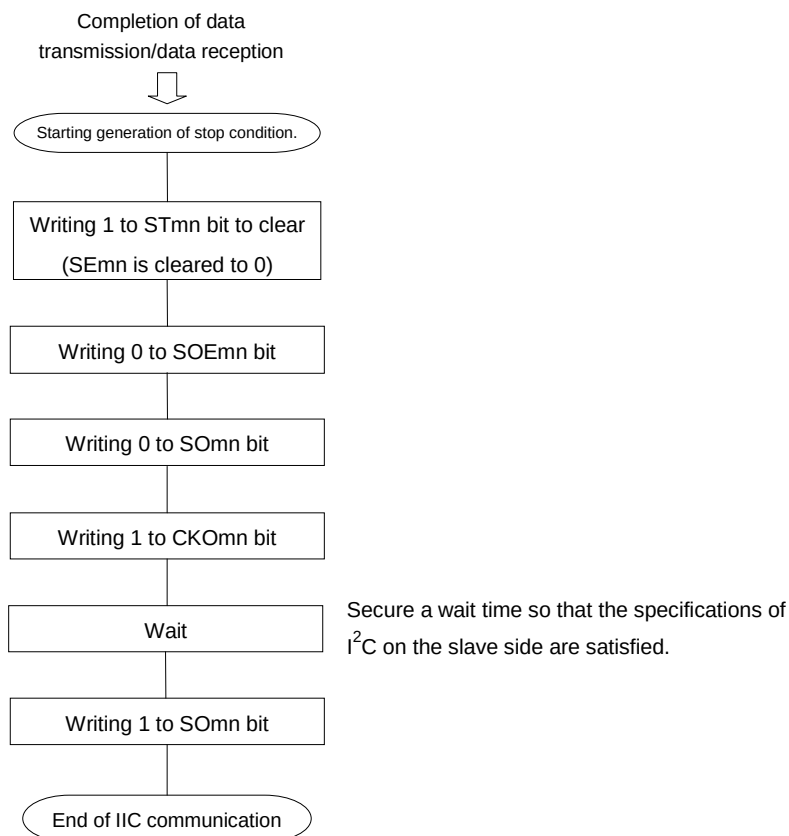
Figure 12-135. Flowchart of Stop Condition Generation
