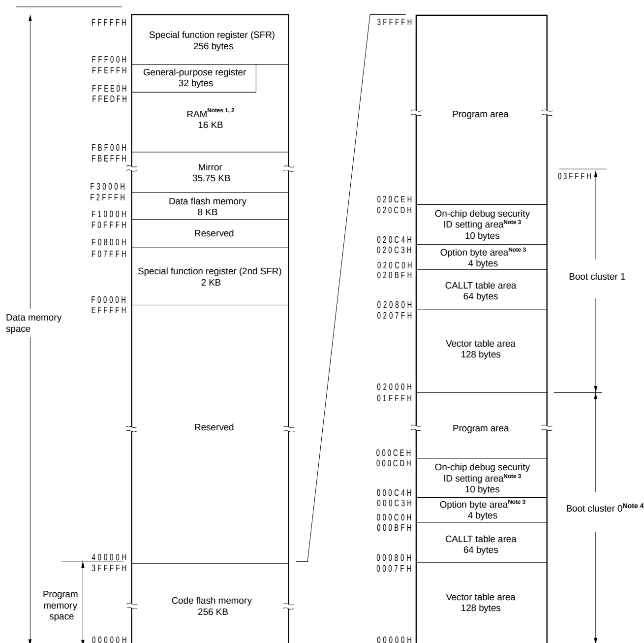
Figure 3-7. Memory Map (R5F10DMJxFB, R5F10TPJxFB, R5F10DPJxFB)
