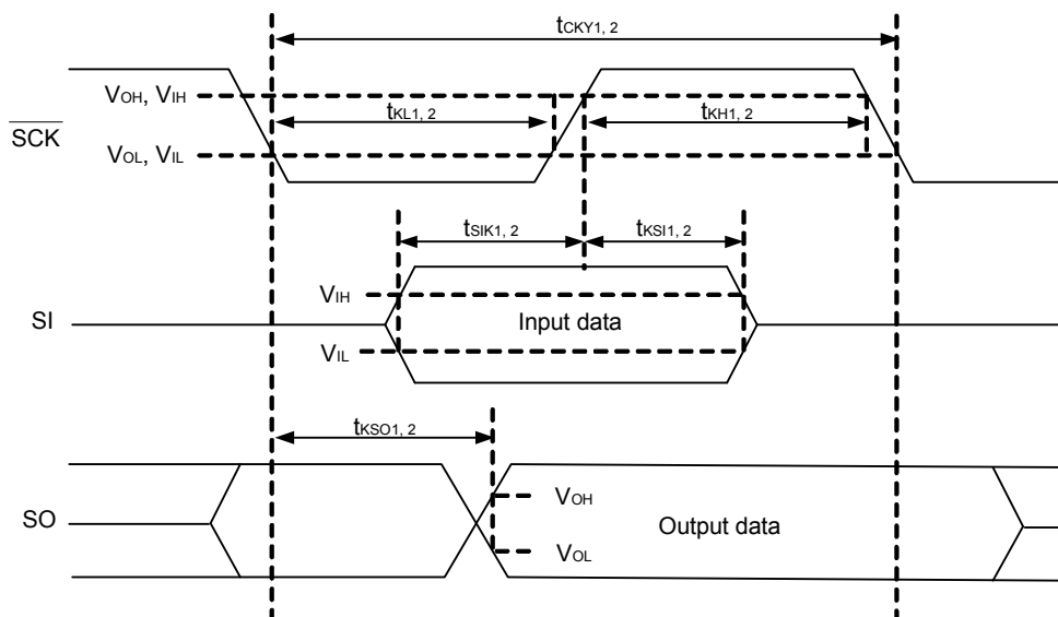
Figure 32-7. CSI mode serial transfer timing (When DAPmn = 0 and CKPmn = 0, or DAPmn = 1 and CKPmn = 1.)
