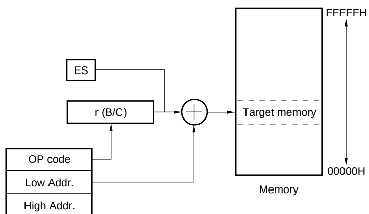
Figure 3-37. Example of ES:word[B], ES:word[C]
