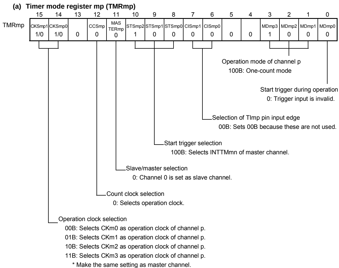
Figure 6-79. Example of Set Contents of Registers When One-Shot Pulse Output Function Is Used (Slave Channel) (1/2)
