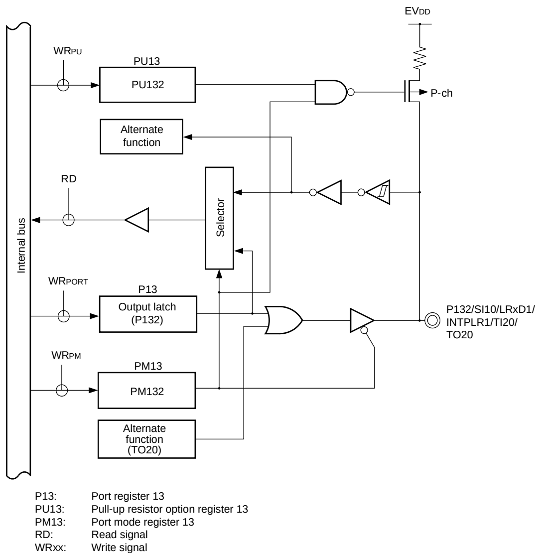
Figure 4-43. Block Diagram of P132
