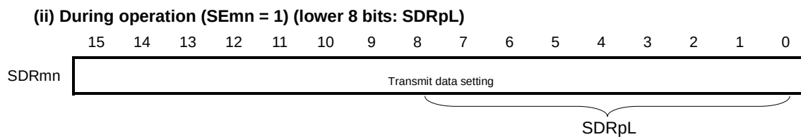
Figure 12-52. Example of Contents of Registers for Slave Transmission of 3-Wire Serial I/O (CSI00, CSI01, CSI10) (2/2)
