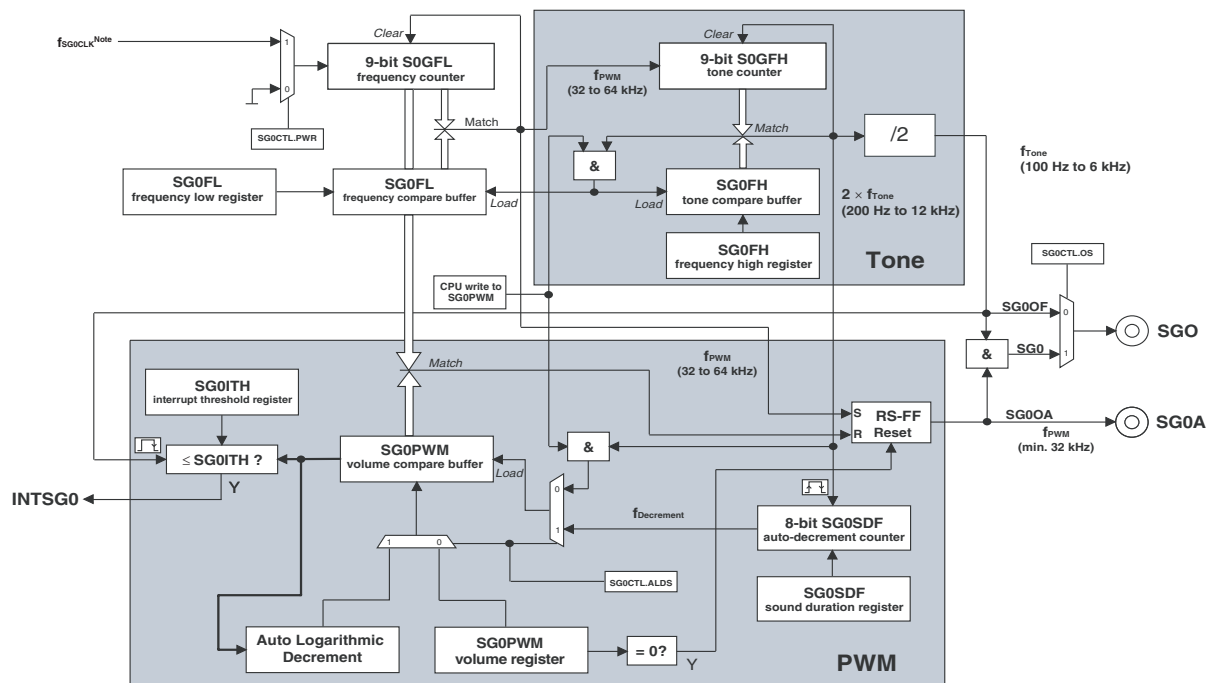
Figure 17-1. Sound Generator Block Diagram
