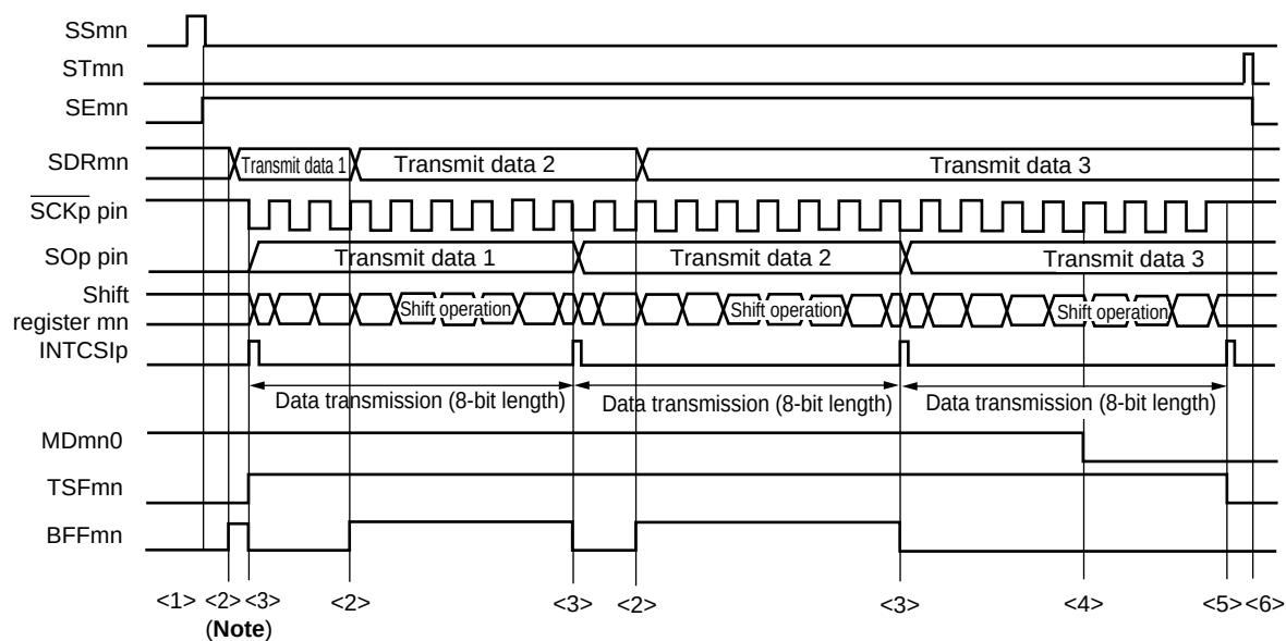
Figure 12-34. Timing Chart of Master Transmission (in Continuous Transmission Mode) (Type 1: DAPmn = 0, CKPmn = 0)
