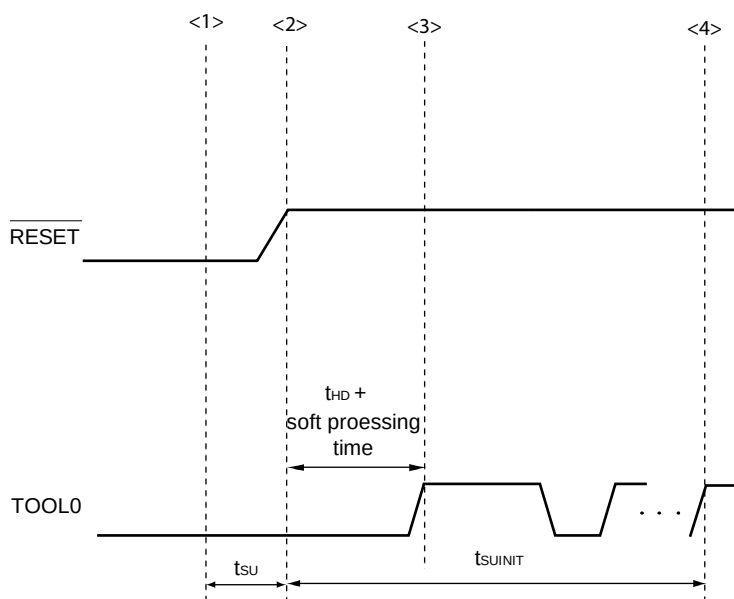
Figure 28-8. Setting of Flash Memory Programming Mode
