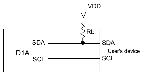
Figure 33-9. simplified IIC connection diagram
