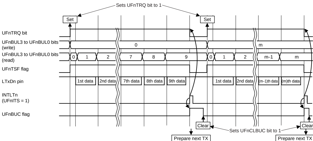
Figure 13-51. UART Buffer Mode Transmission Example (UFnITS = 1)
