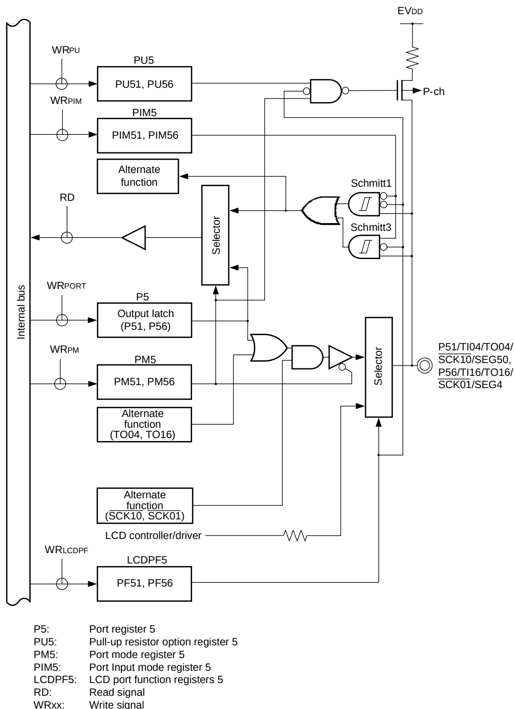
Figure 4-19. Block Diagram of P51, P56
