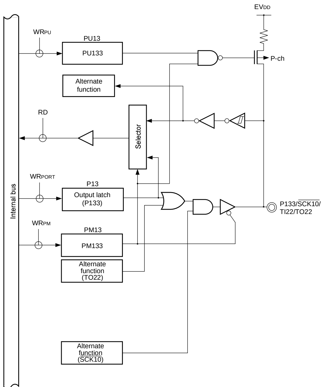
Figure 4-44. Block Diagram of P133
