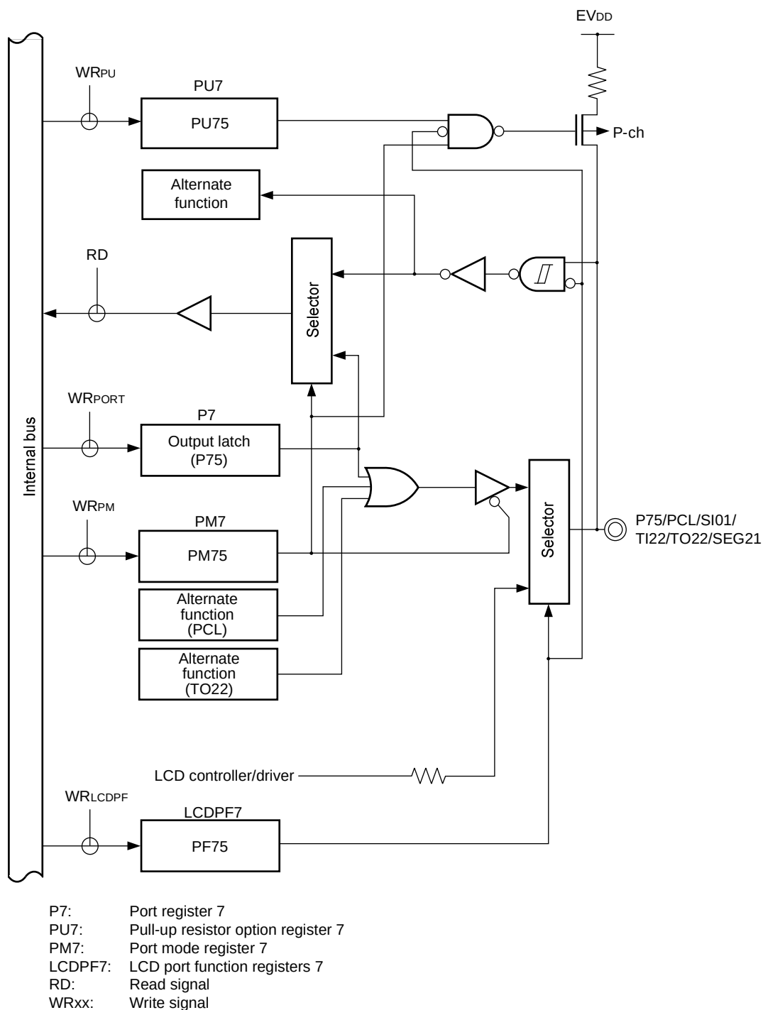
Figure 4-32. Block Diagram of P75
