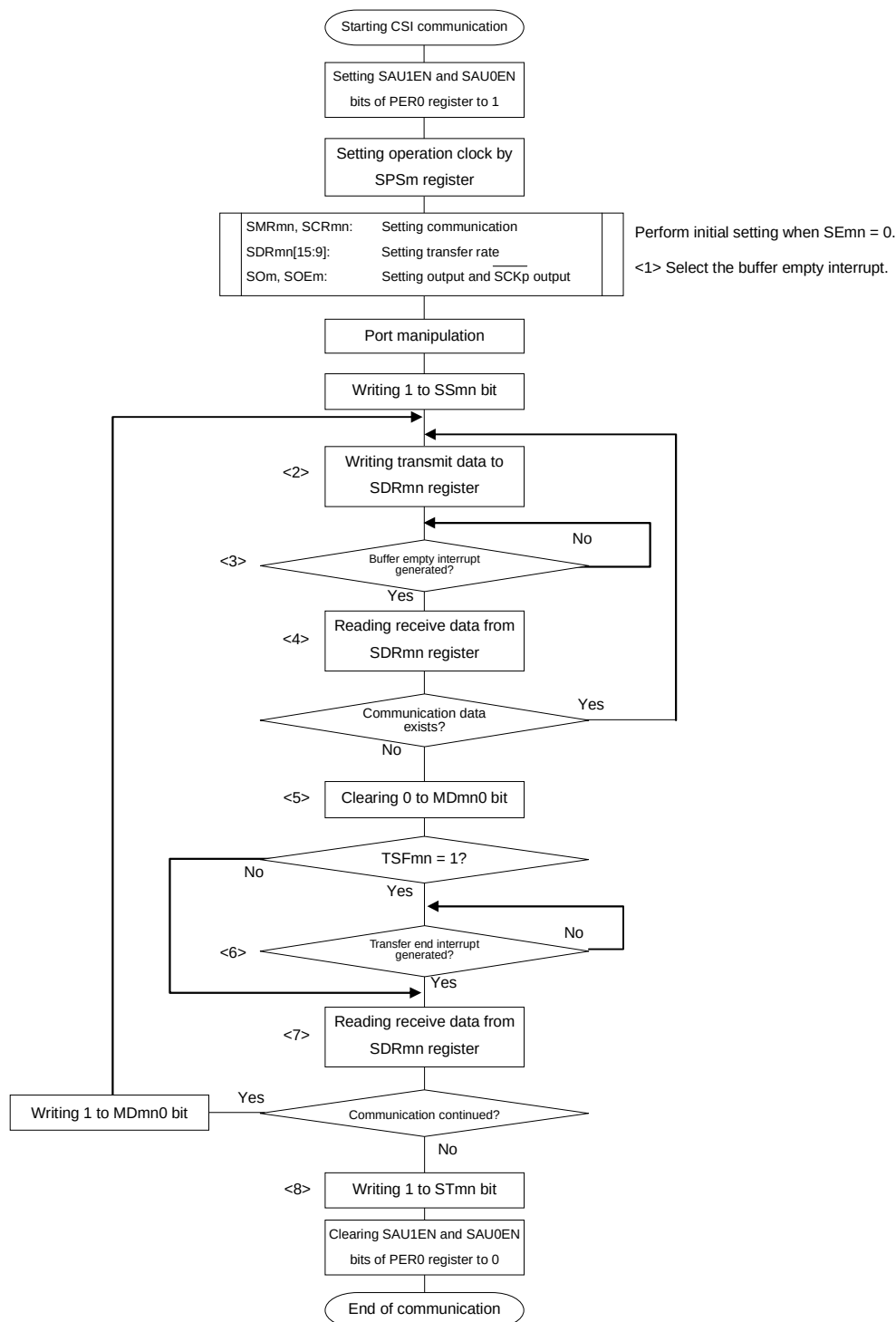
Figure 12-51. Flowchart of Master Transmission/Reception (in Continuous Transmission/Reception Mode)
