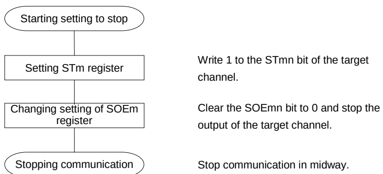
Figure 12-54. Procedure for Stopping Slave Transmission
