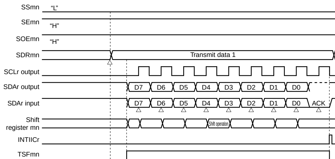
Figure 12-129. Timing Chart of Data Transmission
