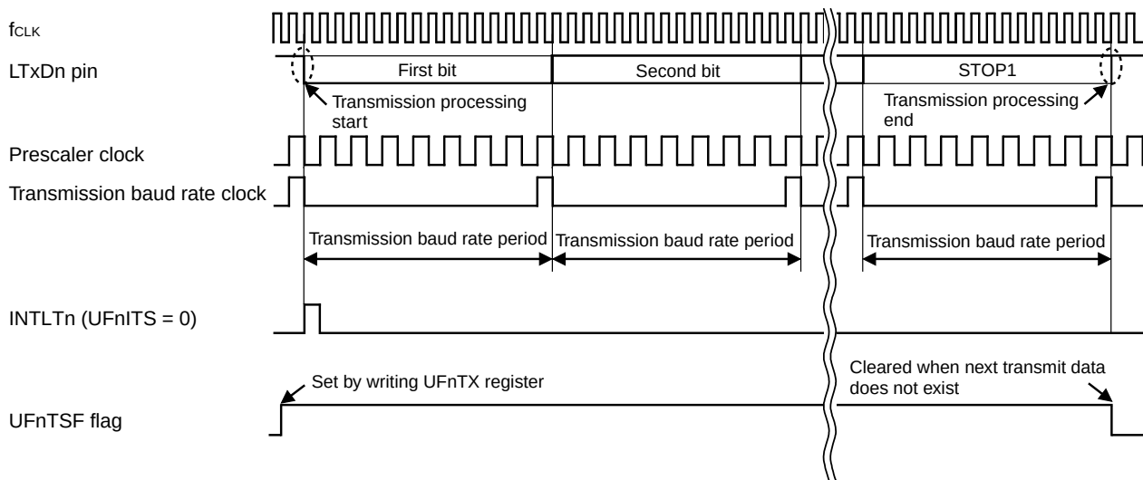
Figure 13-33. BF Transmission Timing Example
