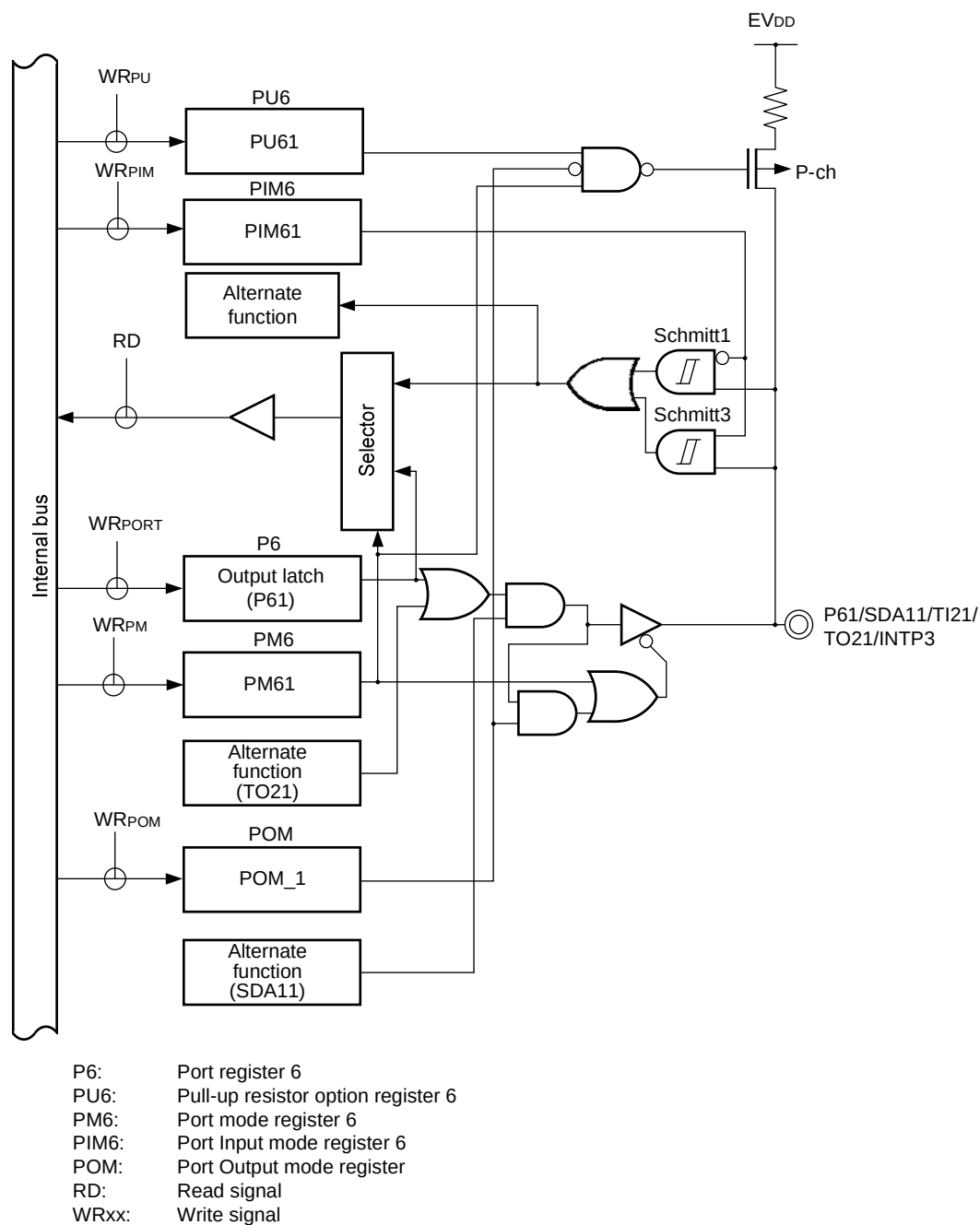
Figure 4-23. Block Diagram of P61
