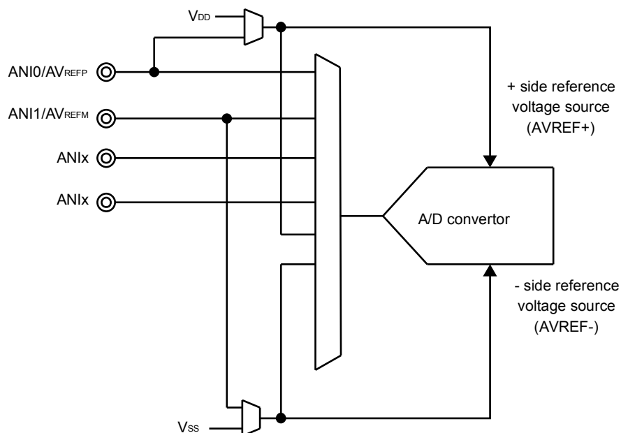
Figure 25-15. Configuration of A/D Test Function
