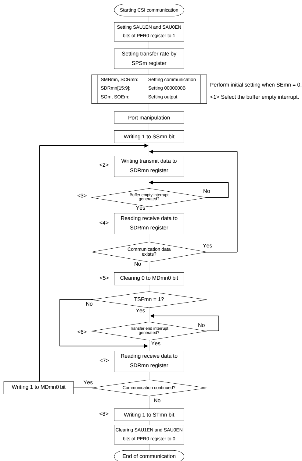
Figure 12-73. Flowchart of Slave Transmission/Reception (in Continuous Transmission/Reception Mode)
