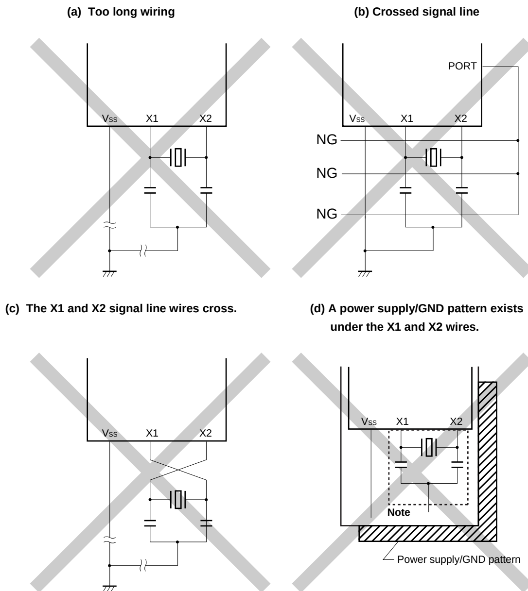
Figure 5-18. Examples of Incorrect Resonator Connection (1/2)
