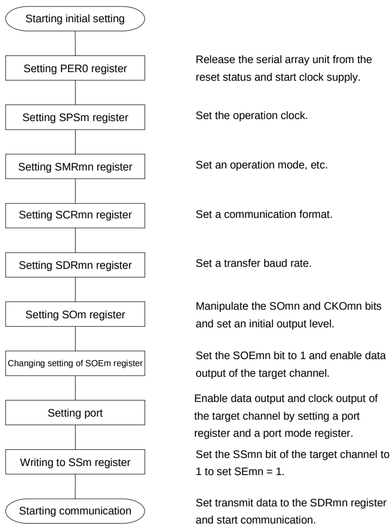
Figure 12-29. Initial Setting Procedure for Master Transmission
