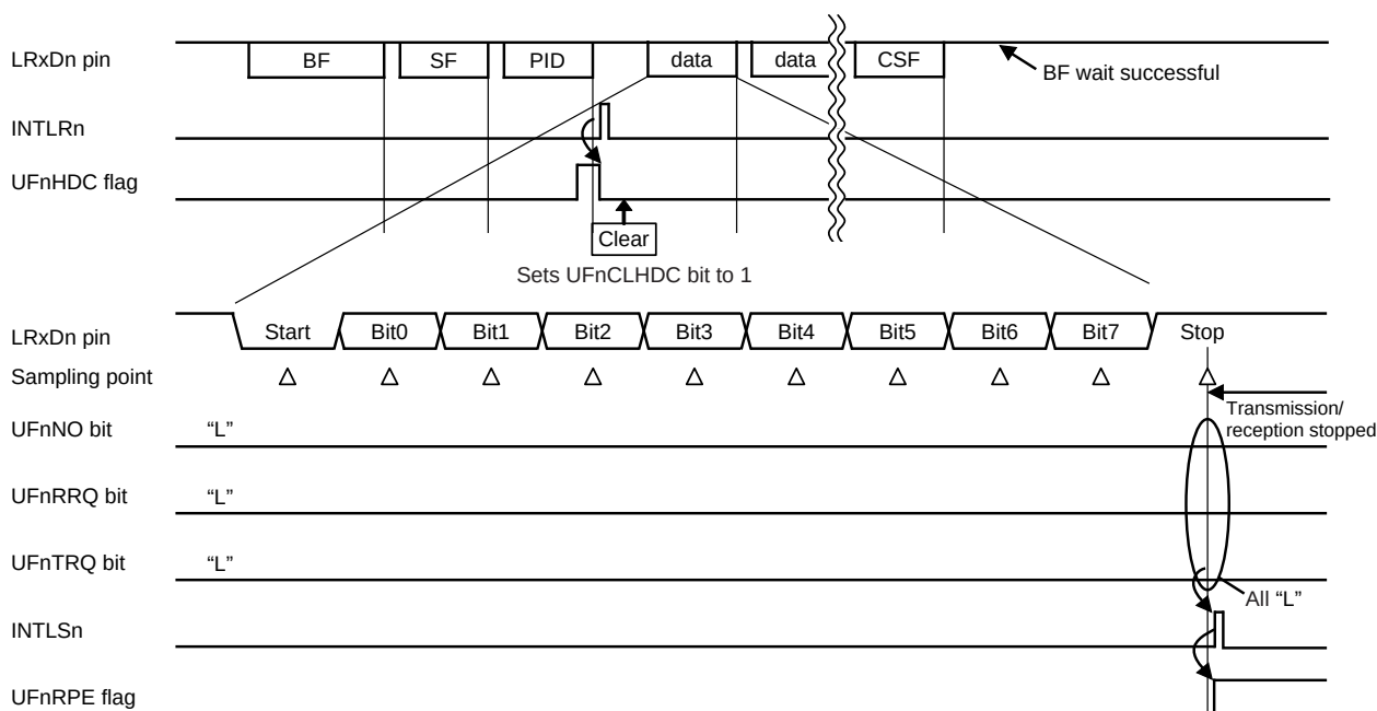
Figure 13-61. Response Preparation Error Occurrence Example
