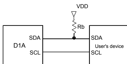
Figure 32-9 simplified IIC connection diagram
