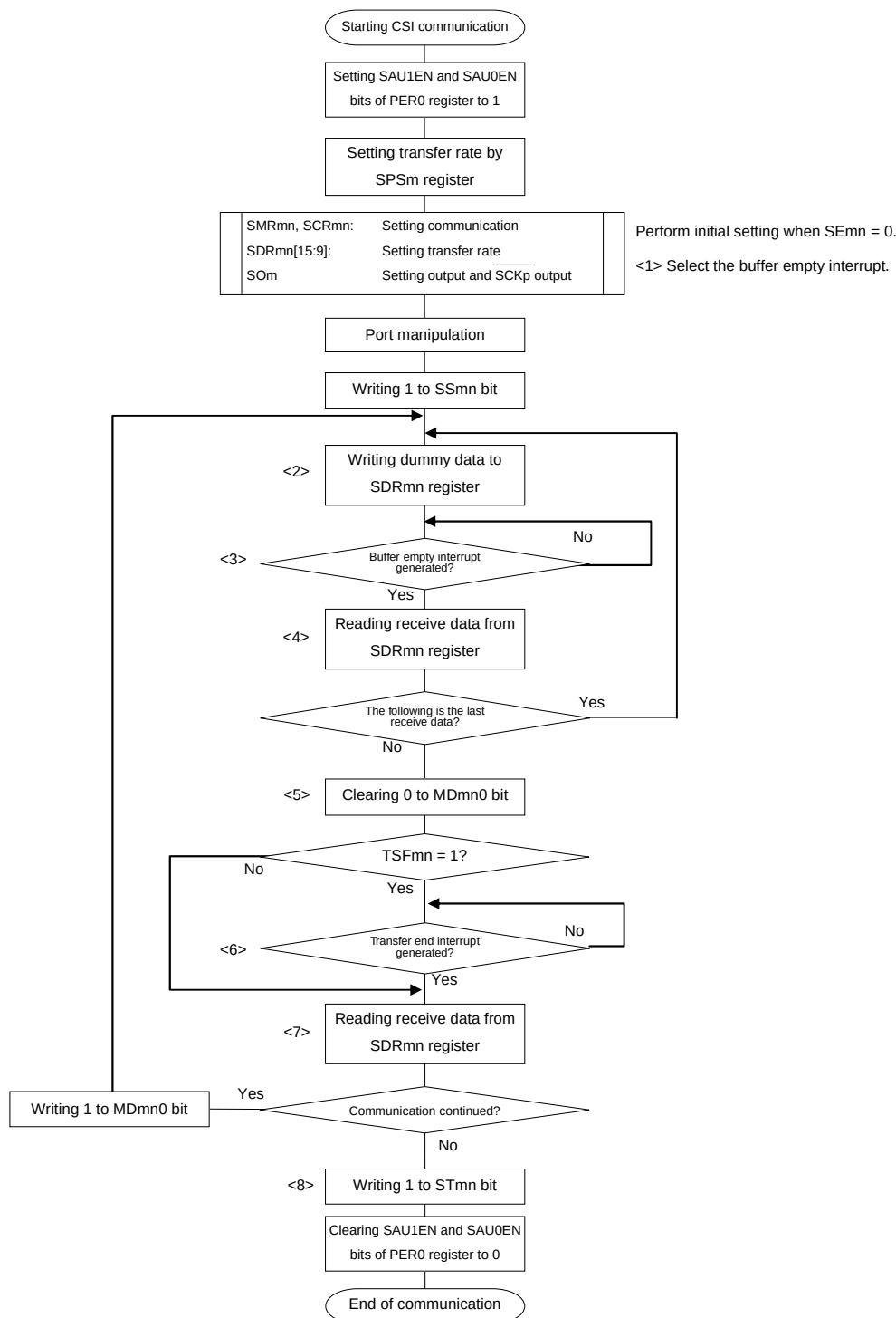
Figure 12-43. Flowchart of Master Reception (in Continuous Reception Mode)
