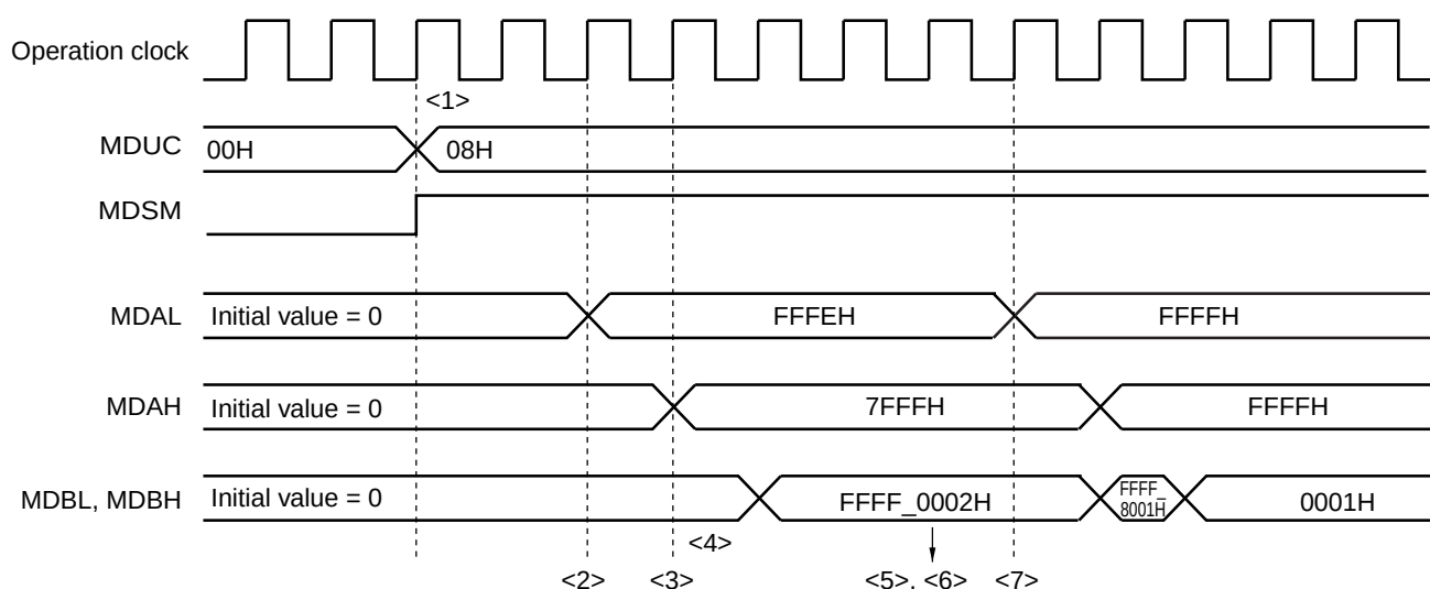
Figure 18-7. Timing Diagram of Multiplication (Signed) Operation ( -2 \times 32767 = -65534 )
