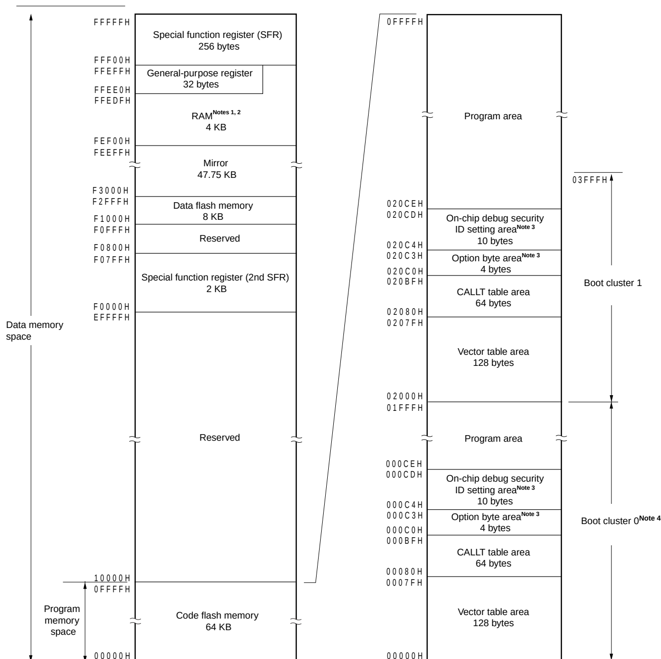
Figure 3-4. Memory Map (R5F10DGExFB, R5F10DLExFB, R5F10CMExFB, R5F10DMExFB, R5F10DPExFB)
