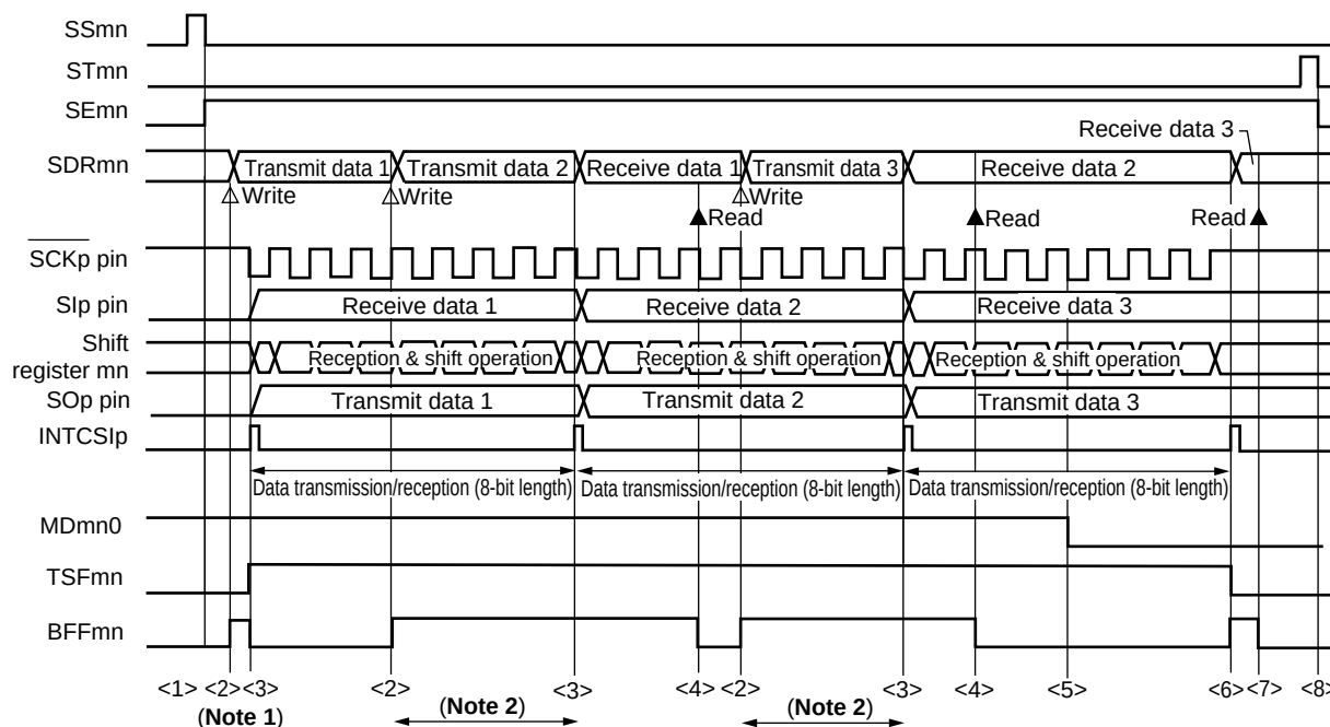
Figure 12-50. Timing Chart of Master Transmission/Reception (in Continuous Transmission/Reception Mode) (Type 1: DAPmn = 0, CKPmn = 0)
