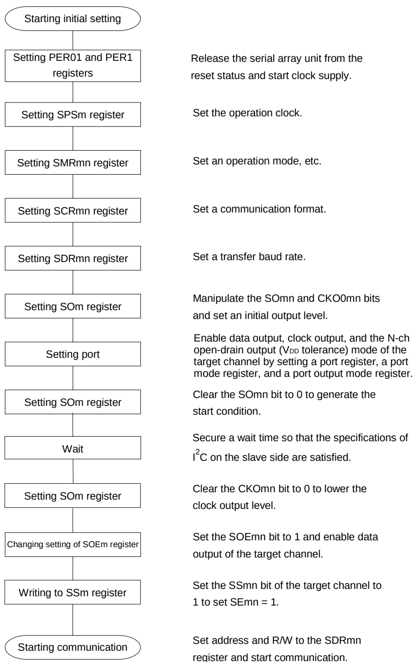
Figure 12-125. Initial Setting Procedure for Address Field Transmission
