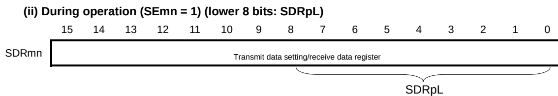
Figure 12-66. Example of Contents of Registers for Slave Transmission/Reception of 3-Wire Serial I/O (CSI00, CSI01, CSI10) (2/2)
