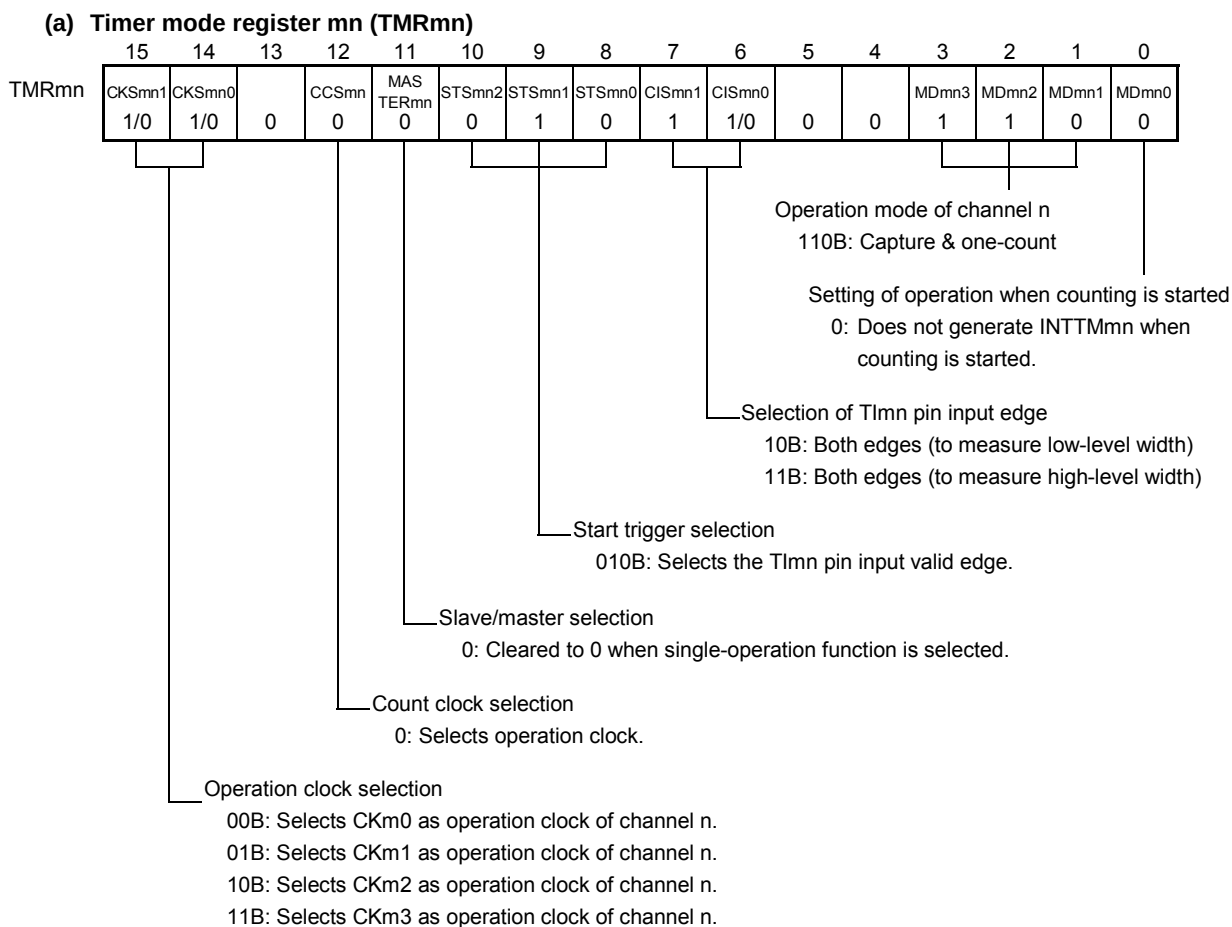
Figure 6-69. Example of Set Contents of Registers to Measure Input Signal High-/Low-Level Width (1/2)
