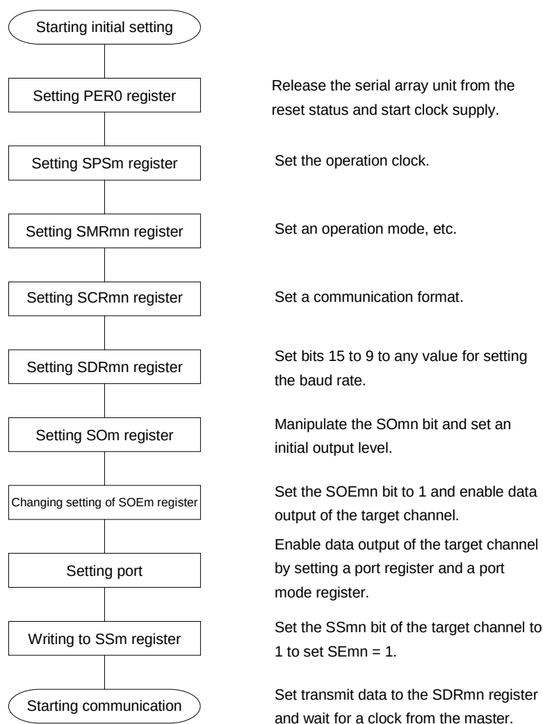
Figure 12-67. Initial Setting Procedure for Slave Transmission/Reception
