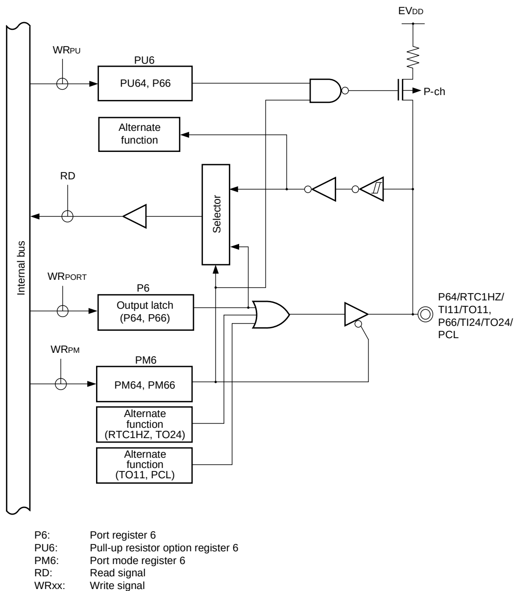
Figure 4-26. Block Diagram of P64, P66
