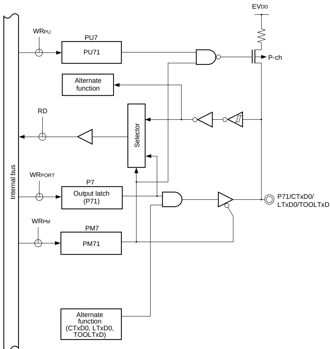
Figure 4-29. Block Diagram of P71
