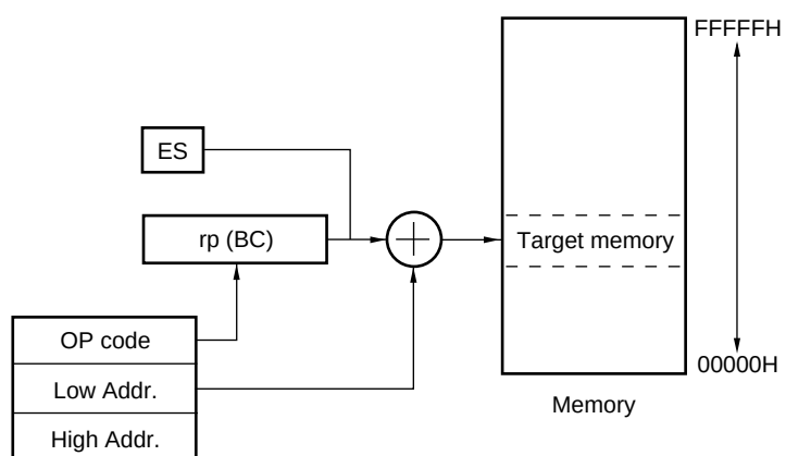
Figure 3-38. Example of ES:word[BC]
