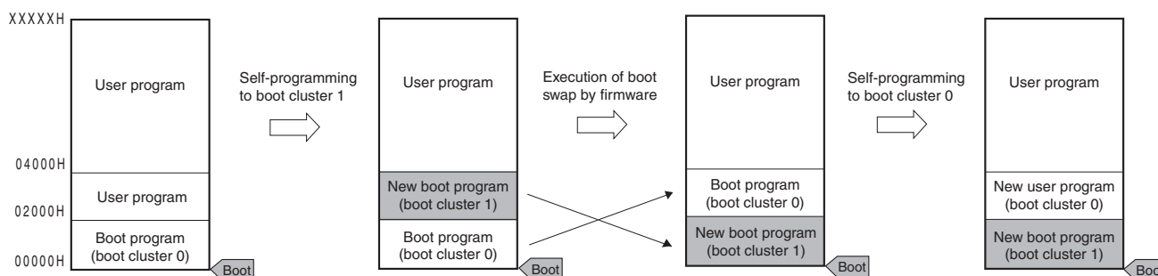
Figure 28-11. Boot Swap Function
