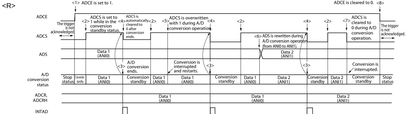
Figure 11-19. Example of Software Trigger Mode (Select Mode, One-Shot Conversion Mode) Operation Timing
