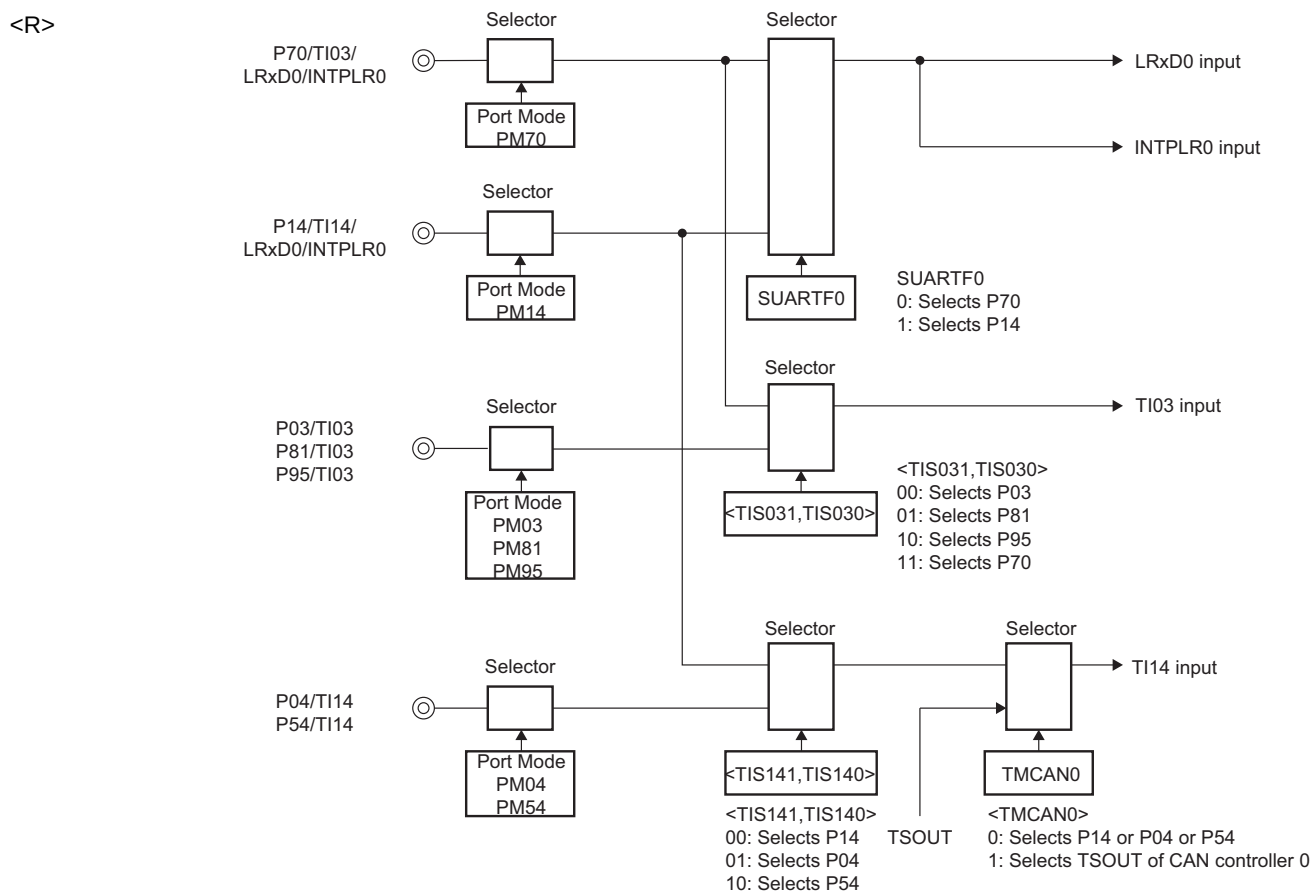
Figure 13-30. Port Configuration of LIN Reception Manipulation
