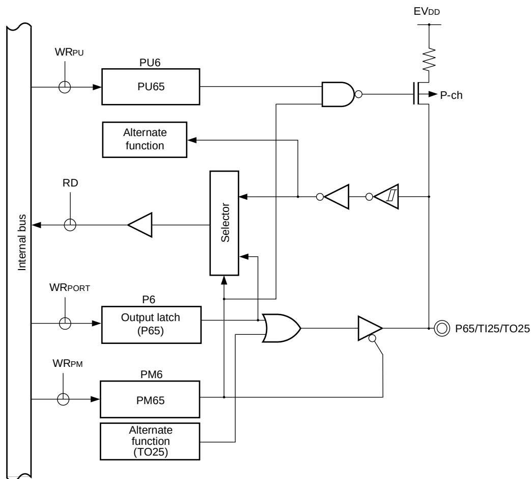
Figure 4-27. Block Diagram of P65
