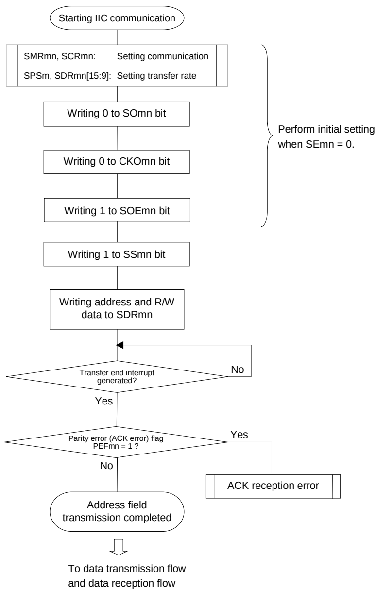
Figure 12-127. Flowchart of Address Field Transmission
