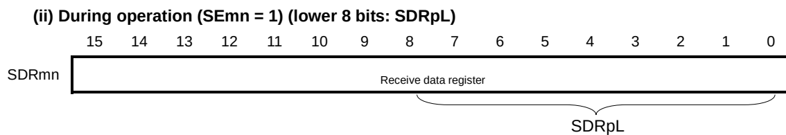
Figure 12-60. Example of Contents of Registers for Slave Reception of 3-Wire Serial I/O (CSI00, CSI01, CSI10) (2/2)
