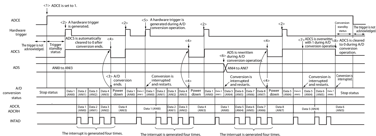
Figure 11-29. Example of Hardware Trigger Wait Mode (Scan Mode, One-Shot Conversion Mode) Operation
