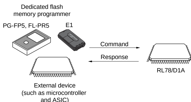
Figure 28-9. Communication Commands
