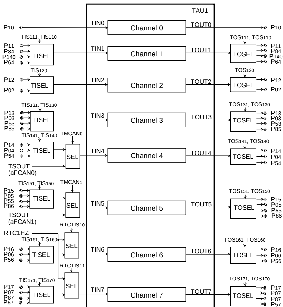
Figure 4-59. Timer Array unit and RTC I/O connection (2/3)
