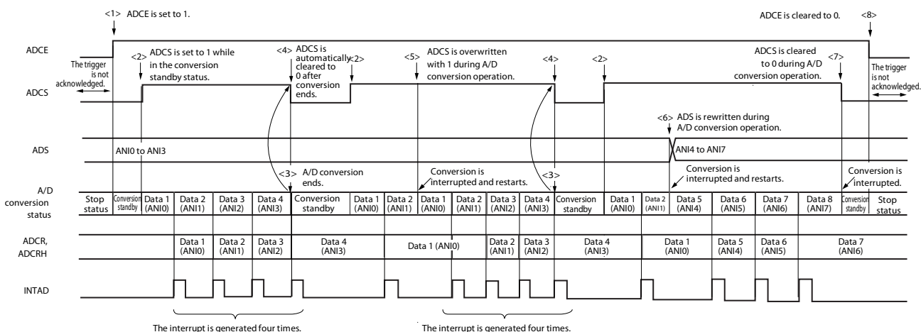
Figure 11-21. Example of Software Trigger Mode (Scan Mode, One-Shot Conversion Mode) Operation Timing
