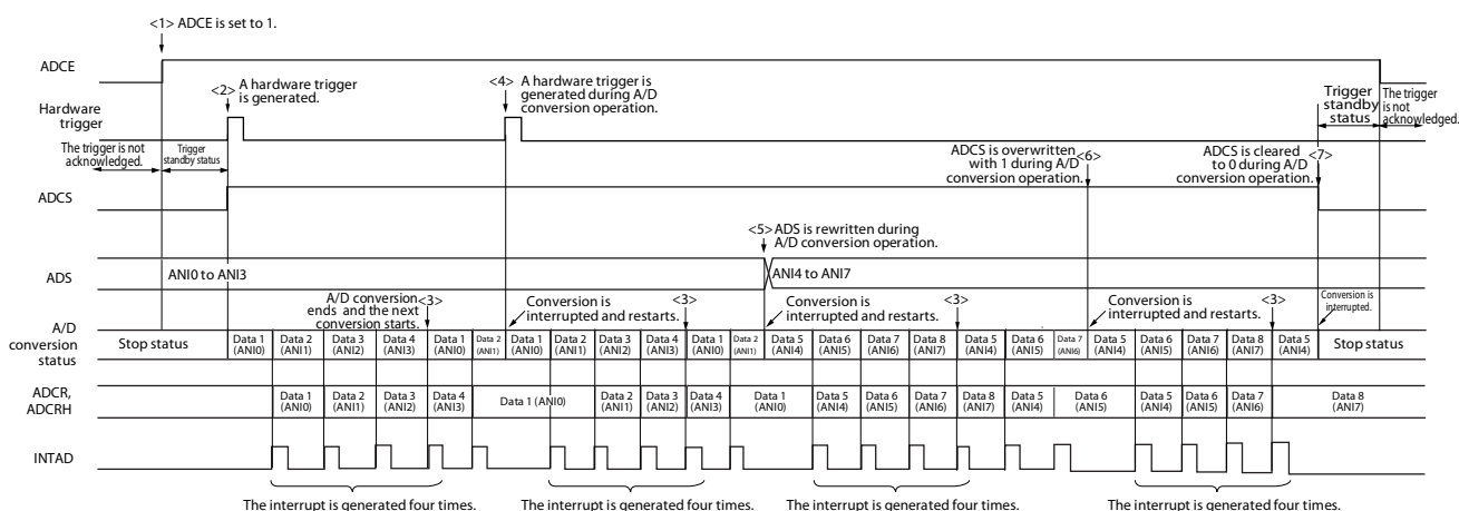
Figure 11-28. Example of Hardware Trigger Wait Mode (Scan Mode, Sequential Conversion Mode) Operation Timing
