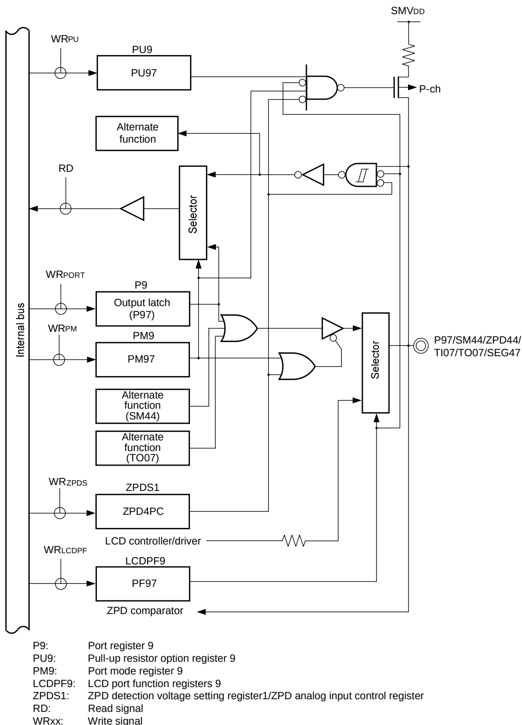
Figure 4-38. Block Diagram of P97
