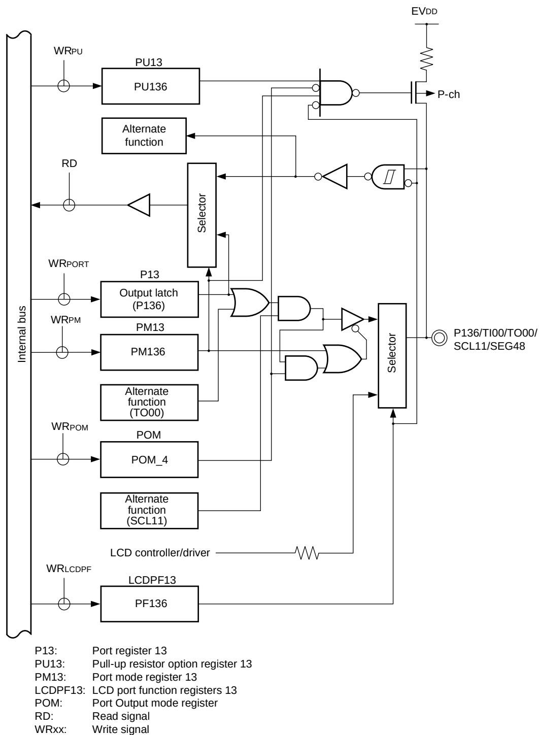
Figure 4-47. Block Diagram of P136
