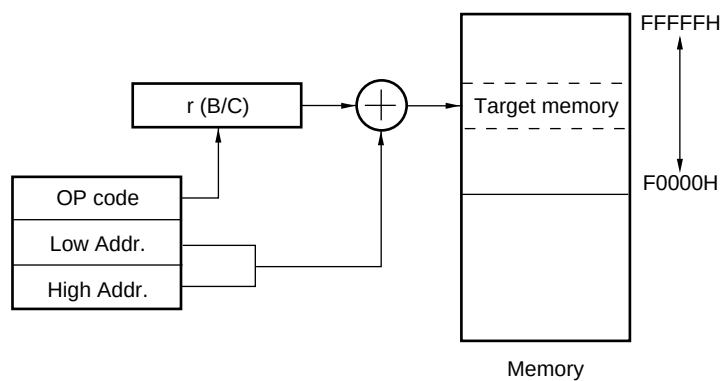
Figure 3-34. Example of word[B], word[C]
