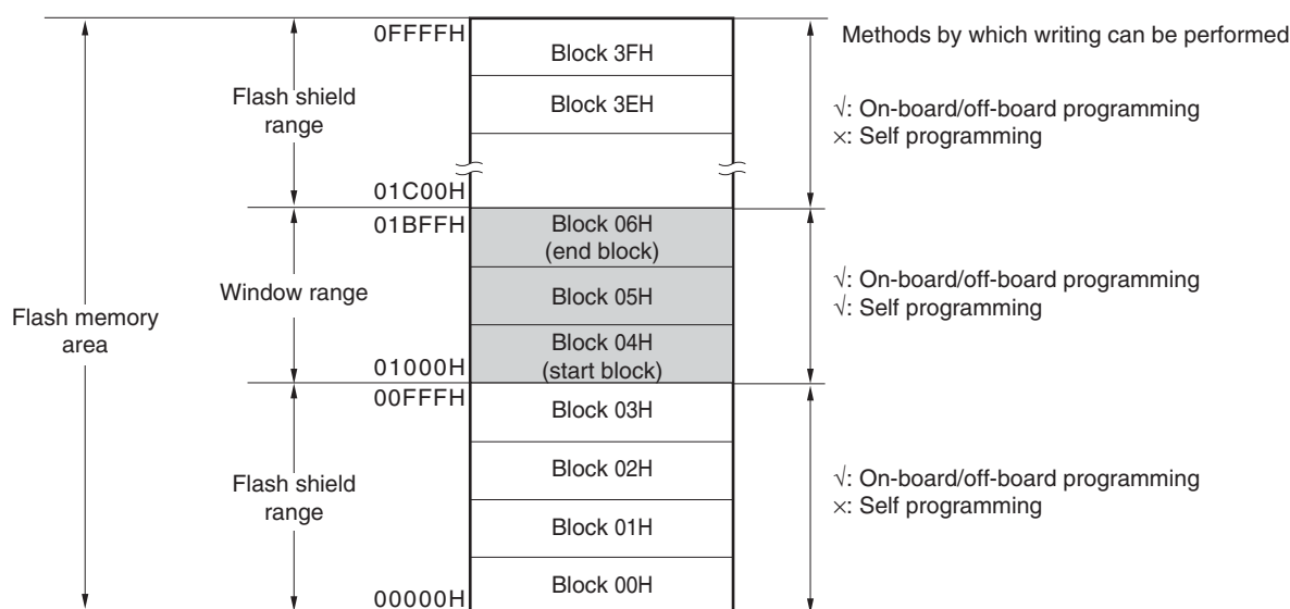
Figure 28-13. Flash Shield Window Setting Example (Start Block: 04H, End Block: 06H)
