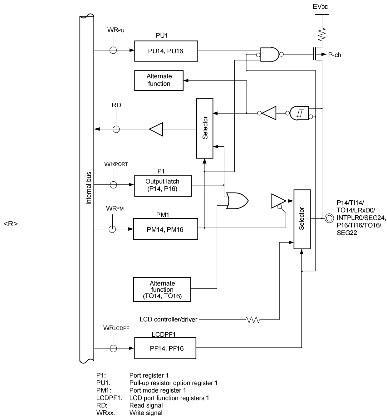
Figure 4-10. Block Diagram of P14, P16
