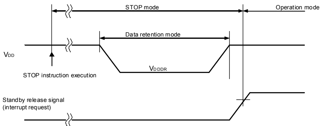
Figure 32-13. STOP Mode Data Retention timing
