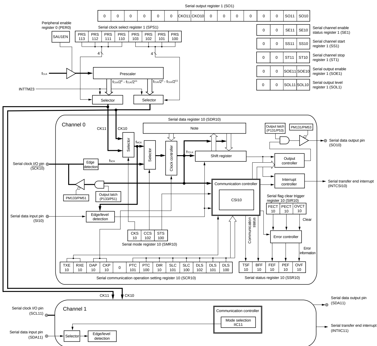
Figure 12-3. Block Diagram of Serial Array Unit 1
