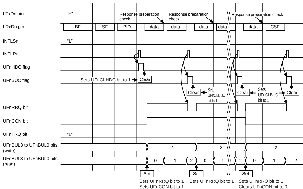
Figure 13-65. Multi-Byte Reception Implementation Example
