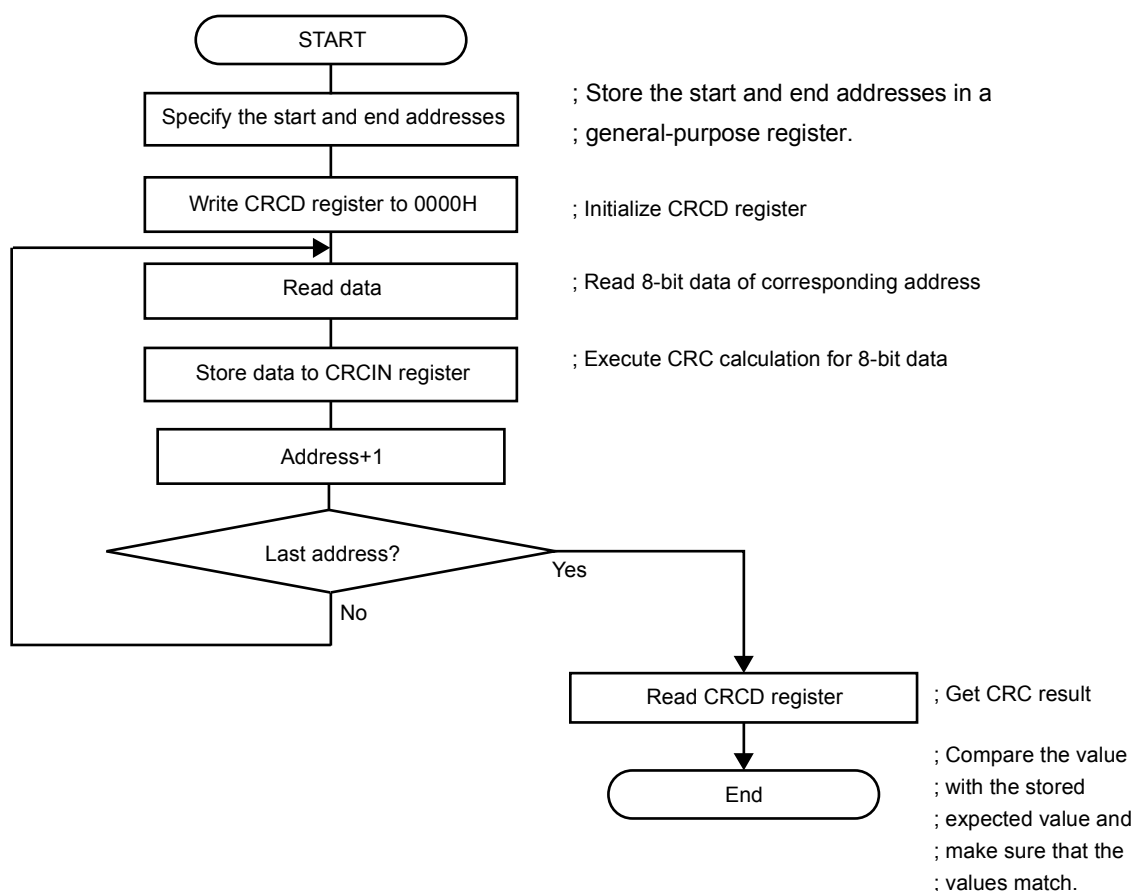
Figure 25-6. CRC Operation Function (General-Purpose CRC)
