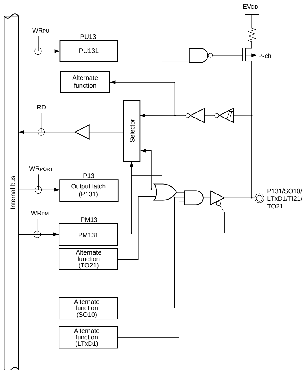
Figure 4-42. Block Diagram of P131
