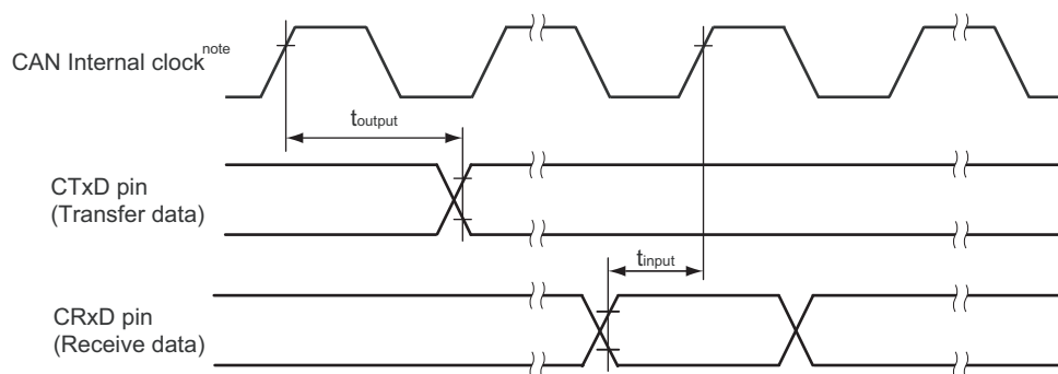
Figure 33-11. Internal delay time of CAN
