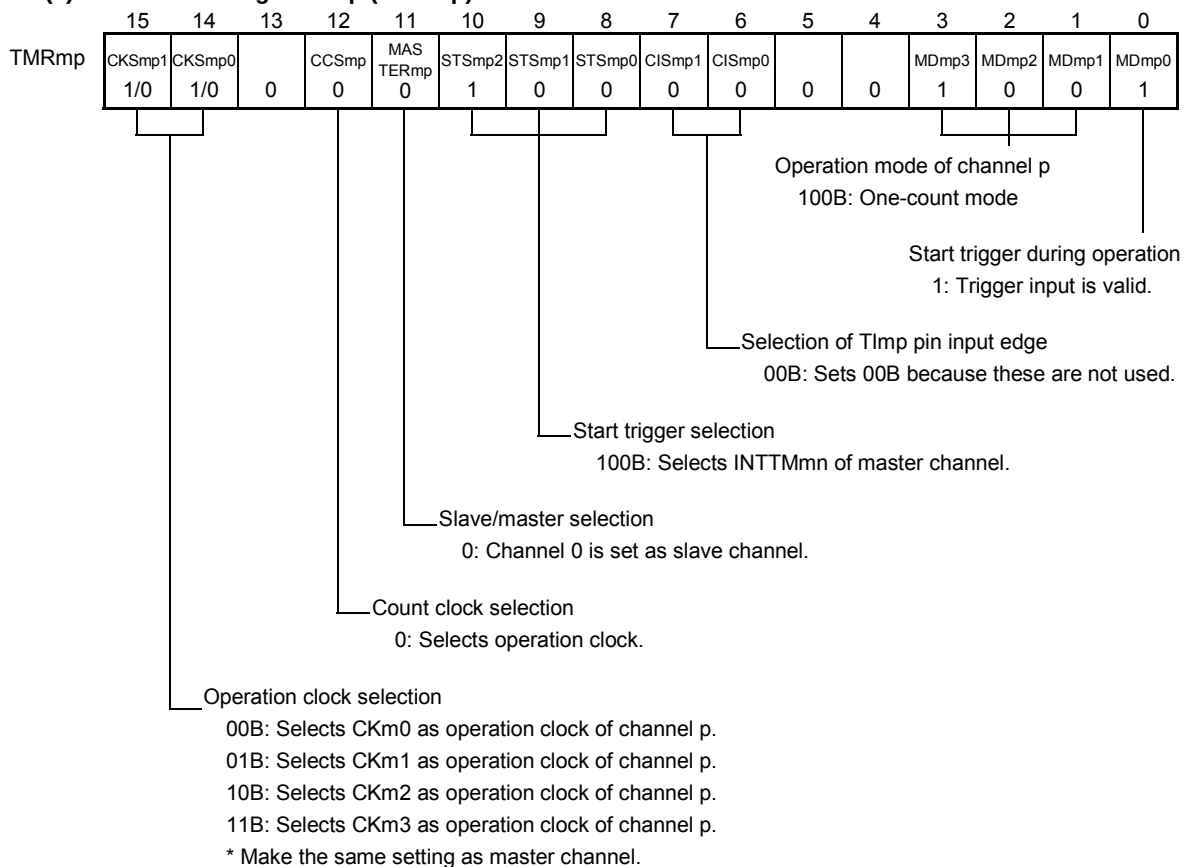
Figure 6-74. Example of Set Contents of Registers When PWM Function (Slave Channel) Is Used (1/2)
