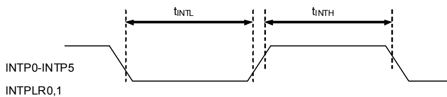
Figure 32-4. Interrupt Request Input Timing
