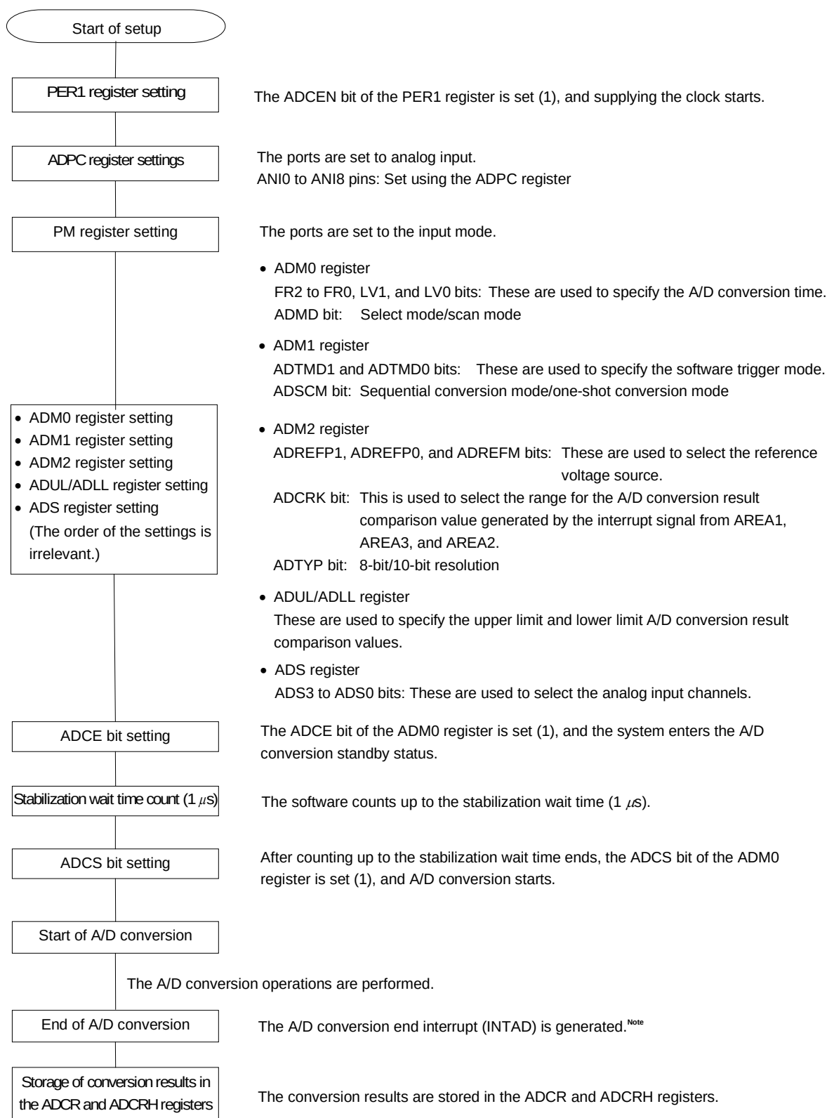
Figure 11-30. Setting up Software Trigger Mode
