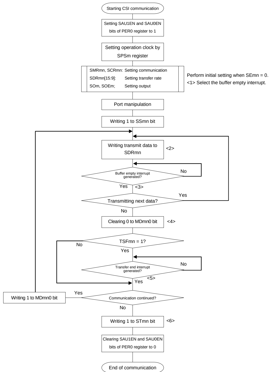
Figure 12-35. Flowchart of Master Transmission (in Continuous Transmission Mode)
