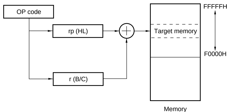
Figure 3-39. Example of [HL+B], [HL+C]
