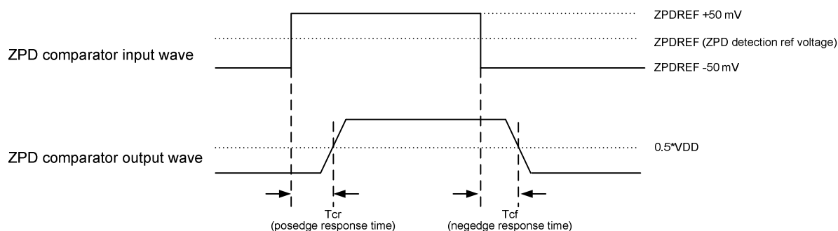
Figure 33-12. ZPD timing
