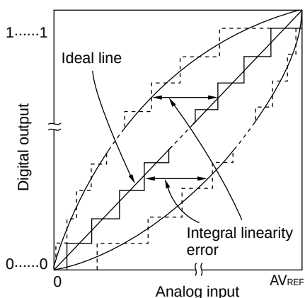
Figure 11-41. Integral Linearity Error
