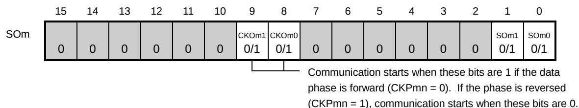
Figure 12-28. Example of Contents of Registers for Master Transmission of 3-Wire Serial I/O (CSI00, CSI01, CSI10) (1/2)
