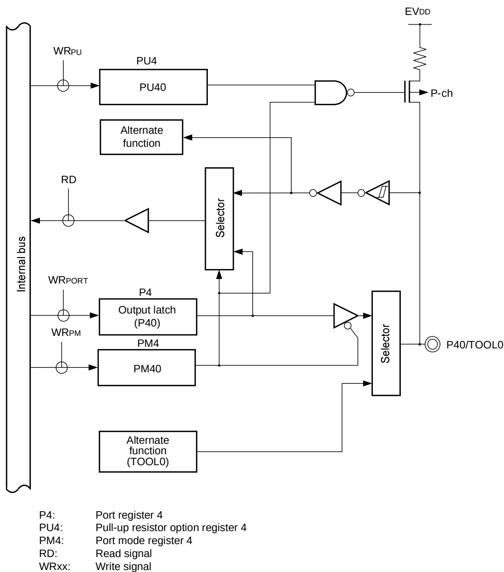
Figure 4-17. Block Diagram of P40
