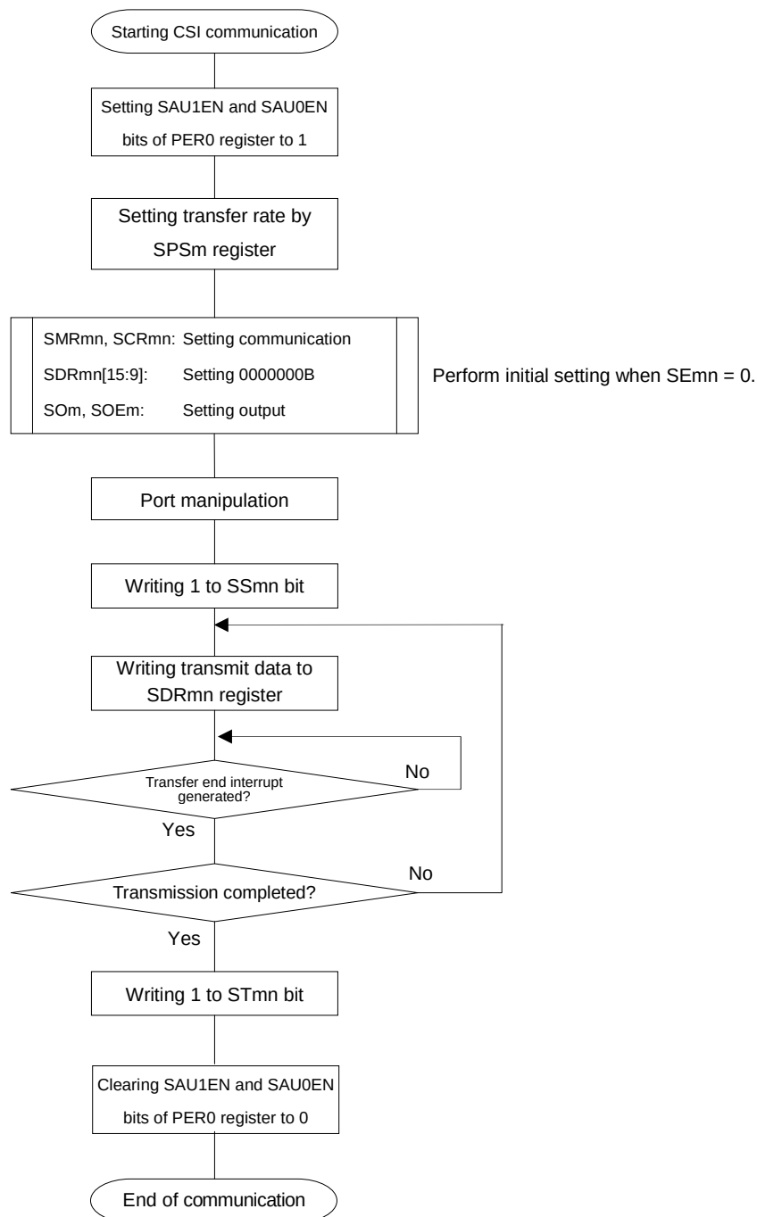
Figure 12-57. Flowchart of Slave Transmission (in Single-Transmission Mode)
