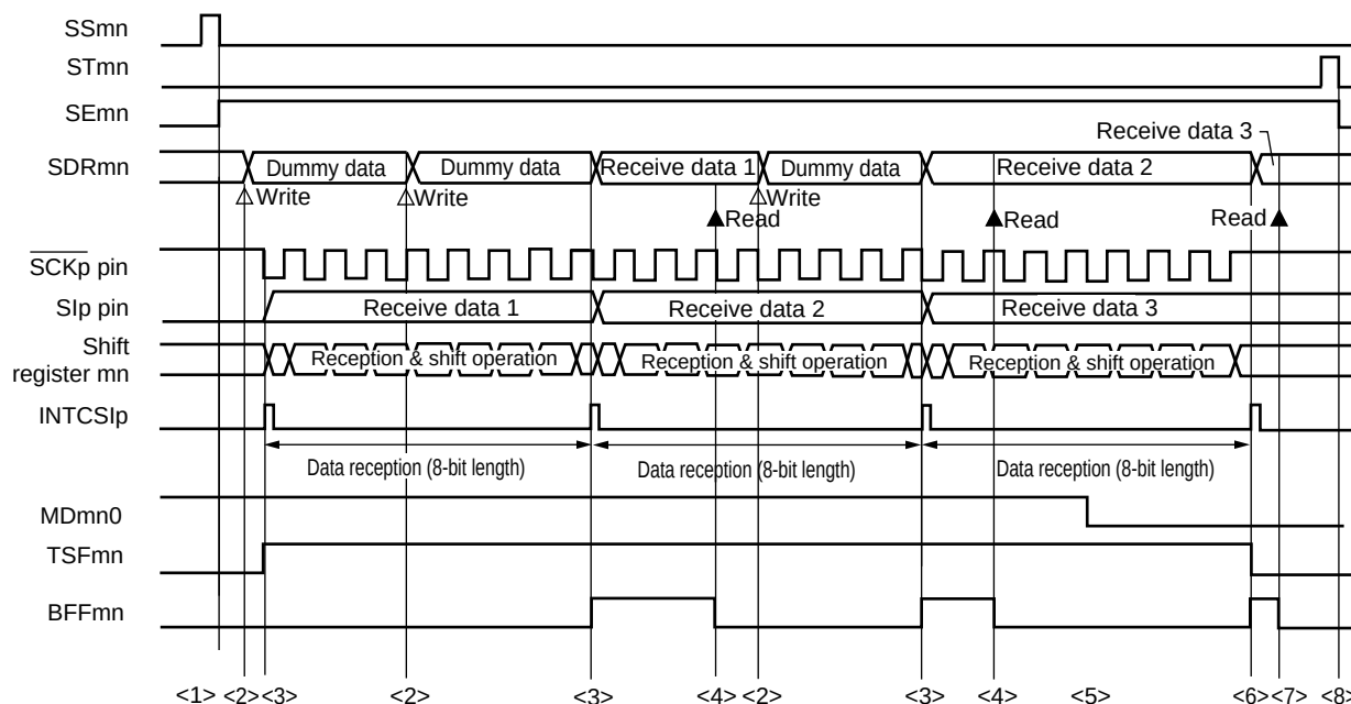
Figure 12-42. Timing Chart of Master Reception (in Continuous Reception Mode)
