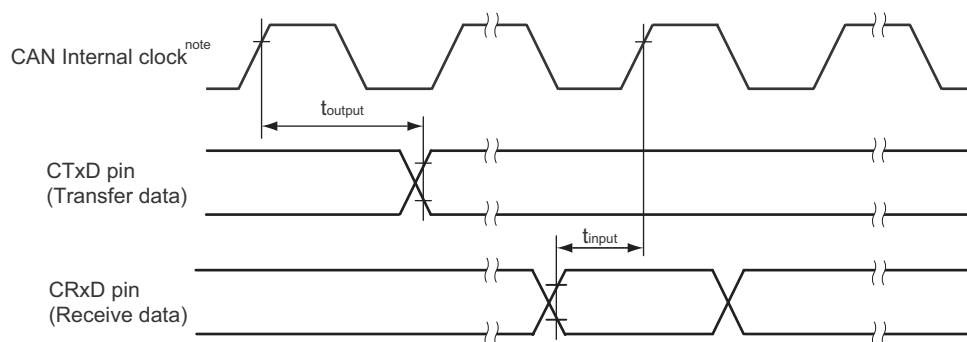
Figure 32-11. Internal delay time of CAN
