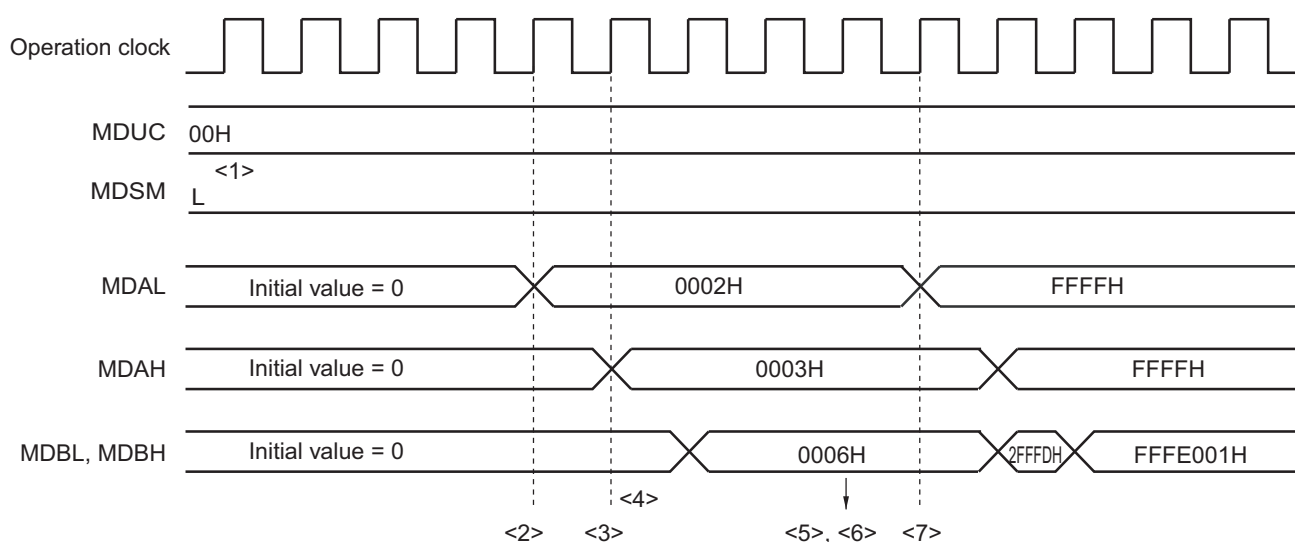
Figure 18-6. Timing Diagram of Multiplication (Unsigned) Operation ( 2 \times 3 = 6 )
