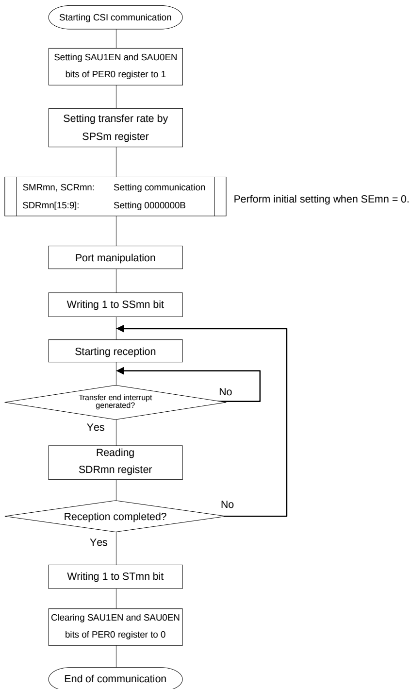
Figure 12-65. Flowchart of Slave Reception (in Single-Reception Mode)
