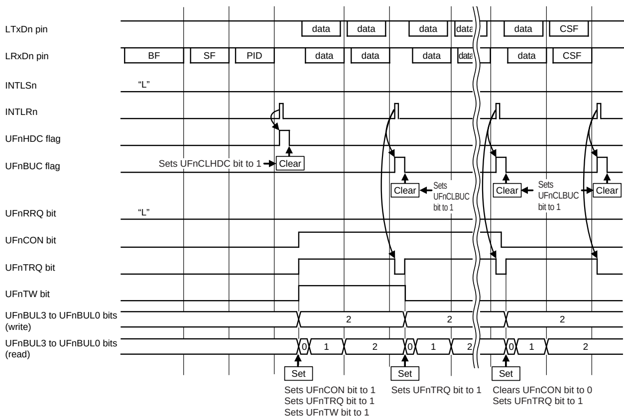
Figure 13-66. Multi-Byte Transmission Implementation Example
