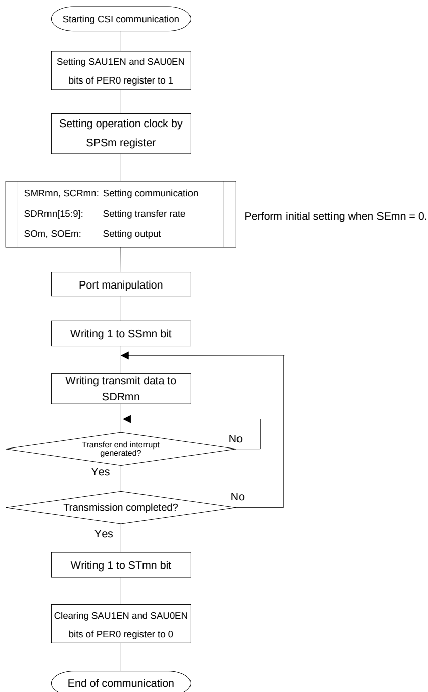
Figure 12-33. Flowchart of Master Transmission (in Single-Transmission Mode)
