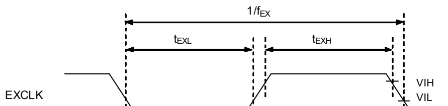
Figure 32-2. External Main System Clock Timing
